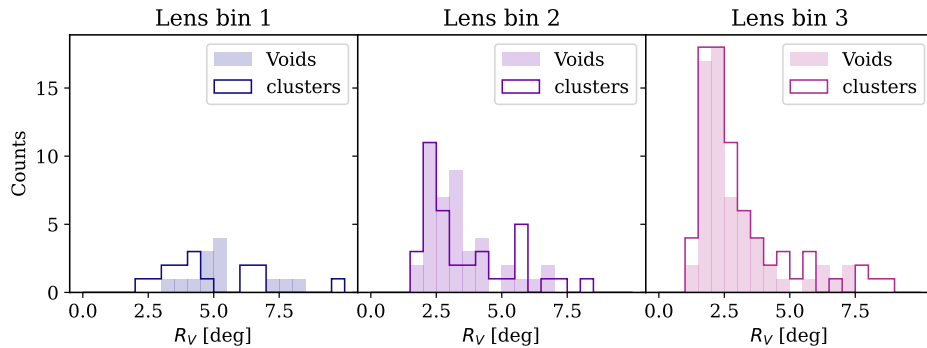
Figure F1. Distribution of the radii, R_V , for the identified voids (shaded region) and clusters (solid lines) in lens bin 1 - 3 for the DES Y3 RedMaGiC galaxies.
