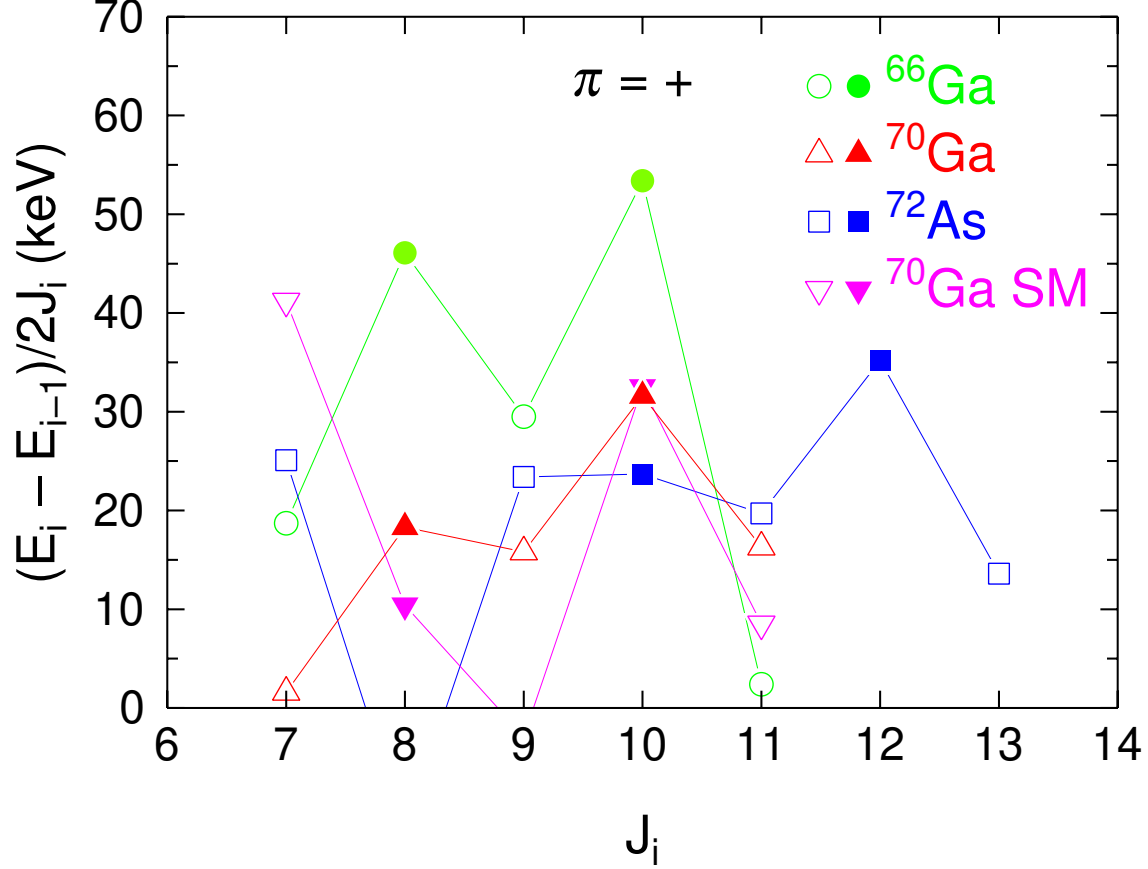
FIG. 7: Normalized energy differences between adjacent states as a function of the spin J_i of the initial state for the yrast positive-parity decay sequences in ^{66}\text{Ga} [1], ^{70}\text{Ga} , and ^{72}\text{As} [39, 40]. Theoretical values predicted by shell-model (SM) calculations for the yrast positive-parity sequence in ^{70}\text{Ga} are also included. Filled (open) symbols are used for states with even (odd) J_i .
