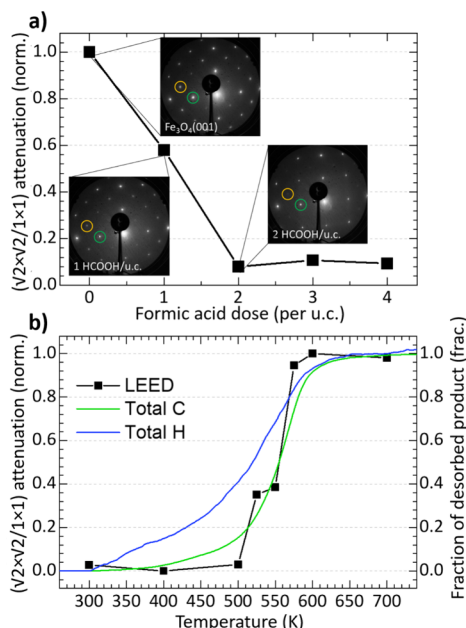
Figure 3. Normalized ratio of (\sqrt{2} \times \sqrt{2}) and (1 \times 1) \text{Fe}_3\text{O}_4(001) LEED spot intensities (black squares) as a function of (a) HCOOH dose at 300 K and (b) annealing temperature for saturation dose of 2 HCOOH/u.c. All data was acquired at 300 K with a beam energy of 66.7 eV, and each image was taken at a different sample location to minimize beam damage. The sample was annealed at the same rate as the TPRS (1 K/s). The yellow and green circles in the LEED images of (a) represent the (\sqrt{2} \times \sqrt{2}) and (1 \times 1) LEED spots, respectively. Additional LEED images are displayed in Figures S4 and S5. Green and blue lines in panel b are the fractional TPRS product yields of carbon and hydrogen-containing products from 2 HCOOH/u.c. presented in Figure 4.
