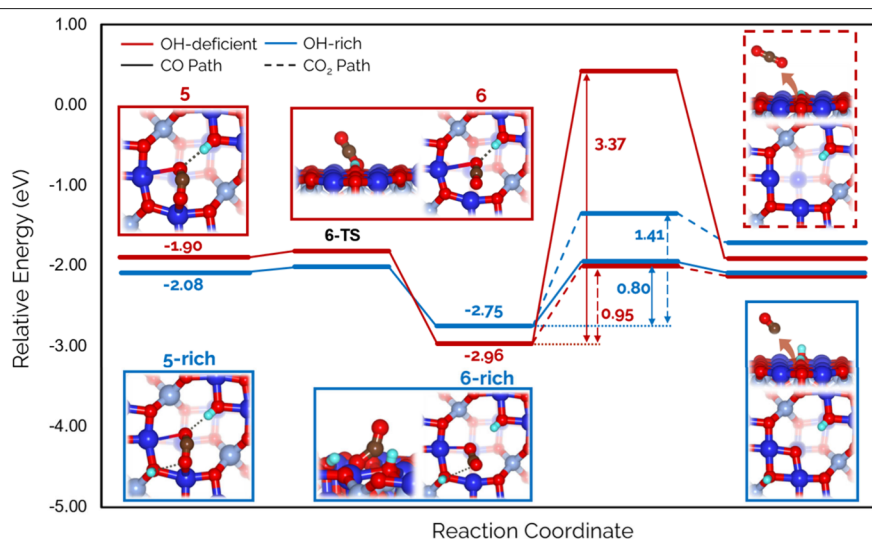
Figure 8. Comparison of different pathways to OCO configurations (steps 5 and 6 in Figure 7) on the (\sqrt{2} \times \sqrt{2})\text{R}45^\circ reconstructed \text{Fe}_3\text{O}_4 (001) surface. The energies are referenced to a clean surface with three noninteracting gaseous formic acid molecules. The differences in the final states are due to the differences in energy of the OH-deficient and OH-rich surfaces. The \text{Fe}_{\text{occ}} , \text{Fe}_{\text{ter}} , C, O, and H atoms are represented as blue, light blue-gray, brown, red, and teal spheres, respectively, and energies are references to the final state of step 5 (embedded OCO). From step 6 on both surfaces, the CO production pathway energetics are denoted with a solid line, and the \text{CO}_2 production pathway energetics are denoted with a dashed line.
