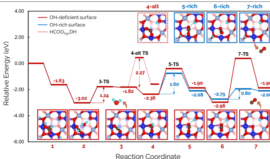
Figure 7. Energy diagram of HCOOH decomposition to CO on hydroxyl-deficient (red) and hydroxyl-rich (blue) (\sqrt{2} \times \sqrt{2})\text{R}45^\circ reconstructed \text{Fe}_3\text{O}_4 (001). All energies are corrected with ZPE and referenced to a clean reconstructed \text{Fe}_3\text{O}_4 (001) surface and three noninteracting gas-phase formic acid molecules. Inserts of the minima configurations for the hydroxyl-deficient paths are framed in red, and the hydroxyl-rich surface is shown in blue (labeled as 5, 6, 7-rich). A dotted red line shows a direct C–H bond cleavage of the bidentate formate step (4-alt). The \text{Fe}_{\text{oct}} , \text{Fe}_{\text{tet}} , C, O, and H atoms are represented as blue, light blue-gray, brown, red, and teal spheres. The hydroxyl-deficient/rich surfaces refer to the location of the OH relative to the BLO and the number of H is consistent for the different calculations. Additional molecular figures highlighting the oxygens from the reactant are included in the SI (Figure S15).
