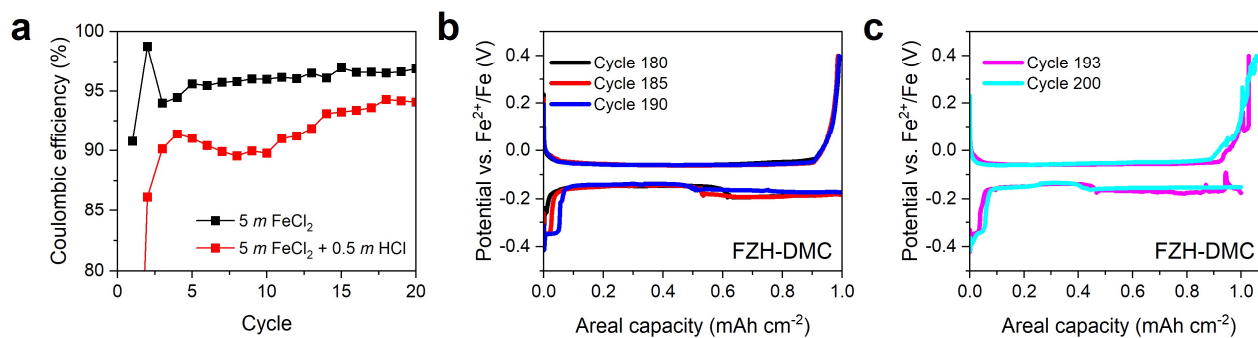
Supporting Figure S8. Additional GCD profiles and CE data related to FZH-DMC. (a) CE of the cells undergo 10 precycles with FZH-DMC, and the electrolyte is rinsed and refilled. (b) GCD profiles of FZH-DMC cell in later cycles. (c) GCD profiles of FZH-DMC cell after cell failure, showing stripping capacity larger than plating capacity.
