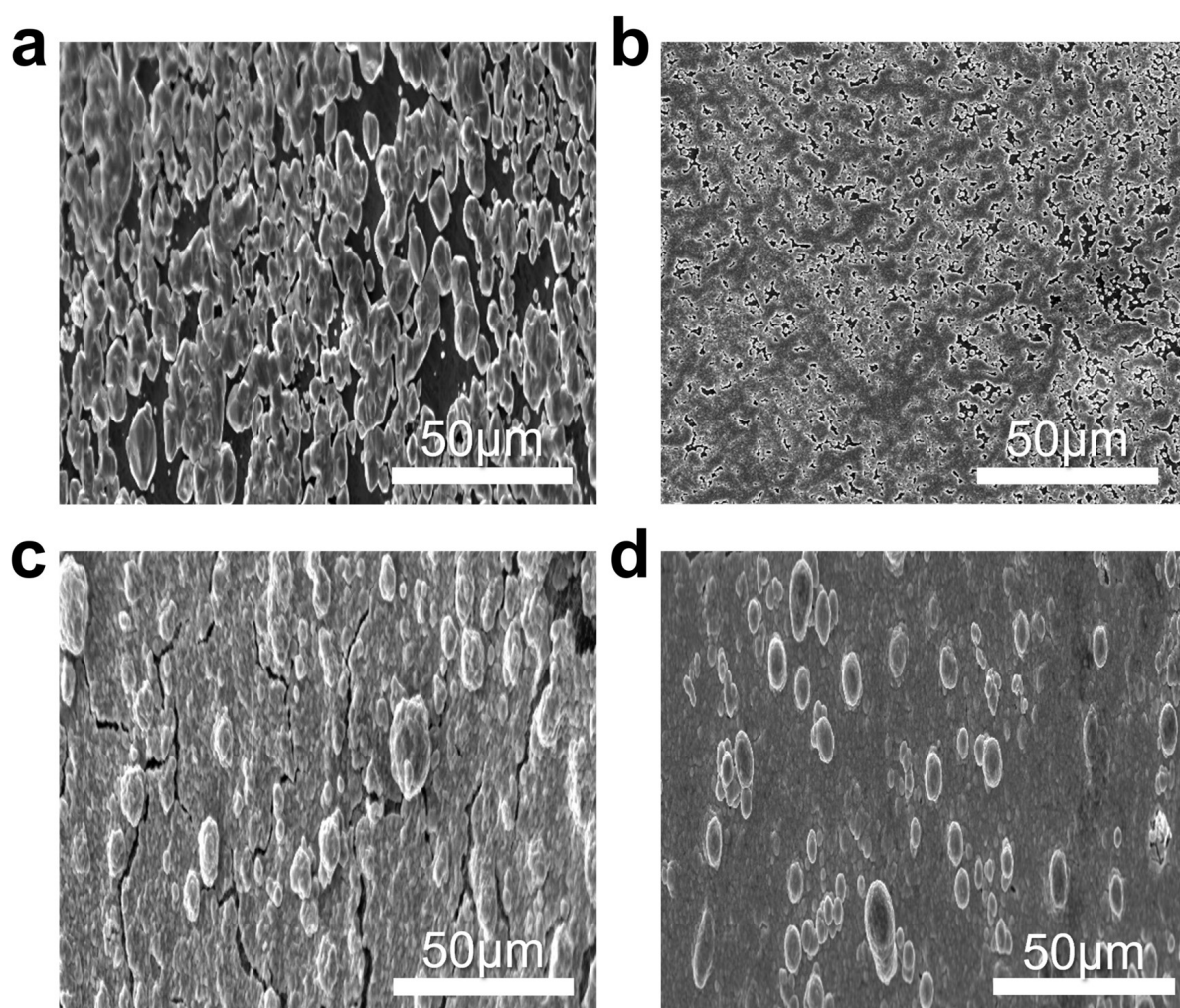
Supporting Figure S11. SEM images of the cycled working electrode surfaces after 10 th plating, using (a) 5 m FeCl 2 , (b) 5 m FeCl 2 + 0.5 m HCl, (c) FZH, and (d) FZH-DMC as the electrolytes.
