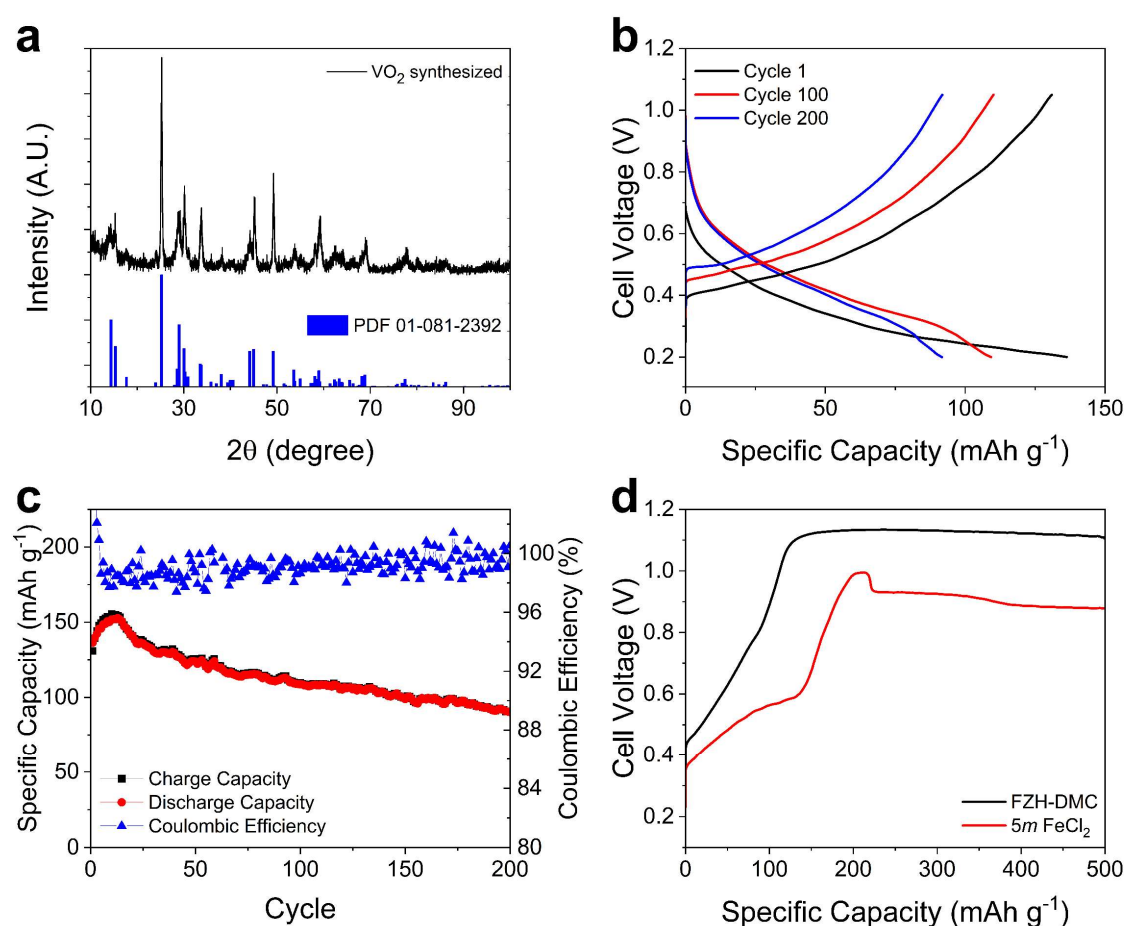
Figure 8. Electrochemical data of FeIBs utilizing VO 2 as a model cathode. (a) XRD pattern of VO 2 synthesized and the corresponding ICDD card PDF#01-081-2392. (b) Representative GCD profiles of the VO 2 ||Fe cell and (c) its cycling performance. (d) Unlimited galvanostatic charging profiles of VO 2 ||Fe cells using different electrolytes.
