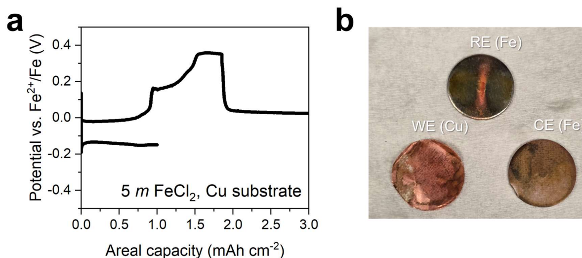
Supporting Figure S1. Impact of the Cu current collector material on the CE measurements. (a) GCD profiles of the Fe anode using Cu foil as a working electrode current collector. (b) Digital images of electrodes taken out from the Swagelok cell after observing “endless” charging of the cell.
