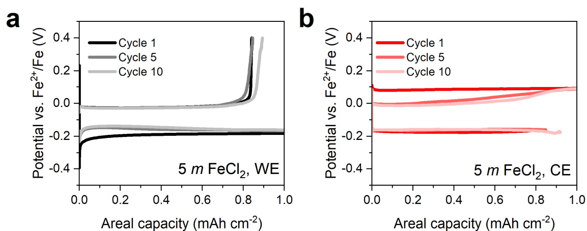
Supporting Figure S3. GCD profiles of the (a) working electrode (WE) and (b) counter electrode (CE) of the three-electrode Ti||Fe cell using another Fe foil as a reference.
