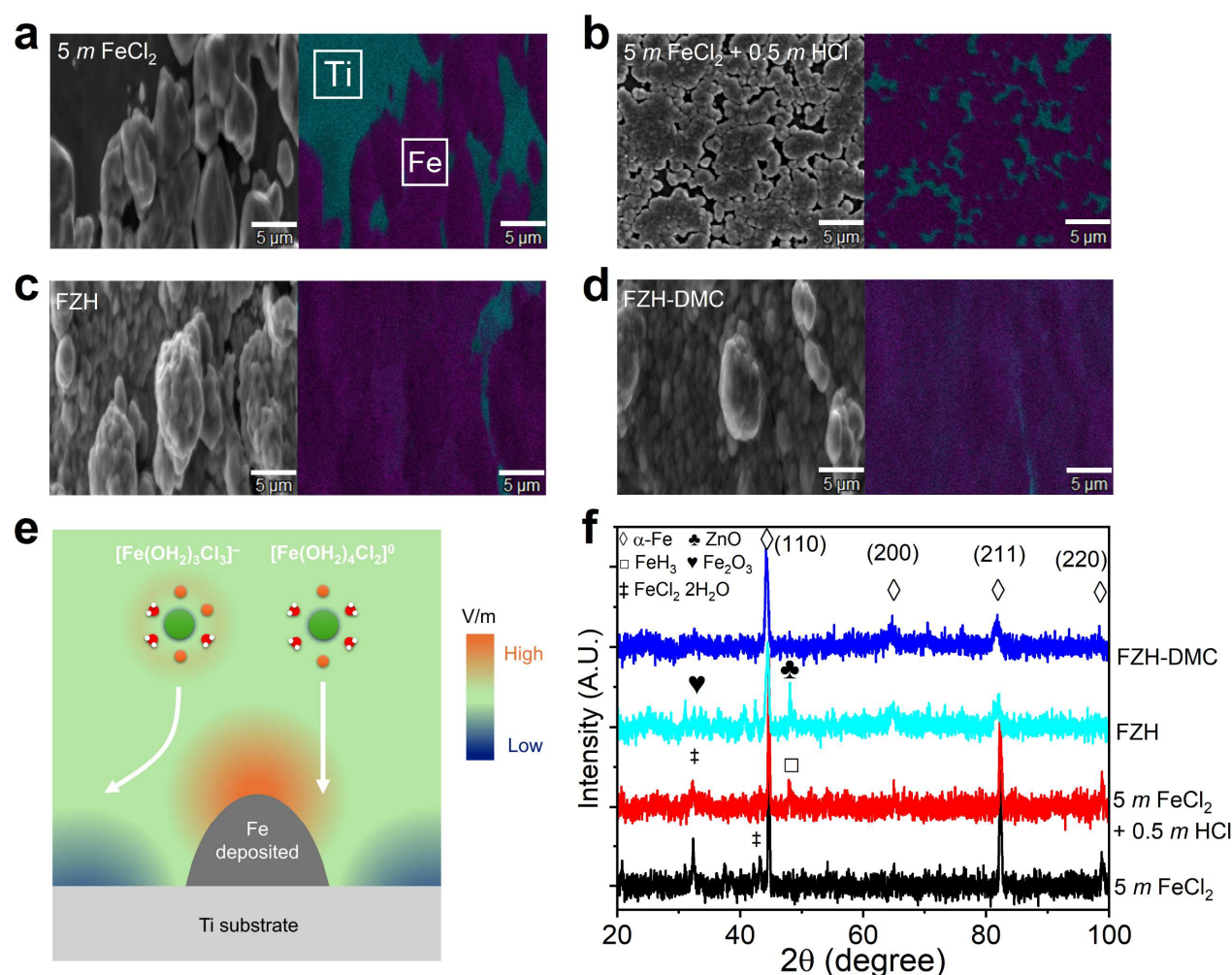
Figure 5. SEM images of the plated mass on a Ti current collector, taken after the 10 th discharge using electrolytes of (a) 5 m FeCl 2 , (b) 5 m FeCl 2 + 0.5 m HCl, (c) FZH, and (d) FZH-DMC. (e) Schematic illustration of the electric field distribution around the deposited iron mass and its effect on the ferrous ions with different solvation structures. (f) XRD patterns of the electrodes after the 50 th discharge using various electrolytes.
