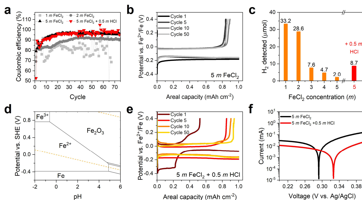
Figure 1. The electrochemical performance of FeMA in \text{FeCl}_2 electrolytes of various concentrations. (a) CE of the FeMA measured in three-electrode cells with a Ti foil working electrode and Fe metal foils as both counter and reference electrodes. (b) GCD profiles of FeMA in 5 m \text{FeCl}_2 . (c) The accumulated amount of \text{H}_2 due to HER after 50 cycles in the headspace of the cells employing various electrolytes. (d) Pourbaix diagram of the Fe species simulated
