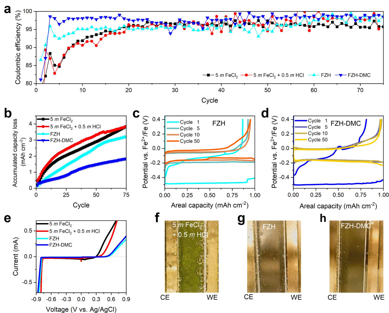
Figure 2. Electrochemical results of electrolytes using ZnCl 2 as a co-salt. (a) CE profiles of the FeMA measured in three-electrode Ti||Fe cells with an Fe reference electrode and (b) their accumulated capacity loss of the cells. GCD profiles of (c) FZH and (d) FZH-DMC electrolytes. (e) Stability window of various electrolytes measured by Linear Sweeping Voltammetry (LSV). Snapshot images captured from the videos ( Supporting Video 1 ) recorded using an optical microscope showing gas bubbles generated from the electrode surface, running with (f) 5 m FeCl 2 + 0.5 m HCl, (g) FZH, and (h) FZH-DMC as electrolytes.
