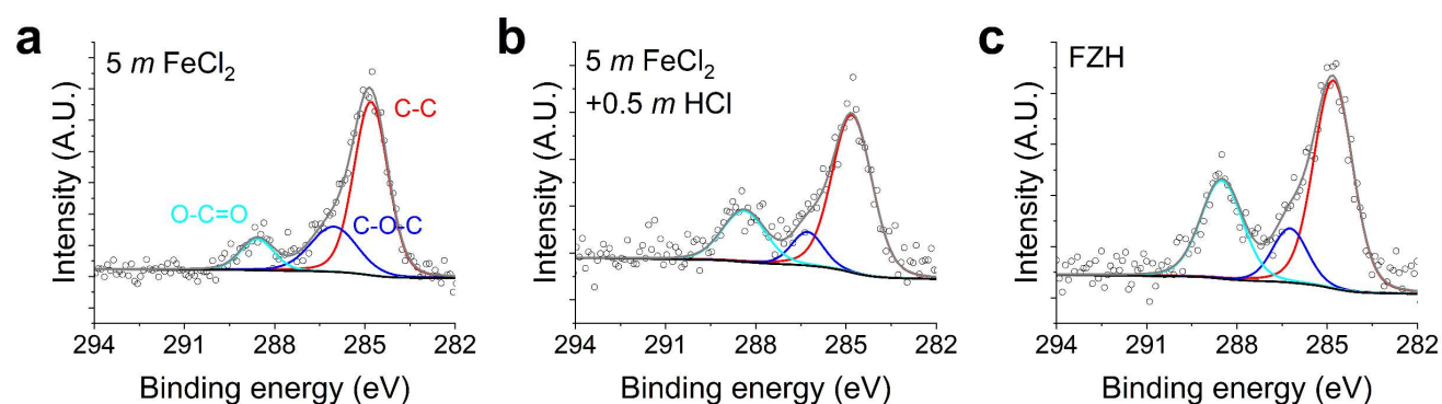
Supporting Figure S13. Peak deconvolution results of XPS C 1s spectra of the cycled working electrodes after 50 th plating, using (a) 5 m FeCl 2 , (b) 5 m FeCl 2 + 0.5 m HCl, and (c) FZH as the electrolyte.
