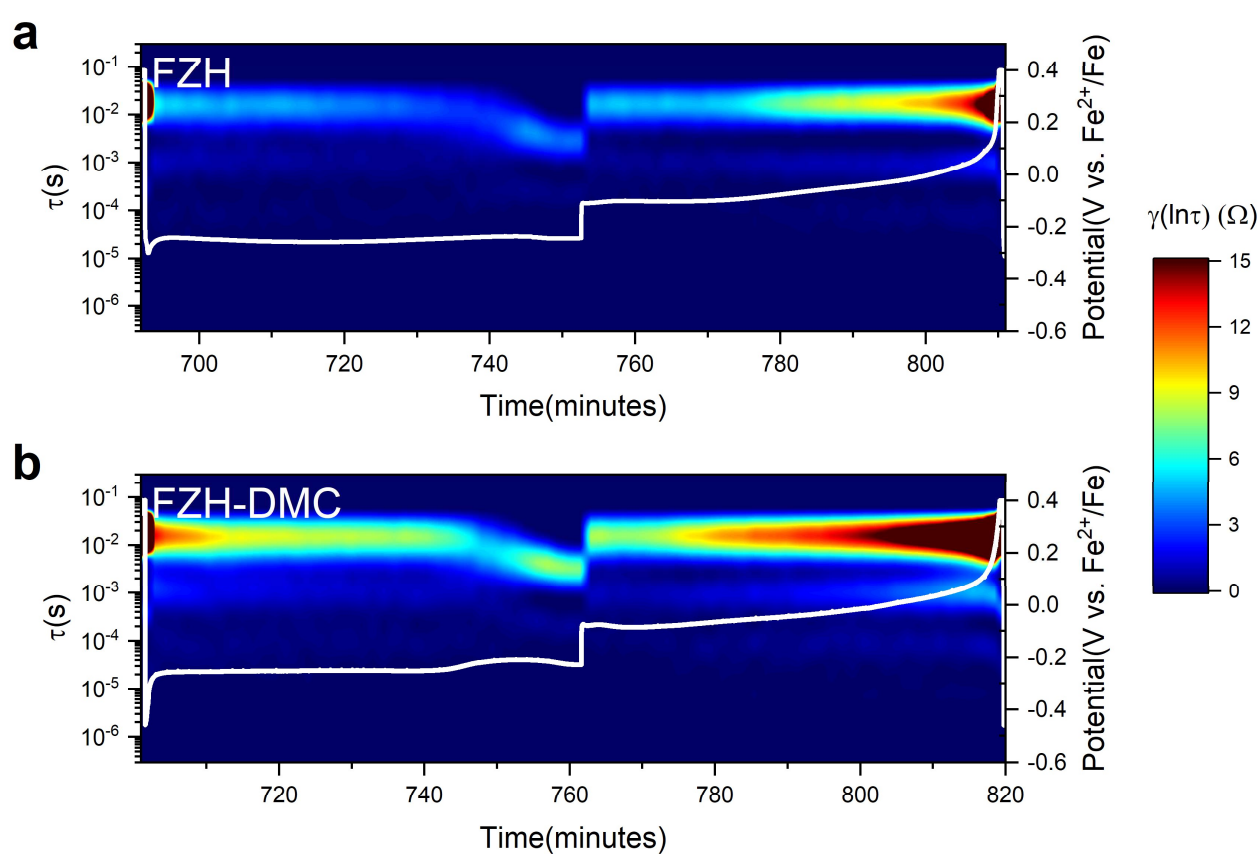
Supporting Figure S14. GEIS-DRT data of the seventh cycle of the plating and stripping on the Ti current collector using electrolytes of (a) FZH and (b) FZH-DMC.
