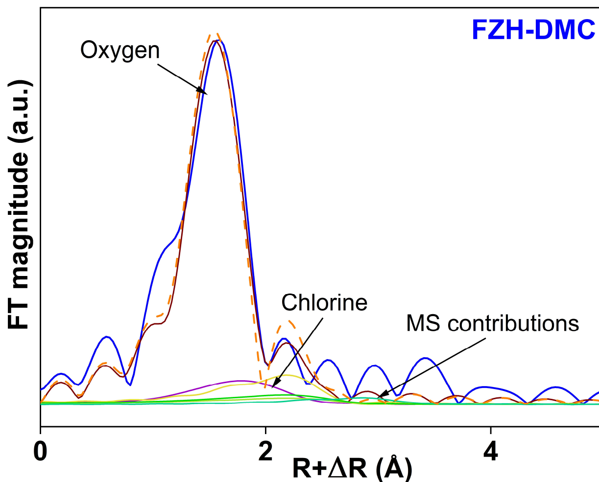
Supporting Figure S10. Atomic scattering paths observed in the Fourier transform (FT) magnitude of k^3 -weighted Fe EXAFS spectrum of the \text{FeCl}_2/\text{HCl}/\text{ZnCl}_2/\text{DMC} electrolyte calculated in the k range of 0 - 10 \text{ \AA}^{-1} . Experimental (blue solid line), best-fit EXAFS model in the R range of 0.5 - 5 \text{ \AA} (orange dashed line), and single scattering contribution of the Fe-O (brown line) and Fe-Cl neighbors (purple line), and contributions of multiple scatterings with a total path length up to 5 \text{ \AA} .
