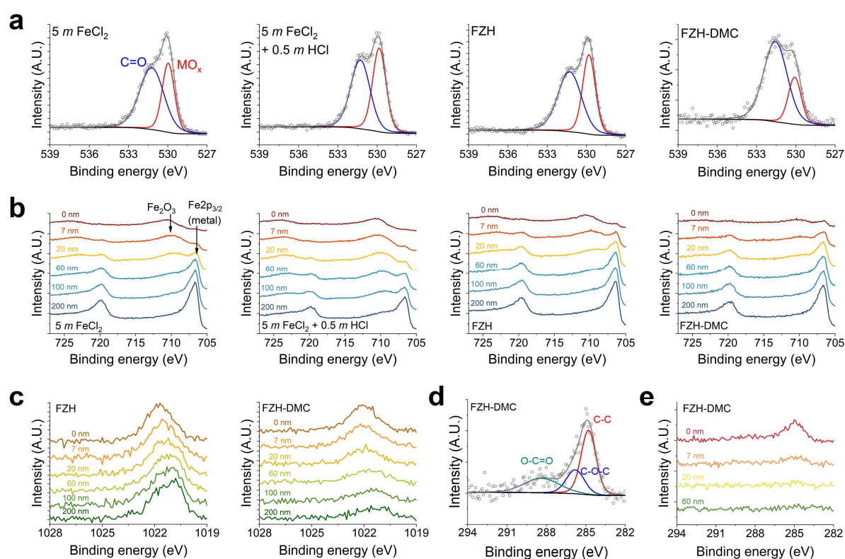
Figure 6. XPS profiles of anode after 50 th discharge with various electrolytes. (a) Peak deconvolution results of the O 1s spectra. Depth profiling of (b) Fe 2p and (c) Zn 2p spectra.
