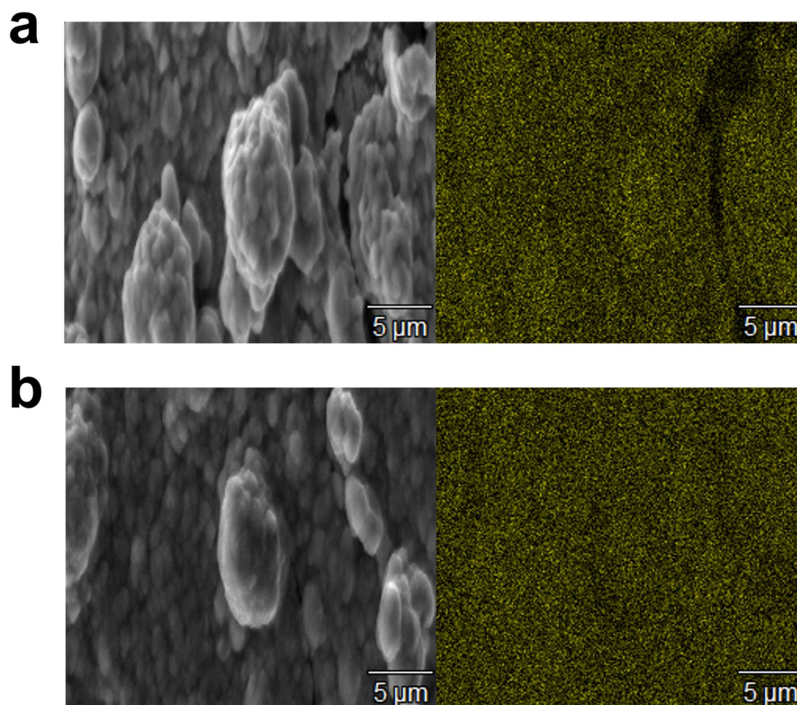
Supporting Figure S12. SEM-EDS mapping of the Zn element of the working electrodes using (a) FZH and (b) FZH-DMC electrolytes.
