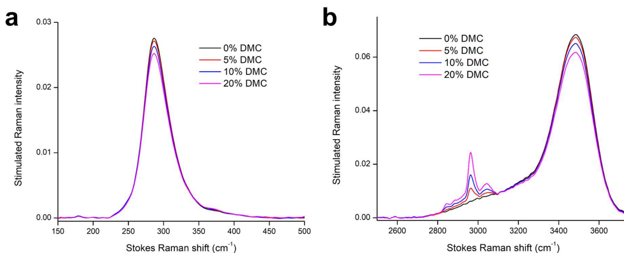
Supporting Figure S9. FSRs measurements of (a) low-frequency and (b) high-frequency regions of the FZH electrolytes with various amounts of DMC added.
