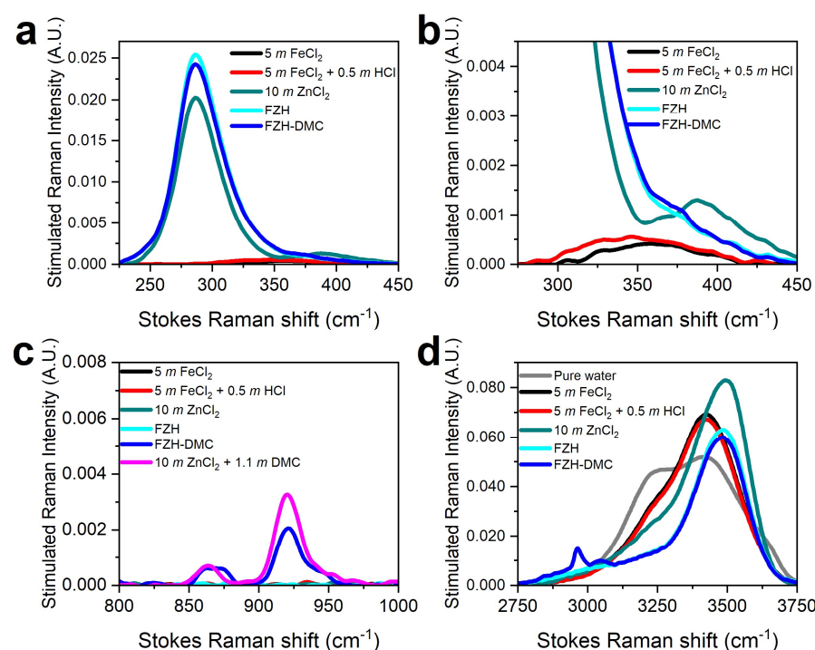
Figure 3. Ground-state FSRS spectra of various electrolytes in the (a) low-frequency region showing ion clusters, (b) enlarged view of the hydrated cluster region, (c) mid-frequency region depicting water-DMC interactions, and (d) high-frequency region of the H-bonding network of water.
