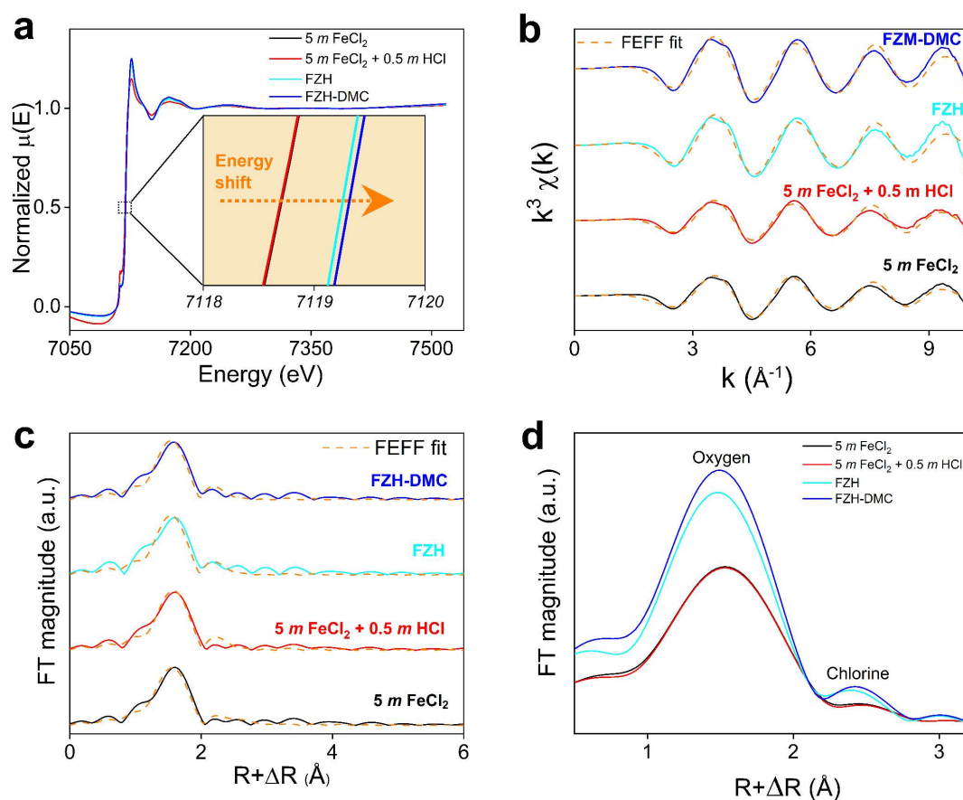
Figure 4. XAS measurements using synchrotron light source. (a) Normalized Fe K-edge XANES with an inset of the energy shift at \frac{1}{2} \mu(E) in concentrated chlorine electrolytes, (b) the k^3 -weighted Fe K-edge EXAFS spectra, and (c) their corresponding Fourier Transform (FT) magnitude of the electrolytes (solid line – experimental results, orange dashed line – best FEFF fits of the EXAFS model in the R range of 0.5 - 5\text{ \AA} ). (d) FT magnitude of the electrolytes overlapped.
