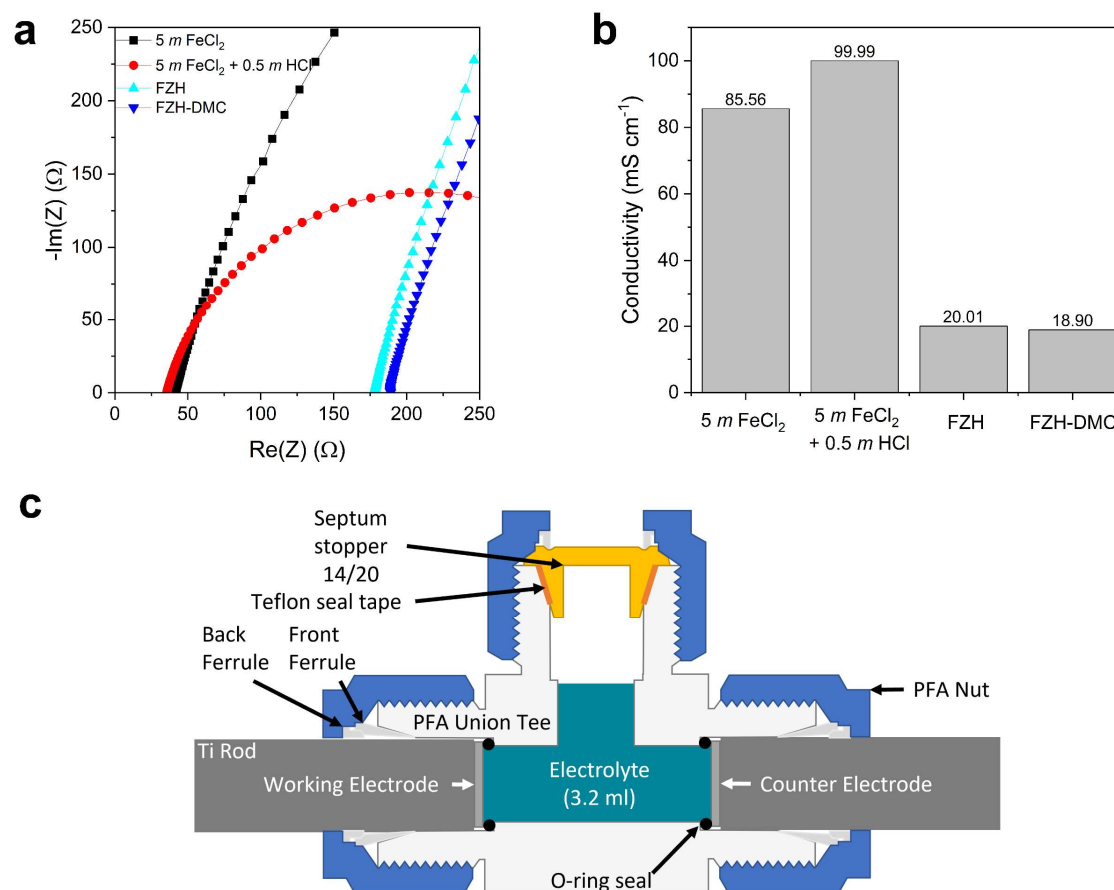
Supporting Figure S5. Ionic conductivity measurements of the different electrolytes. (a) Nyquist plots obtained from Fe||Fe symmetry cells, using separator-free Swagelok cells. (b) Conductivity of each electrolyte was calculated from the Nyquist plot. (c) Illustration of the separator-free Swagelok cell used for EIS.
