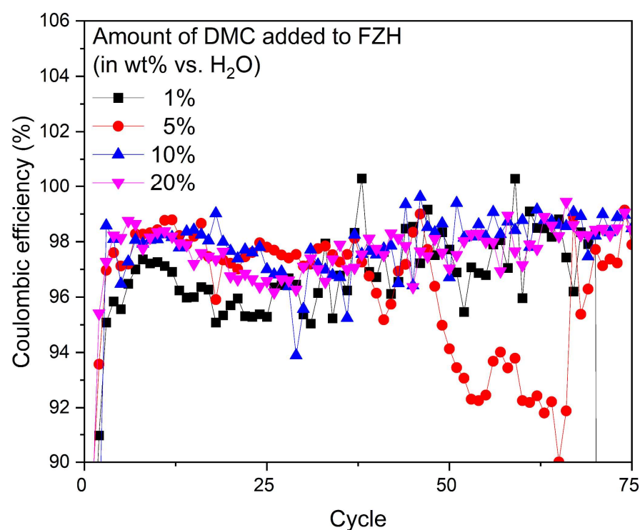
Supporting Figure S6. Coulombic efficiency data of the FZH electrolyte with the addition of various concentrations of DMC.
