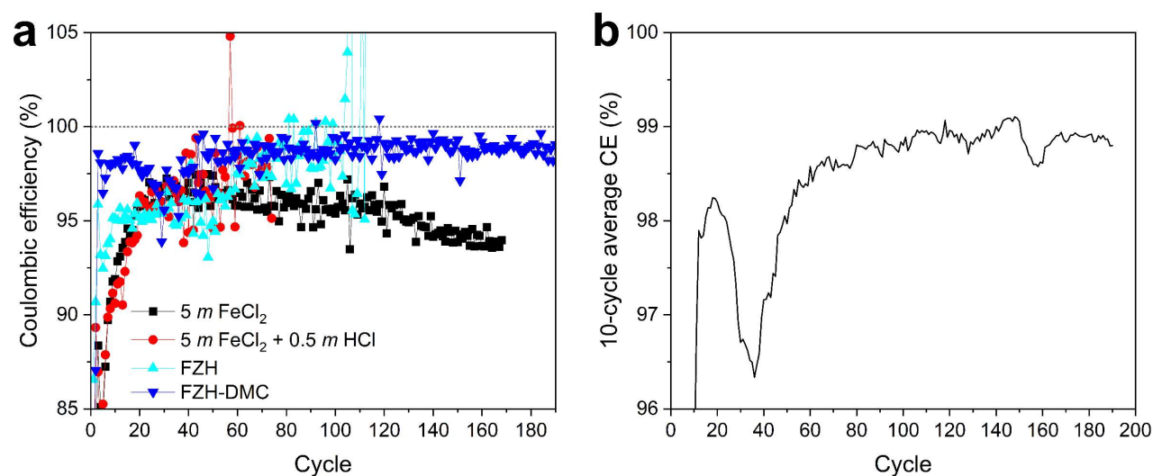
Supporting Figure S7. Additional Coulombic efficiency data of various electrolytes. (a) CE of Ti||Fe cells using various electrolytes until they fail. (b) Trends of 10 cycle average CE of FZH-DMC cell.
