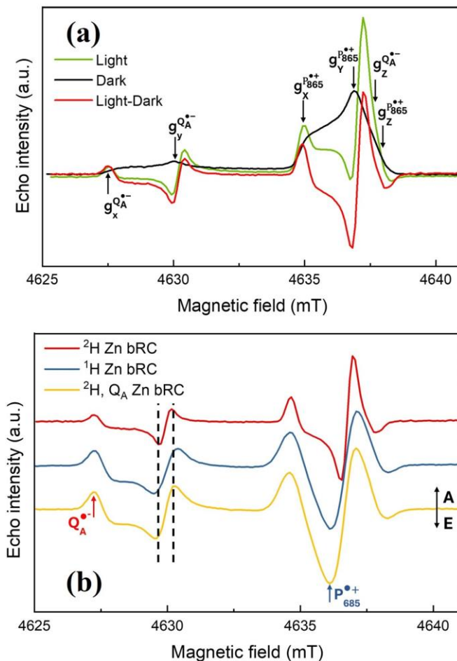
Figure 2: (a) Typical D-band field-swept pulsed ESE spectra of a deuterated bacterial reaction center sample recorded in the “dark” (black), “light” (green), and the “light” minus “dark” difference (red). The SCRPs spectrum (red) is consistent with our previously published spectra. 20 Arrows show the canonical positions of the g -tensors ( g_x , g_y and g_z ) for P_{865}^+ and Q_A^- . (b) SCRPs spectra from Zn bRCs with different biochemical treatments. Spectra were recorded as the difference “light” minus “dark” with a DAF time 700 ns. Arrows indicate the magnetic field positions where the two pulse ESE measurements were recorded. Note that the g_x and g_y regions of the partially deuterated sample (yellow) are narrower than those of the protonated sample (blue). The dashed lines in the figure are guide for the eye.
