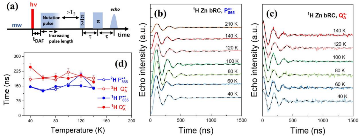
Figure 3: Rabi oscillations recorded in protonated, deuterated, and partially deuterated Zn bRCs. (a) Microwave pulse sequence for recording Rabi oscillations. For light induced states, a <10 ns laser pulse at 550 nm was applied 700 ns ( t_{\text{DAF}} ) before the first \pi/2 microwave pulse. Data were recorded within an excitation bandwidth of ca. 10 MHz. (b) Rabi oscillations as a function of temperature recorded for “light-dark” state of P_{865}^+ . (c) Rabi oscillations as a function of temperature recorded for “light-dark” state of A_1^- . (d) Temperature dependence of the Rabi oscillation decay times, t_0 , for “light-dark” states of P_{865}^+ and Q_A^- in all Zn bRCs.
