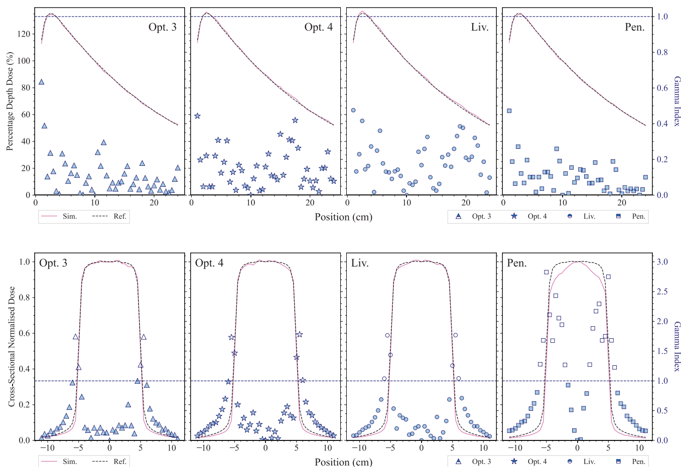
FIGURE 5 Results of the \gamma index test for all the tested EM constructors ( Opt3 , Opt4 , Liv , and Penelope ). Top row: longitudinal profiles. Bottom row: transverse profiles. Dotted line signifies a \gamma index of 1.
