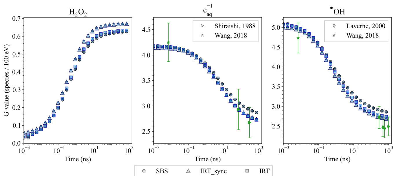
FIGURE 37 G-values of e_{aq}^- , H_2O_2 , and \bullet OH species calculated with the chemistry test, using the SBS , IRT-sync , and IRT models. Results obtained with Geant4 11.1. The error bars of the simulation results are within the symbols.
