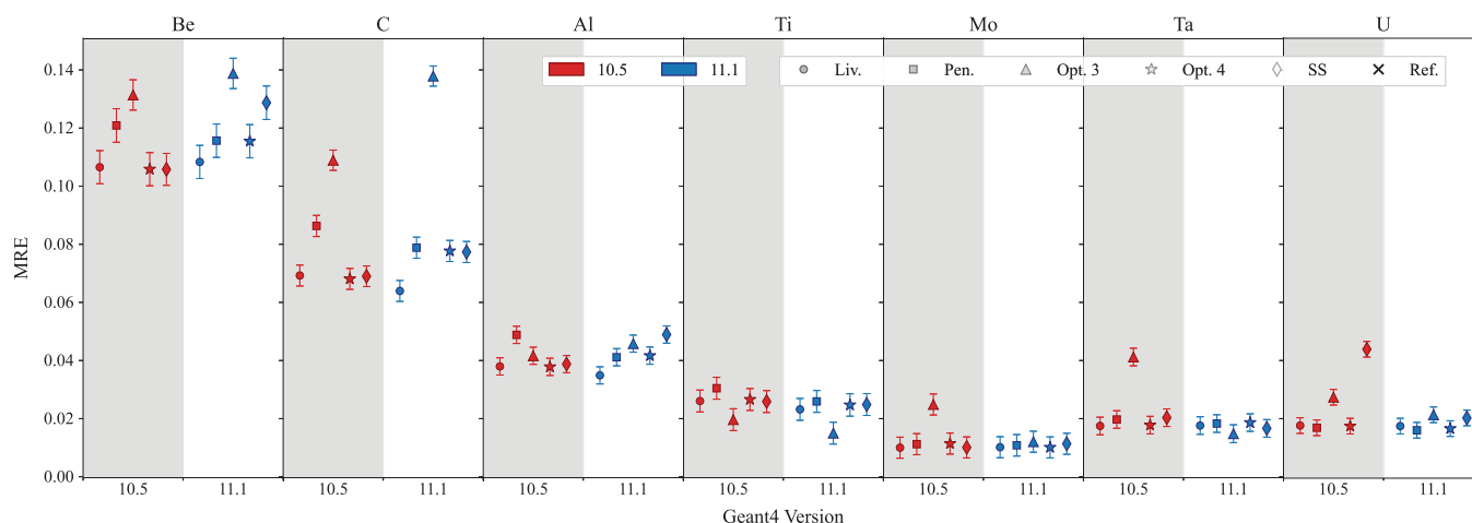
FIGURE 13 Mean relative error (MRE) calculated for Be, C, Al, Ti, Mo, Ta, and U targets, compared against the Sandia Lab experimental data. 58, 59 The MRE is calculated over the incident angles and electron energies under study. Here the uncertainties are provided as 1\sigma (see Section 2.1).
