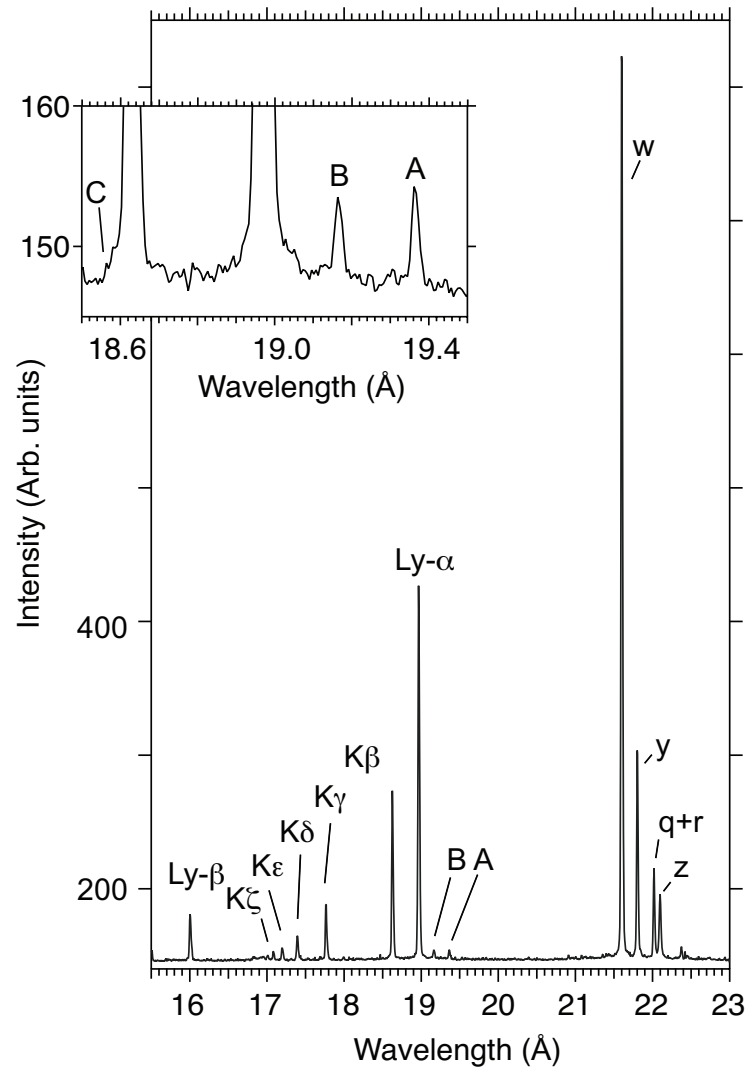
Figure 1. Spectrum of the K-shell emission lines of oxygen measured on the EBIT-I electron beam ion trap at Livermore. Besides the O VIII Lyman- \alpha and Lyman- \beta transition, the spectrum shows the 1sn p\ ^1P_1 \rightarrow 1s^2\ ^1S_0 Rydberg series lines of O VII, labeled K \beta through K \zeta . The n = 2 \rightarrow n = 1 O VII transitions are labeled w , y , and z , and the n = 2 \rightarrow n = 1 O VI transitions are labeled q and r . The two strongest n = 3 \rightarrow n = 1 O VI features of interest here are labeled A ( 1s2s3p \rightarrow 1s^22s ) and B ( 1s2s3p \rightarrow 1s^22s ); line C is labeled on the inset.
