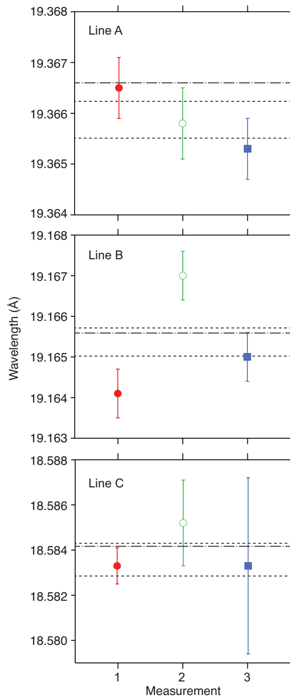
Figure 2. Comparisons of measured and predicted K-shell lines of O VI. Here the measurements by Togawa et al. [6] are shown in red (solid circles) and those by Beiersdorfer et al. [1] are shown in green (open circles). The present measurements are shown in blue (solid squares). The uncertainty-weighted average of the measurements of each line is indicated by the band enclosed by its upper and lower uncertainties, which are shown as dashed lines. The theoretical value is given by the dot-dashed line.
