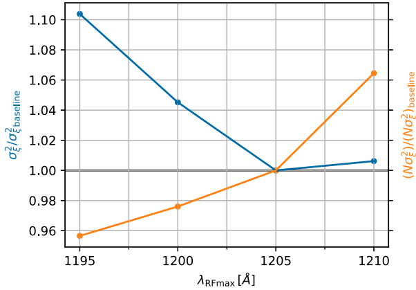
Figure 11. Comparison of the size of the errorbars in the Lyman- \alpha auto-correlation for different choices of \lambda_{RF,max} . The blue points show the errorbars size after averaging over all scales (given the small scale dependence of this quantity), and scaled to a reference value at \lambda_{RF,max} = 1205 \text{ \AA} . The orange points show the equivalent measurement but in this case for the product of errorbar sizes times the number of pixel pairs, removing the dependence on the number of pairs used in the measurement. Following the blue points, we observe an improvement in the precision of our auto-correlation measurements when increasing the \lambda_{RF,max} parameter, having the optimal value at 1205 \text{ \AA} . The orange points show that the quality of these added points actually decrease for higher wavelengths, revealing that the improved performance is only driven by the inclusion of more information in our sample. We selected 1205 \text{ \AA} as our default value as a compromise between these two features. We used data from the whole EDR + M2 data set for these measurements.
