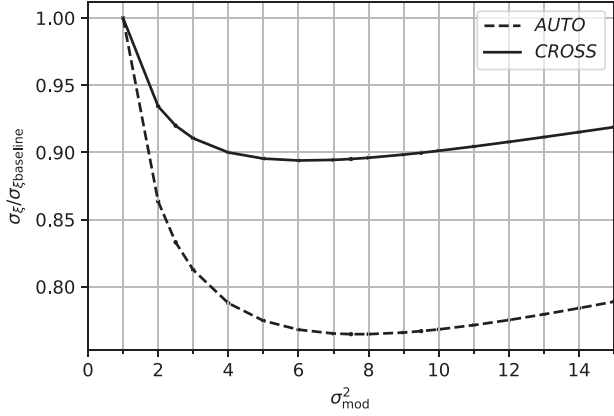
Figure 10. Measurement of the Lyman- \alpha auto- (solid) and cross- (dashed) correlation errorbars for different choices of the \sigma_{mod}^2 parameter, scaled to a reference value at \sigma_{mod}^2 = 1 . The value of the errorbars was averaged over all scales, given the small scale dependency. The \sigma_{mod}^2 parameter modified the inverse-variance weighting scheme as defined in equation (8), the use of a \sigma_{mod}^2 \neq 1 allows us for the optimization of the weighting scheme. In both auto- and cross-correlations, we observe a reduction in the size of the errorbars when we approach the optimal value of the \sigma_{mod}^2 parameter. This optimal value is slightly different, but in both cases is found around 7–8. In the optimal value, the improvement in the measurement of the auto-correlation is about 20 per cent and 10 per cent for the case of the cross-correlation. Both measurements have been performed with the full EDR + M2 data set.
