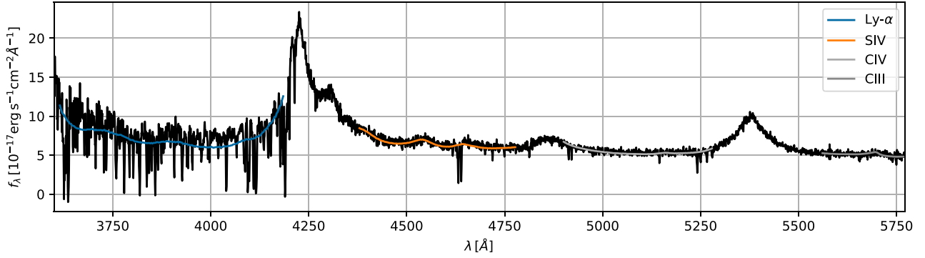
Figure 9. Example of a high signal-to-noise quasar spectrum. The mean expected flux \bar{C}(\lambda_{\text{RF}}) as in equation (4) is shown for the Lyman- \alpha , SIV, CIV, and CIII regions. The quasar has a redshift z_q = 2.495 and is identified as a DESI object with TARGETID = 39628443918272474. As in this example, we occasionally observe metal absorption in the calibration regions.
