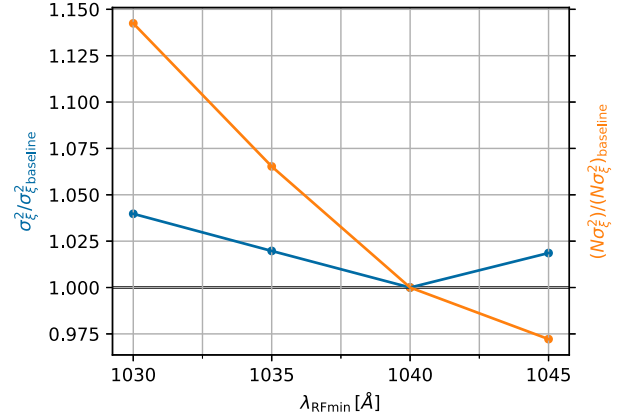
Figure 12. Identical measurements as the ones displayed in Fig. 11, in this case for values of \lambda_{RF,min} . The optimal wavelength is found at \lambda_{RF,min} = 1040 \text{ \AA} , while having similar features for the orange points: a decrease in the quality of the points added when approaching the emission line. Following the same arguments as in the case of \lambda_{RF,max} , we decided to keep the limit at 1040 \text{ \AA} . Again, these measurements were performed using the EDR + M2 sample.
