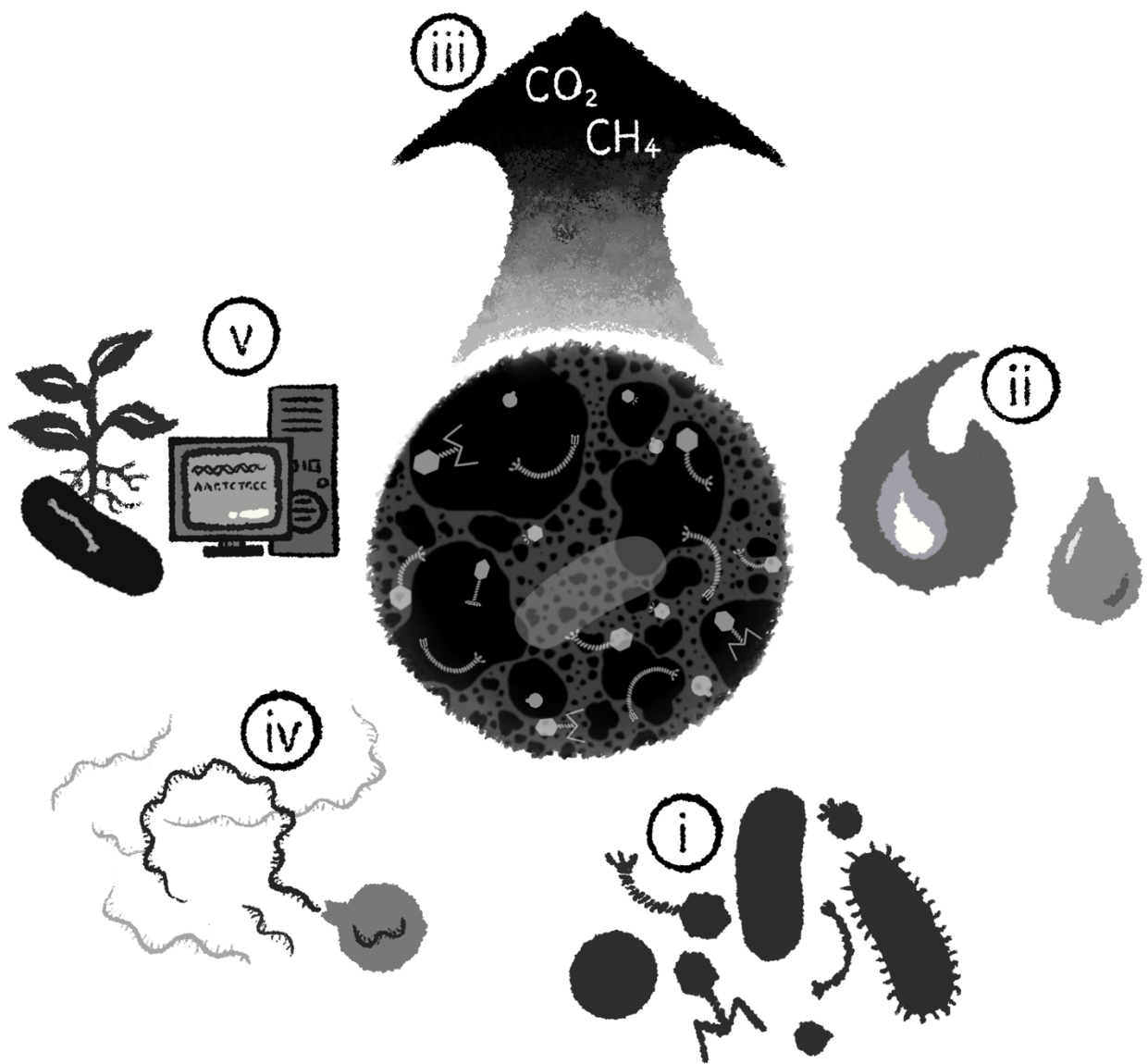
Figure 2. Soil viral talk topic areas. Topic areas covered by the talks during the International Soil Virus Conference 2024: (i) Viral diversity and community structure in the soil; (ii) Response of soil viral communities to ecosystem disturbance; (iii) Impacts of viruses on the soil microbiome and ecosystem processes; (iv) Soil RNA virome; (v) In vivo and in silico approaches to the study of soil viruses. All talks contributed to building up a more comprehensive picture of the soil virome and its wider impacts.
