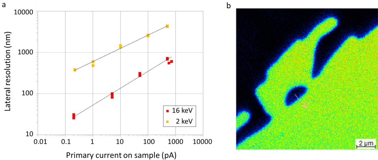
Figure 4. (a) Comparison of \text{Cs}^+ primary current vs. lateral resolution for the NanoSIMS-HR with 16 and 2 keV impact energy. (b) NanoSIMS-HR \text{Si}^- ion image of silicon grain in Al-Si sample using \leq 0.2 pA \text{Cs}^+ at 2 keV with lateral resolution = 378 nm.
