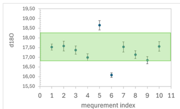
TEST C1, \delta^{18}\text{O} \sigma < 0.8\text{‰}
