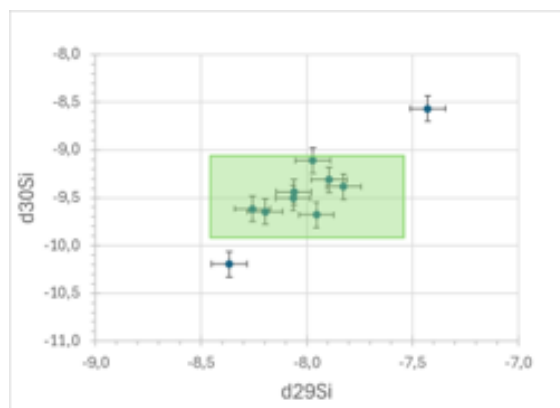
TEST B1, \delta^{29}\text{Si} and \delta^{30}\text{Si} \sigma < 0.45 ‰
