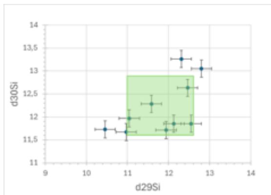
Fig. S6 (below). Isotope measurement plots for the nine specification tests. The shaded box in each graph represents the \pm 1 sigma results for the plotted data. See Table S1 for descriptions of the tests.
