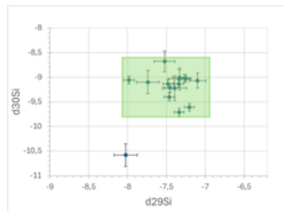
TEST B2, \delta^{29}\text{Si} and \delta^{30}\text{Si} \sigma < 0.6 ‰
