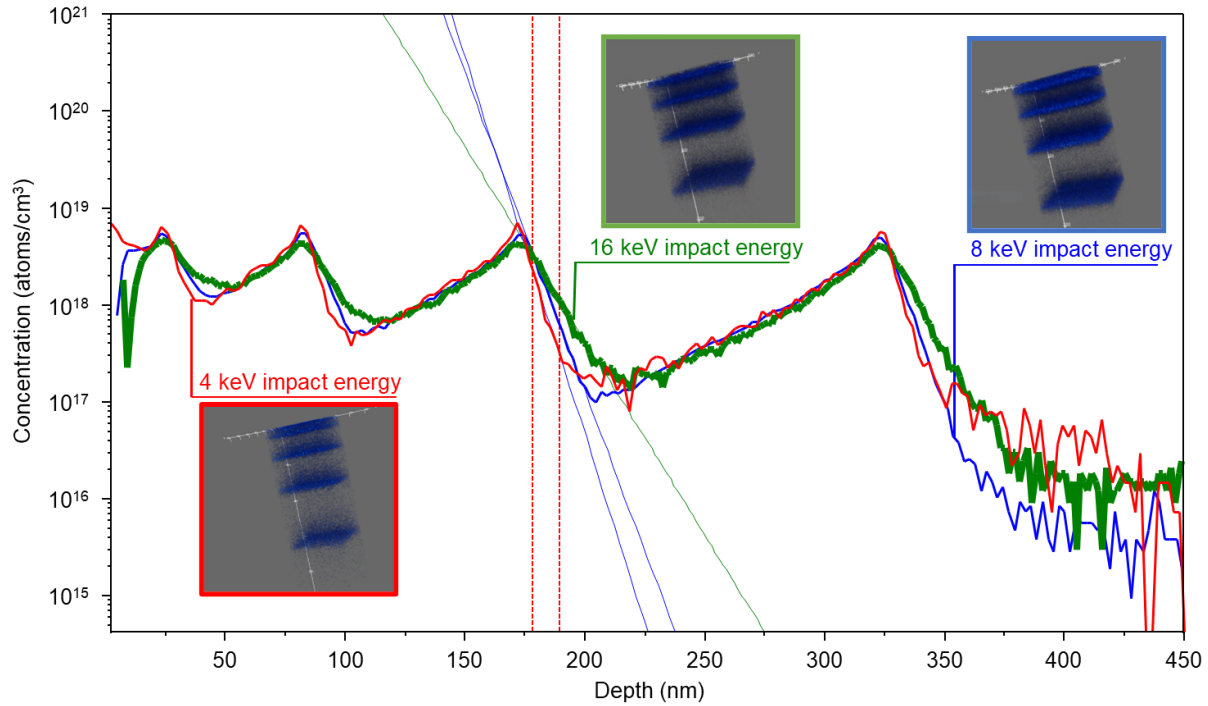
Figure 5. P depth profiles in a phosphorus-silicon delta layer sample with 16, 8 and 4 keV Cs + impact energy. Inset images show 2D projections of the 3D distribution of the 31 P - ions detected with depth in the silicon matrix for the three profiles. Note that depth resolution is measured on the trailing edge of the P delta layer because it presents a sharp chemical contrast (see Experimental Section).
