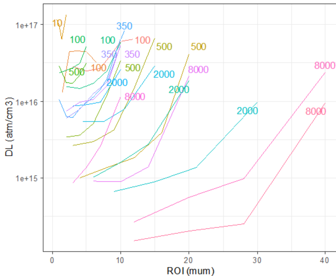
Fig. S5. P detection limit versus ROI size for individual analyses. The number associated with the individual curves is the Cs^+ primary ion current used for each measurement in pA. The raster size that resulted in the lowest detection limit for each primary current was tested empirically.
