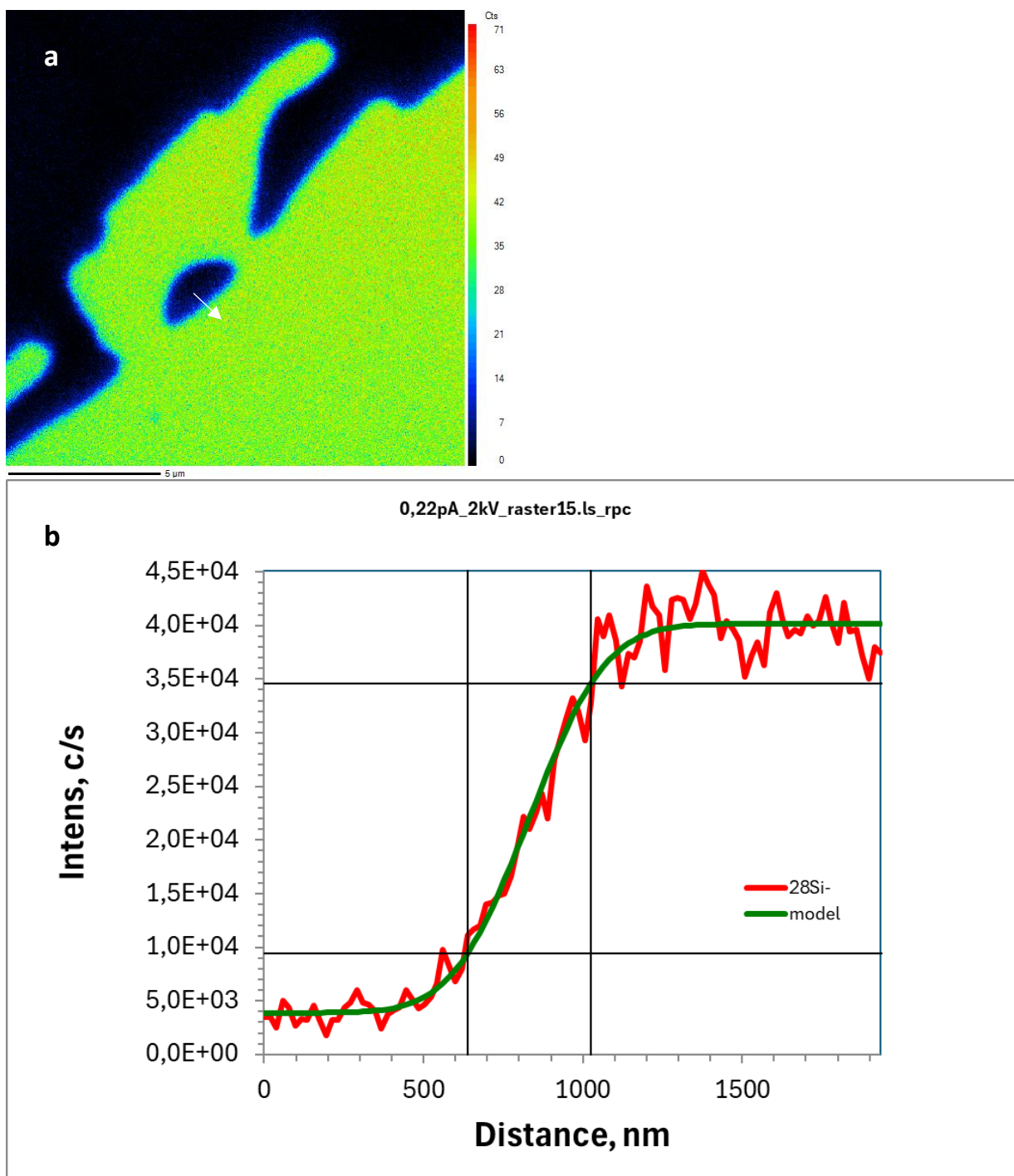
Fig. S3. Resolution at low impact energy. (a) ^{28}\text{Si}^- image collected with 0.2 pA \text{Cs}^+ with 2 keV impact energy, and (b) the measured lateral resolution for on an Al-Si sample (arrow in image center). The image is 15 \times 15 \mu\text{m}^2 and was collected with 512 \times 512 pixels.
