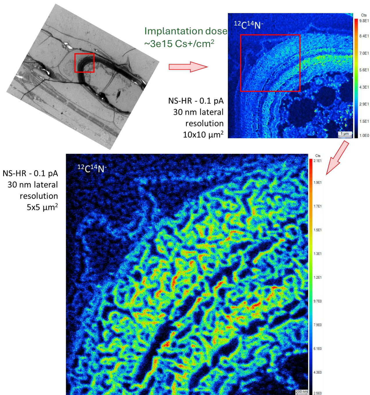
Fig. S2. Correlated TEM and NanoSIMS-HR \text{CN}^- images of an AMF vesicle in a P. hallii root at 16 keV impact energy. The images were collected in sequence. Boxes show the area of the subsequent image.
