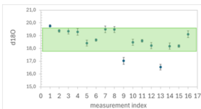
TEST C2, \delta^{18}\text{O} \sigma < 1.0\text{‰}
