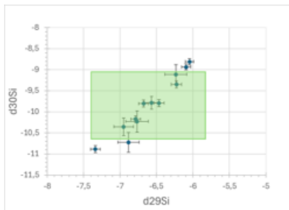
TEST B3, \delta^{29}\text{Si} and \delta^{30}\text{Si} \sigma < 0.8\text{‰}
