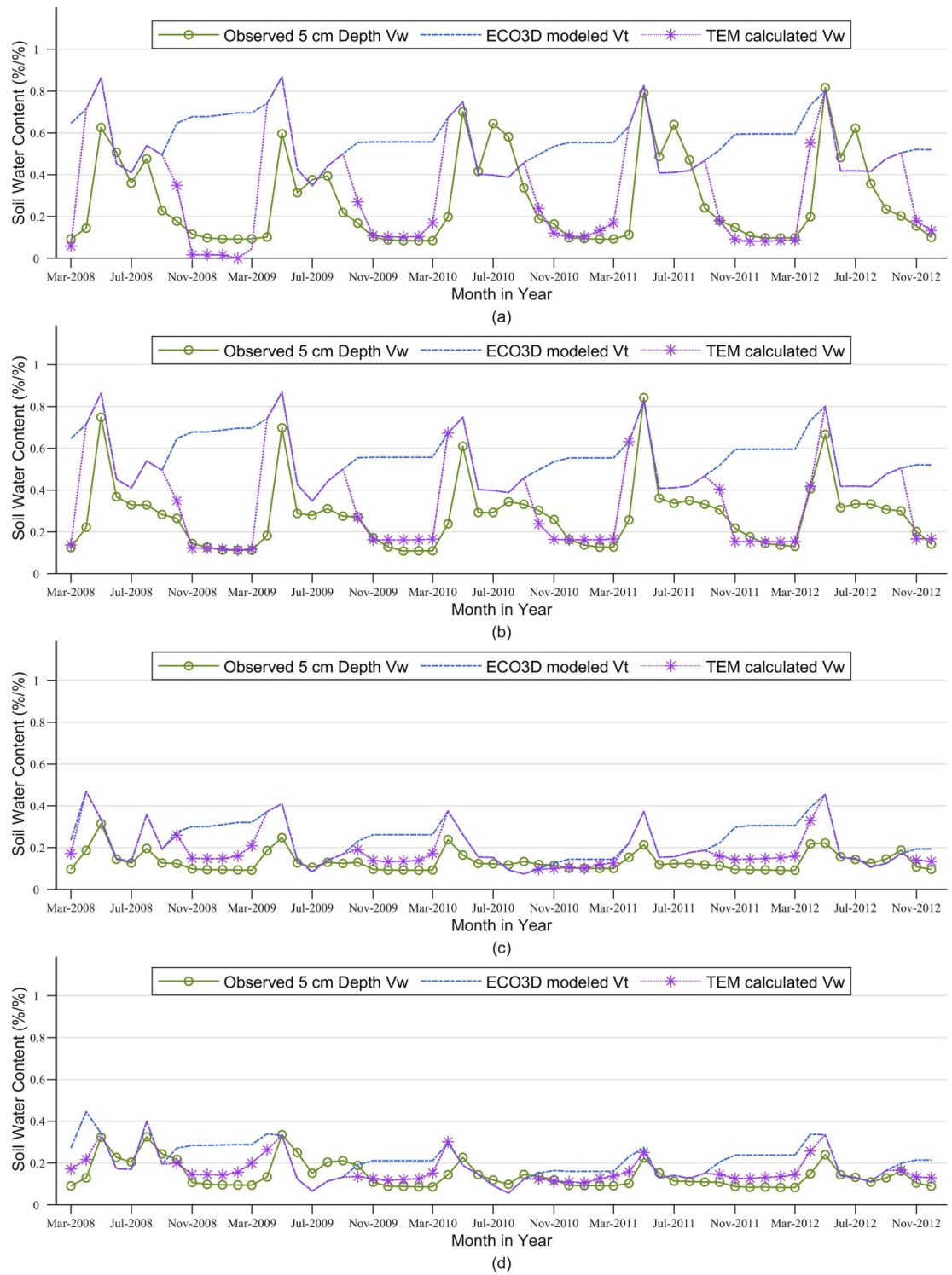
Figure 3. Comparison between ECO3D output total soil water content ( SWC/V_t ), TEM calculated soil liquid water content ( V_w ) during frozen season and measured 5 cm depth volumetric water content ( VWC/V_w ) at site FP1A (a), FP2A (b), UP1A (c), and UP2A (d) (table S2).
