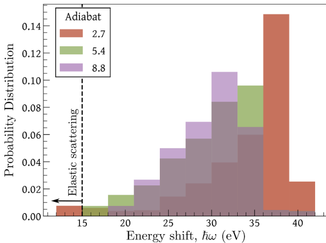
Figure 8. Probability distribution functions of the energy shift determined by the plasmon dispersion relation (equation (9)) for each target. As in figure 3(b), the energy shift is weighted by the electron density in each region and is determined for a 2 keV incident x-ray energy with a scattering angle of 40^\circ . A bin size of 3 \text{ eV bin}^{-1} is utilised based on the assumed spectral resolution of the detector. The black dashed vertical line indicates the highest observed energy of the elastic scattering peak.
