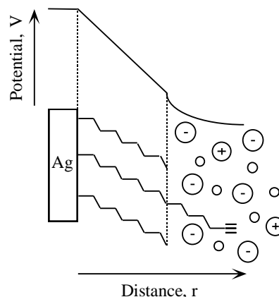
Figure 1. Schematic of the Ag/SAM/aqueous interfacial region.
