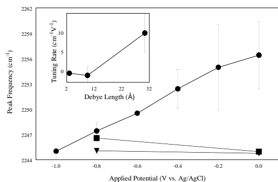
Figure 2. Peak frequency of nitrile stretching mode as a function ionic strength: (●) 10 mM NaClO 4 (■) 100 mM NaClO 4 and (▼) 1000 mM NaClO 4 . Inset shows the dependence Stark tuning rate of the nitrile stretching mode on the Debye length.
