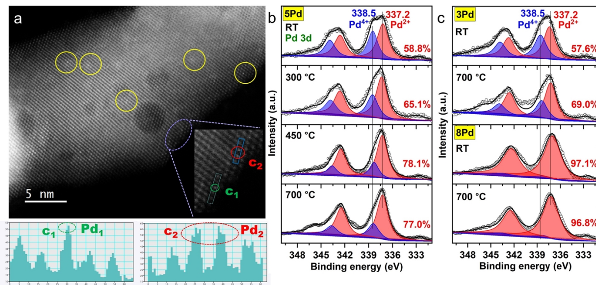
Figure 4. Local distribution and electronic properties of Pd species. (a) A representative STEM image of the spent 5Pd catalyst. More images can be found in Figure S5 . Insert shows the presence of both single ( c_1 ) and dimer ( c_2 ) Pd atoms on crystalline ceria. (b) The Pd 3d XPS spectra (scatter) of the as prepared 5Pd catalyst and the 5Pd catalyst after the methane combustion at 300 °C, 450 °C, and 700 °C. (c) The Pd 3d XPS spectra (scatter) of the as prepared and spent (after reaction at 700 °C) 3Pd and 8Pd catalysts. For (b, c), the fitted spectra and the contribution of Pd 2+ and Pd 4+ species are included for references. The Pd 2+ concentrations obtained from peak fittings are also listed next to the corresponding spectra.
