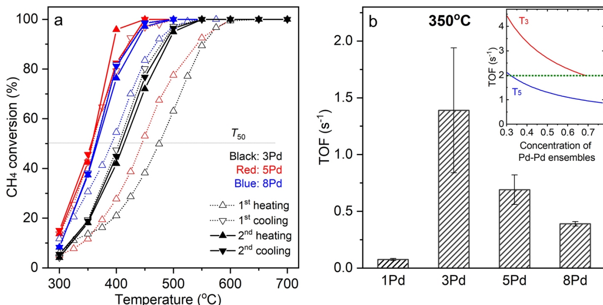
Figure 5. Catalytic properties of Pd-based catalysts for methane combustion. (a) Light-off and light-out curves of CH 4 oxidation over 1Pd, 3Pd, 5Pd and 8 Pd catalysts. Dashed line and open symbol stand for the first reaction cycle while the solid line and symbol stand for the second reaction cycle. The gas mixture consists of 0.5 % CH 4 and 2.5 % O 2 in He. (b) TOFs of 1Pd, 3Pd, 5Pd, and 8Pd at 350 °C. The inset shows the estimated range of TOFs of Pd-Pd ensembles in 3Pd (T 3 ) and 5Pd (T 5 ) catalysts.
