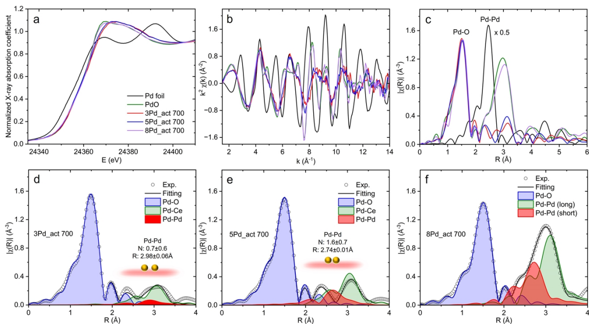
Figure 3. Local atomic structures of Pd in (3, 5, 8) Pd samples. (a) Pd K edge XANES, and (b) k-space, and (c) R-space EXAFS spectra of the spent 3Pd, 5Pd, and 8Pd catalysts. For comparison, the spectra of Pd foil and PdO are included. (b, c) share the same label as in (a). The comparison of experimental and the fitted spectrum of (d) spent 3Pd, (e) 5Pd, and (f) 8Pd catalysts. (d, e, f) also include the contribution of individual fitting paths for references.
