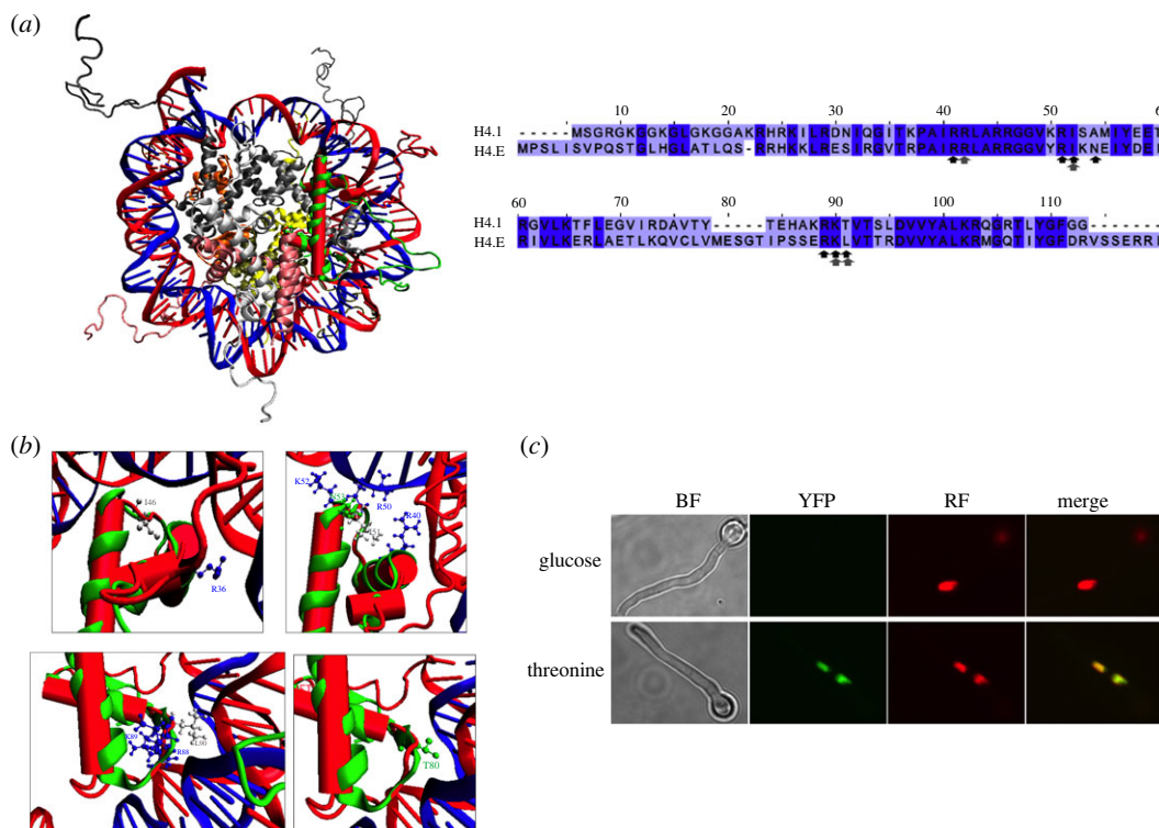
Figure 6. H4E fits in a nucleosome. (a) Left: superimposition of a model of H4E obtained through I-Tasser (https://zhanggroup.org/I-TASSER/) (solid red) with a nucleosome containing a canonical H4 derived from 1KX5 [43]. The second canonical H4 molecule is shown in orange; H2A: yellow and greyish white; H2B: tan and pink; H3: dark grey and intermediate grey. Right: alignment of the amino acidic sequences of A. nidulans H4.1 and H4.E. Residues that contact DNA in H4E I-Tasser model are indicated with black arrows (Arg40, Arg50, Ile51, Lys52, Asn53, Arg88, Lys89 and Leu90), while those of the canonical histone are indicated with grey arrows (Arg36, Ile 46, Lys79, Thr80). (b) Detailed view of proposed DNA-H4E contact zones. Basic residues are coloured in blue, polar residues in green, and neutral in grey. (c) Bimolecular fluorescence complementation (BiFC) microscopy to show the interaction of H4E with canonical histone H3. H3::YFP N and H4E::YFP C fusions are overexpressed from the P alcA promoter when induced with threonine (lower panels). Glucose inhibits the expression of the fusions (upper panels). BiFC YFP signals are visible in green in the nuclei, where they co-localize with mRFP-tagged histone H1 (HhoA), seen in red. BF: bright-field microscopy. Merge: co-localization of YFP and mRFP signals. Growth conditions are detailed in Materials and methods. Black scale bars, 10 μm.
