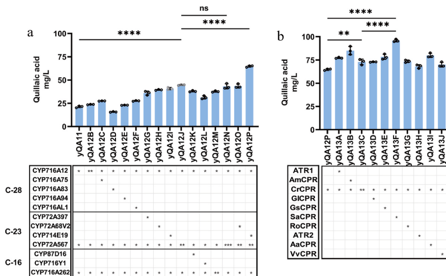
Fig. 4. Combinatorial expansion of enzyme network and taking advantage of network effects increased quillaic acid production. a, Quillaic acid titer of new strains established by rescreening the CYP library in strain yQA11, and b, rescreening the CPR library in strain yQA12P.
