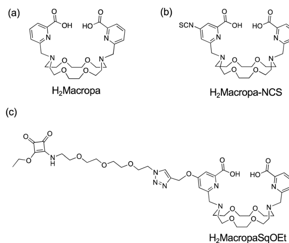
Fig. 1 Structure of (a) H 2 Macropa, (b) H 2 Macropa-NCS from Radchenko and Wilson, 39 and (c) H 2 MacropaSqOEt (this work).
