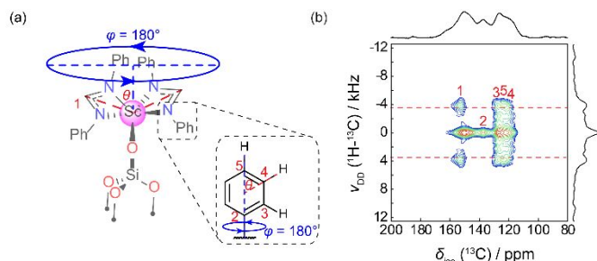
Figure 1. (a) Possible dynamic modes of supported scandium formamidate complexes. The inset shows the C_2 rotation of Ph moieties. (b) 2D dipolar recoupled PARS spectrum of Sc\{\kappa^2-(NPh)_2CH_2\}_2/SiO_{2,60\text{\AA}} acquired at -100^\circ\text{C} , with assignments described according to the structure in (a).
