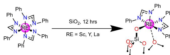
Scheme 1. Representation of the grafting procedure of the rare earth formamidate complexes to silica gel.
