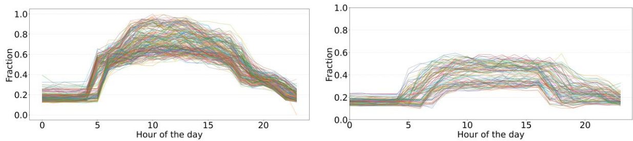
Fig. 4. Clusters of electricity consumption profiles (weekdays: left, weekends: right).
