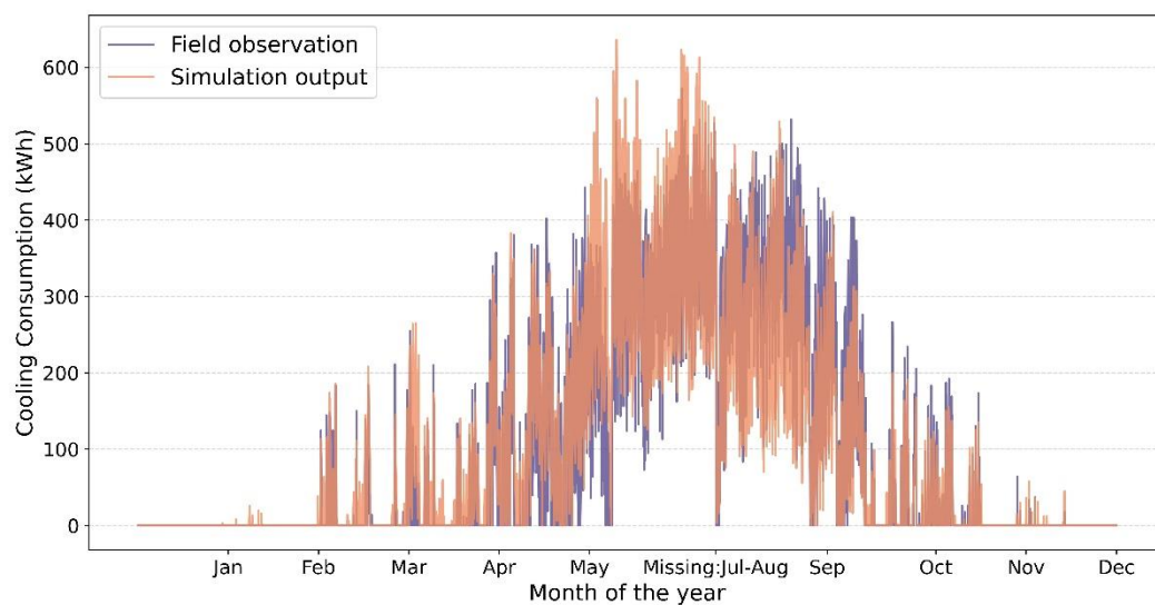
Fig. 11.b. Comparison of cooling consumption.
