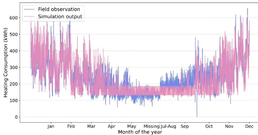
Fig. 11.a. Comparison of heating consumption.
