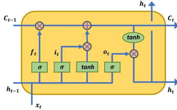
Fig. 7. LSTM unit structure.
