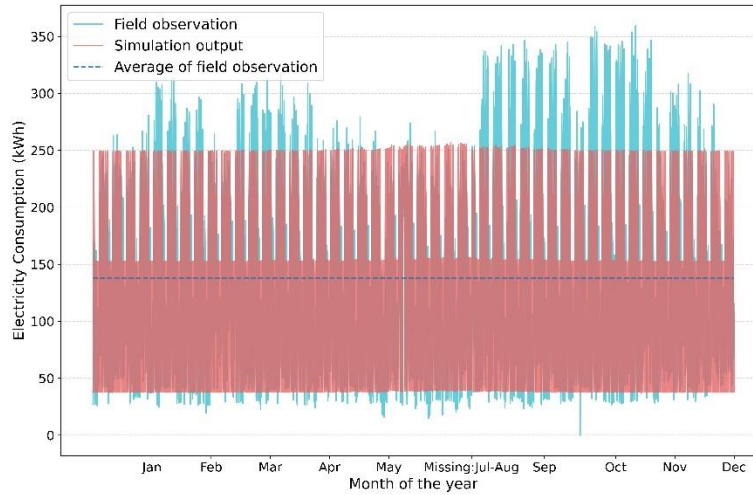
Fig. 13.c. Hourly electricity consumption distribution
