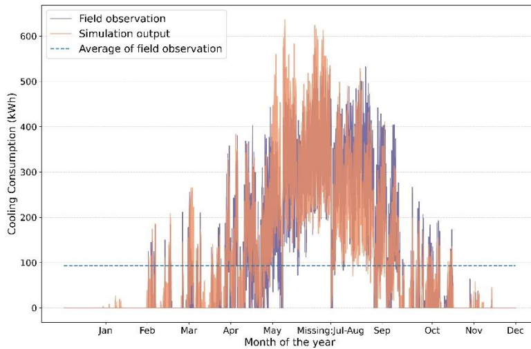
Fig. 13.a. Hourly cooling consumption distribution
