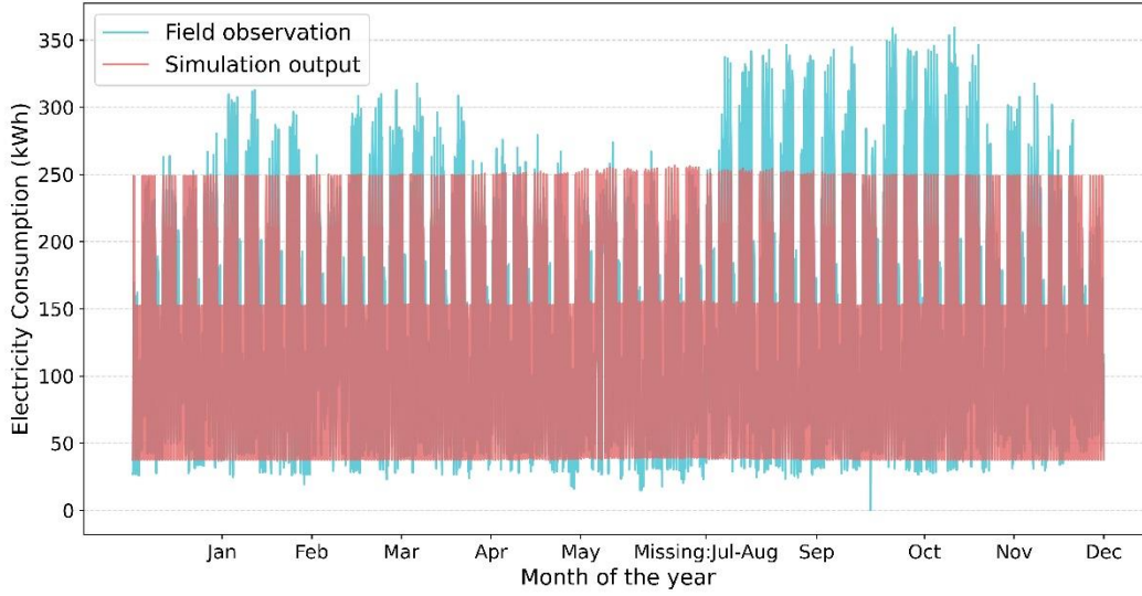
Fig. 11.c. Comparison of electricity consumption.
