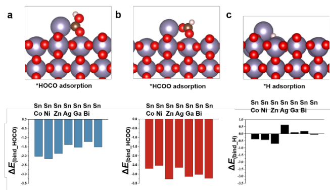
Fig. 6 DFT optimized configurations and binding energy between Sn-based catalysts and (a) \text{HOCO}^* , (b) \text{HCOO}^* or (c) \text{H}^* . Sn: gray, C: brown, O: red and H: pink. \text{X}^* represents species X adsorbed on the catalyst.
