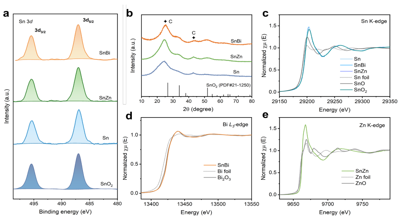
Fig. 4 Electronic structure of Sn, SnBi, and SnZn. (a) Sn 3d XPS spectra of Sn, SnBi, SnZn, and SnO 2 reference; (b) XRD. (c) XANES spectra at the Sn K-edge of Sn, SnBi, SnZn, Sn foil, SnO, and SnO 2 standards. (d) XANES spectra at the Bi L 3 -edge of SnBi, Bi foil, and Bi 2 O 3 standard. (e) XANES spectra at the Zn K-edge of SnZn, Zn foil, and ZnO standard.
