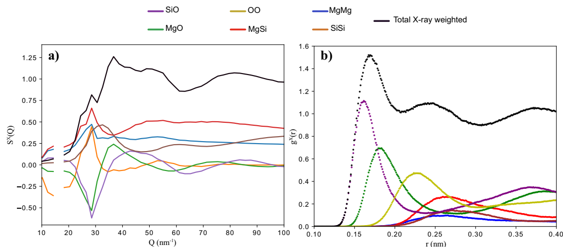
Fig. 3 | AIMD calculations on \text{MgSiO}_3 glass Hugoniot at 6000 K ( P = 167 GPa; density of 5.17 g/cm 3 ). a Total and partial Faber-Ziman structure factors S^X(Q) . b Total and partial radial distribution functions g^X(r) .
