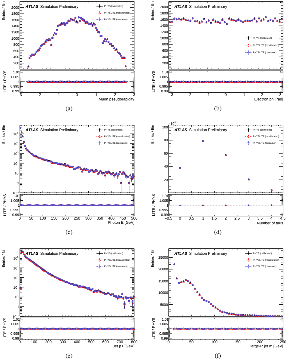
Figure 2: Validation of PHYSLITE by comparing object kinematics to those from objects in PHYS that have been calibrated using CP algorithms (black circles), for (a) muons, (b) electrons, (c) photons, (d) hadronic taus, (e) small-radius jets and (f) large-radius jets. Two comparisons are overlayed, either directly using the stored objects from PHYSLITE (red triangles) or passing them again through their respective CP algorithms (blue stars). Plots taken from Ref. [8].
