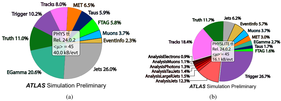
Figure 1: The composition of a Run 3 t\bar{t} sample in (a) PHYS and (b) PHYSLITE format. The disk size from PHYS is dominated by the jet collections, while PHYSLITE is currently dominated by the trigger information. The containers that hold the calibrated analysis objects in PHYSLITE are shown in the red slices. Plots taken from Ref. [8].
