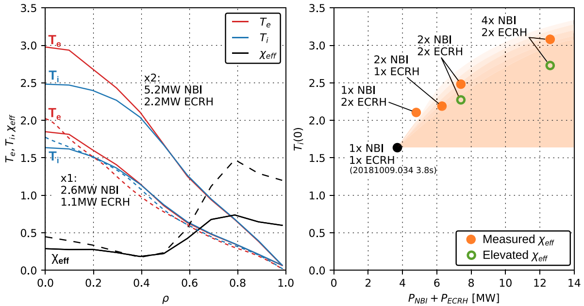
Figure 15. Results of NTSS transport simulations at constant anomalous heat diffusivity and density. (a) Electron (red) and ion (blue) temperature profiles from simulations based on the heat diffusivity profile (solid black) determined from steady state phase of discharge 20181009.034 with 2.6 MW of NBI and 1.1 MW of ECRH. Lower profiles show the simulation matched to the original discharge (dashed blue/red) and upper profiles show a doubling of both NBI and ECRH power deposition profiles. (b) Central ion temperature for original (black) and for different combinations of ECRH and NBI power scaling (orange points) with respect to the original discharge. Green points show two simulations assuming increased anomalous transport outside of the steep density gradient region (dashed \chi in (a)). Orange shaded region shows the range of possible values from these simulations through to the ITG dominated scenario, depending on particle transport.
