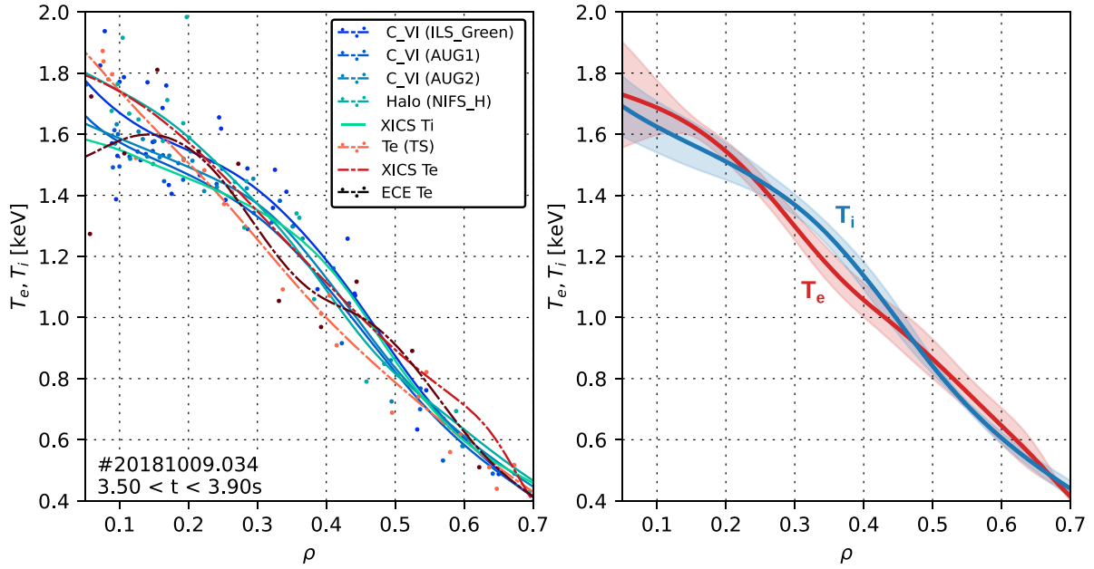
Figure 10. (a) Data points and fitted radial profiles from different diagnostics for ion (blue) and electron (red) temperatures during NBI plasma with low power O2 ECRH. (b) Average and spread (FWHM) of individual fits as an estimation of systematic errors.
