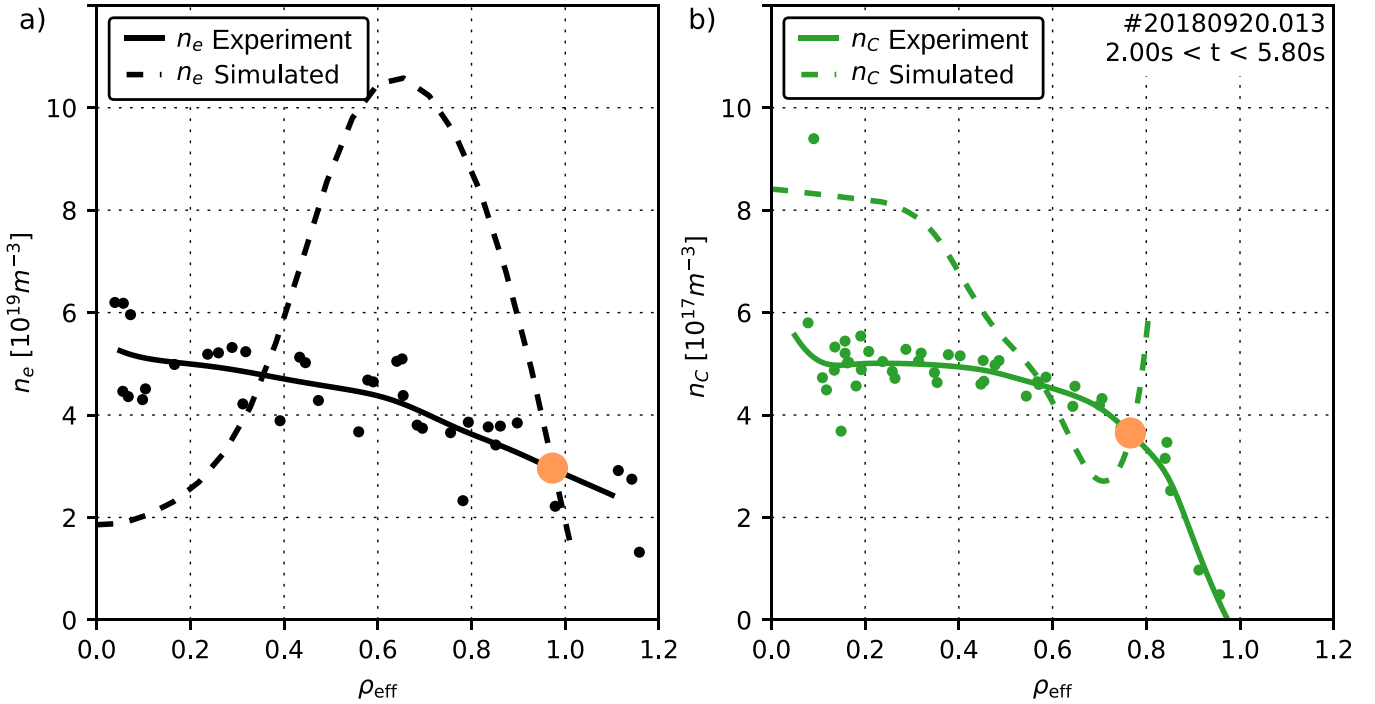
Figure 1. Observed (a) electron and (b) carbon density data (points) and profiles (solid) in typical steady-state gas-fuelled and centrally ECRH heated W7-X plasmas. Dashed profiles show simulated (a) electron density profiles assuming neoclassical particle transport given the experimental temperature profiles and (b) carbon density profiles assuming neoclassical impurity transport given experimental electron density and temperature profiles.
