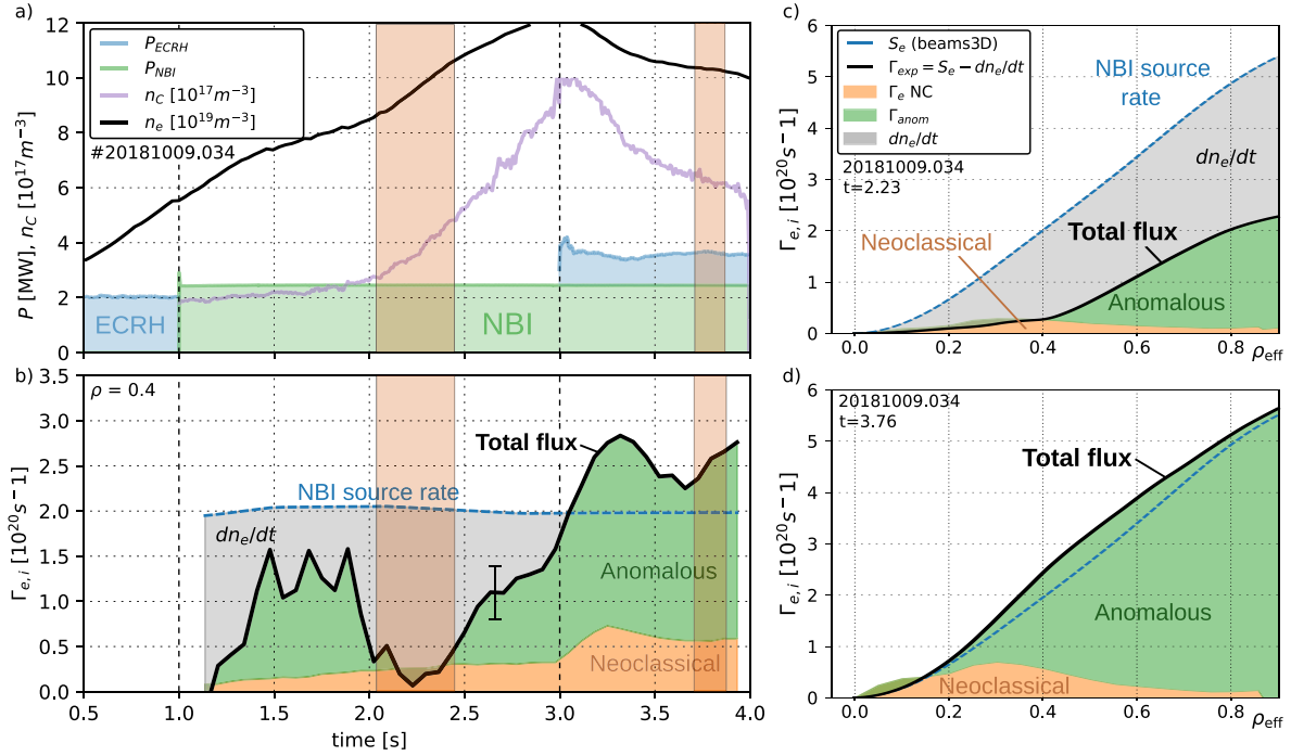
Figure 8. Time trace at \rho = 0.4 (b) and radial profiles at selected time points (c), (d) of particle fluxes during NBI/ECRH mixed heating discharge #20181009.034. Experimental fluxes (black) are calculated by subtracting the rate of change of density (shaded gray when positive) from the NBI particle source rate (blue dashed). The difference of experimental and calculated neoclassical (orange) fluxes is attributed to anomalous transport (green). Power and density traces (a) from figure 6 are repeated for reference. The profiles are time-averaged over the pure-NBI phase with maximum density rise (b) and the mixed NBI+O2 ECRH phase with highest stable performance (d), which are highlighted (orange) in the time trace. A representative error bar is shown in (b) derived from the average noise level of dn_e/dt .
