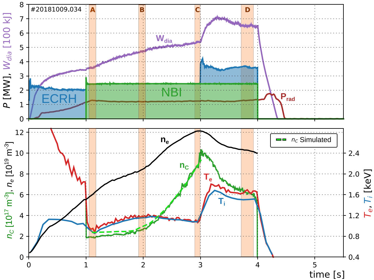
Figure 6. Time traces of global powers and energy (top) and densities and temperatures (bottom) for discharge #20181009.034 which included phases of ECRH X2, NBI and mixed NBI + ECRH O2 heating. The averaged time range of the profiles shown in figure 7 are highlighted in orange. Also shown is the core carbon density (dashed green) from transport simulations assuming only neoclassical transport during the pure-NBI phase.
