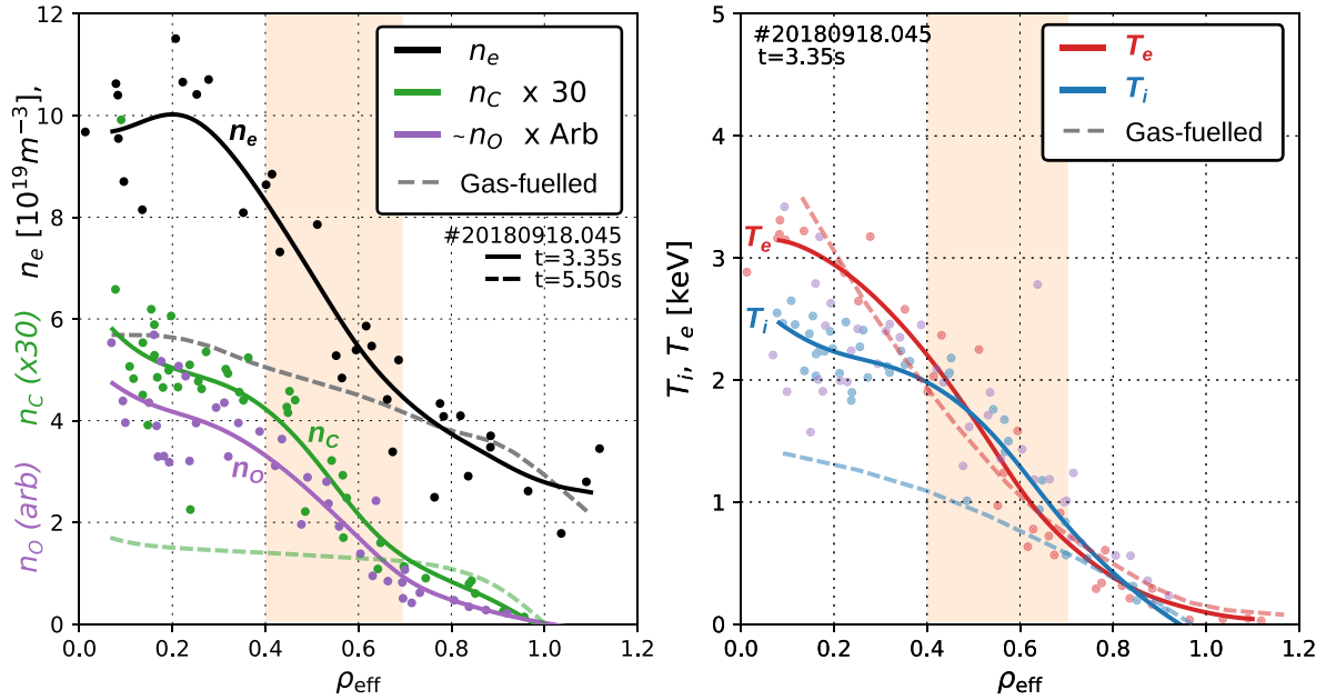
Figure 2. (a) Electron (black), carbon (green) and oxygen (purple) density profiles during a high performance phase after pellet injection (solid) and in matching conditions without pellet injection (dashed). (b) Electron (red) and ion (blue) temperature profiles in the same cases. Oxygen profiles are arbitrarily scaled as validated charge exchange rate coefficients are not yet available. Ion temperatures derived from the oxygen charge exchange emission (purple dots) are also included in the T_i fit. The region of steep gradients is highlighted in orange.
