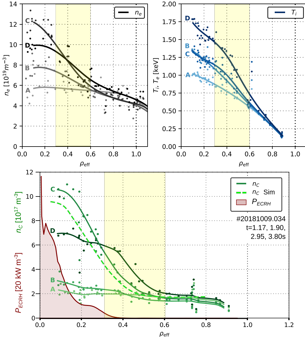
Figure 7. Electron density (a), ion temperature (b) and carbon density (c) profiles at selected points in discharge #20181009.034. The profiles are averaged over the time windows A,B,C and D shown in figure 6. The O2 ECRH deposition profile in red (c) and the region of strongest density gradient is highlighted in yellow. A simulation of the expected carbon density profile is shown as a dashed green line in (c) for time point C assuming only neoclassical transport.
