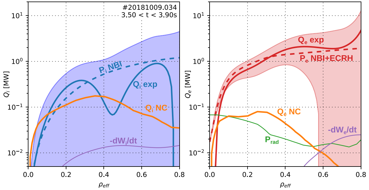
Figure 11. (a) Ion and (b) electron power balance profiles. Experimental fluxes (solid red/blue, with uncertainty band) compared to calculated neoclassical fluxes (orange). Components of the experimental fluxes are also shown: ECRH+NBI power deposition (dashed red/blue), change of stored energy (purple) and radiation (green). The uncertainty band represents the range of T_e and T_i measurements.
