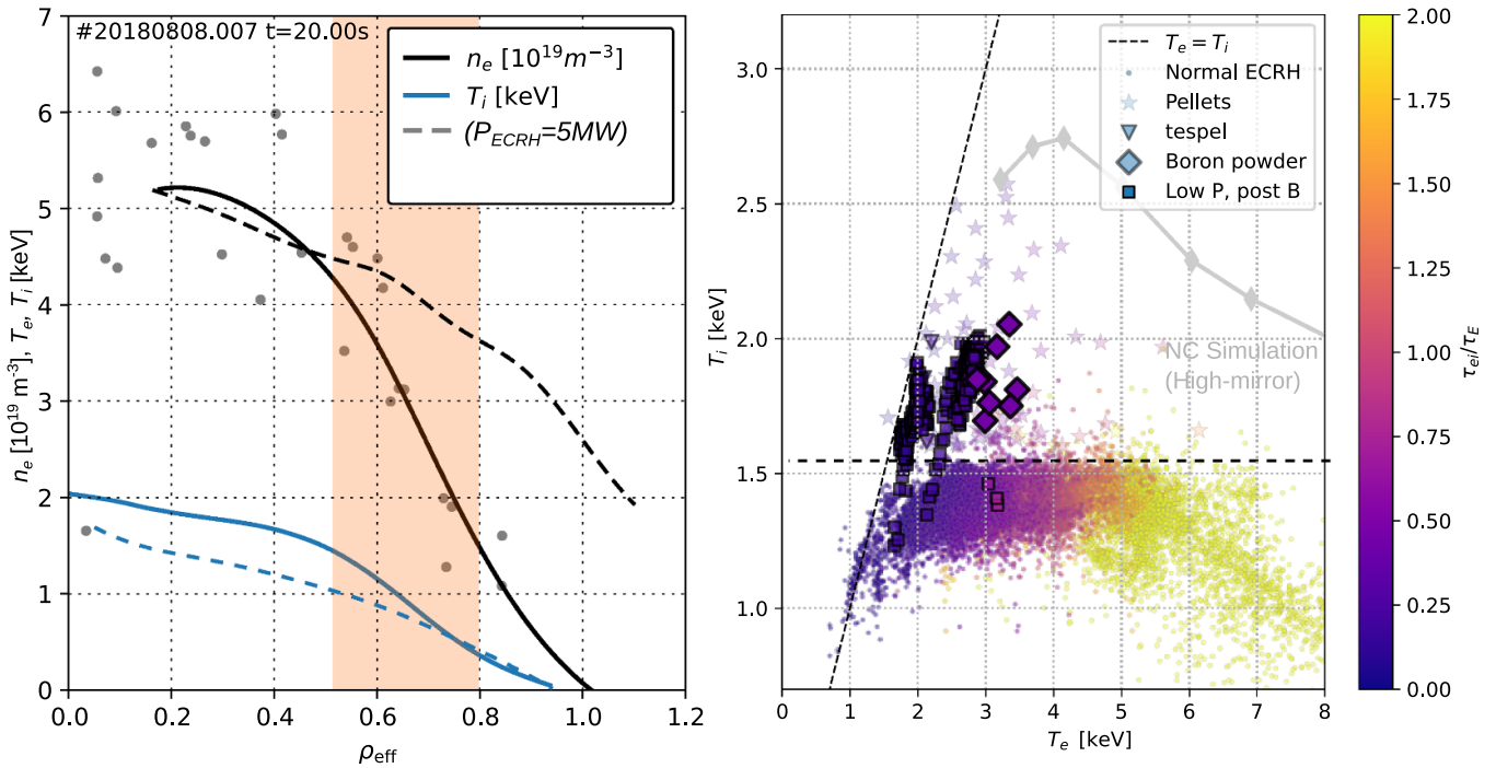
Figure 4. (a) Profiles of electron density (black) and ion temperature (blue) in a low ECRH power discharge after boronisation (solid) compared with similar density high-power discharge (dashed). (b) Scatter plot of core ion vs electron temperature as figure 2(b) including low-power post-boronisation plasmas (squares) and boron dropper experiments [48] (diamonds).
