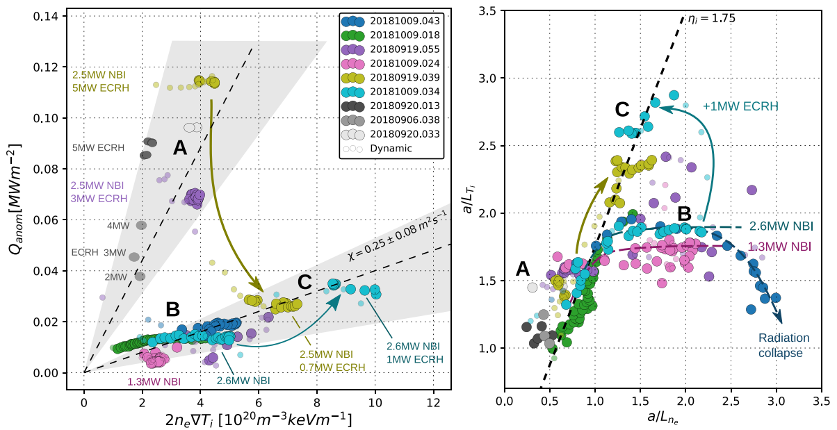
Figure 13. Left: anomalous heat flux versus 2n_e \nabla T_i and right: normalised ion temperature gradient versus electron density gradient for a selection of shots involving mixed heating scenarios. Three groups of plasmas are indicated: (A) High ECRH power ( >2 MW) plasmas with high ion heat flux but low achieved temperature gradients, (B) Pure NBI plasmas with high density gradient and low heat diffusivity but low total heat flux and hence low ion temperature gradient, (C) NBI plasmas with high density gradient and low ( <2 MW) but sufficient ECRH power to achieve higher temperature gradients. Left is shown a line of constant heat diffusivity Q_{\text{anom}} = \chi 2n_e \nabla T_i with \chi \approx 0.25 and right is shown a line of constant \eta_i = L_{T_i} / L_{n_e} .
