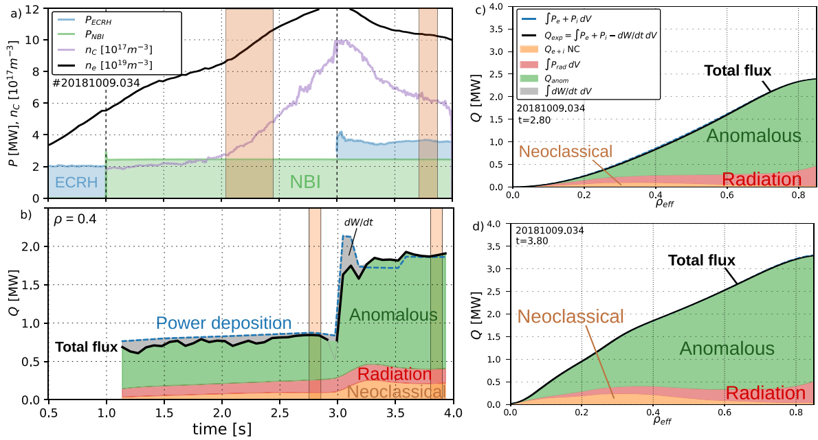
Figure 12. Time trace for \rho = 0.4 (b) and radial profiles at selected time points (c), (d) of energy fluxes during NBI/ECRH mixed heating discharge #20181009.034. Experimental fluxes (black) are calculated by subtracting the rate of stored energy (shaded gray when +ve) from the NBI and ECRH deposited power (blue dashed). The difference between experimental and calculated neoclassical (orange) and measured radiation (red) fluxes is attributed to anomalous transport (green). Power and density traces (a) from figure 6 are repeated for reference. The profiles are time-averaged over the end of the pure-NBI phase (c) and the mixed NBI+O2 ECRH phase with stable performance (d), which are highlighted (orange) in the time trace.
