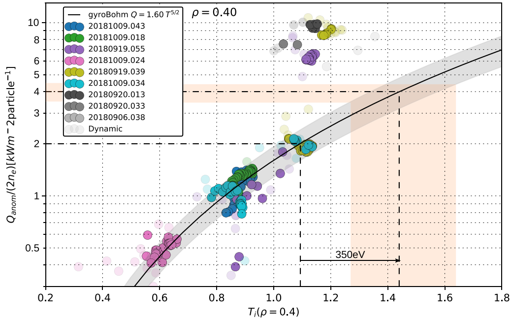
Figure 14. Energy flux per particle versus ion temperature in the steep gradient region for a selection of shots involving mixed heating scenarios. Also plotted is gyro-Bohm scaling Q \propto n_e T^{5/2} with fitted scaling factor and the projection of possible T_i at mid-radius based on a doubling of the NBI and ECRH power compared to the highest T_i discharges measured so far.
