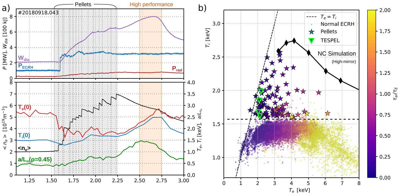
Figure 3. (a) Time traces of main plasma parameters through pellet injection (gray) and high performance (orange) phases. (b) Scatter plot of core ion vs electron temperature for ECRH heated gas-fuelled (small points) and pellet-fuelled (stars) plasmas in the 2018 experiment campaign. The color scale shows the electron-ion equilibration time relative to the energy confinement time. Black diamonds show the expectation from transport simulations [31] assuming only neoclassical heat transport for the high-mirror magnetic configurations.
