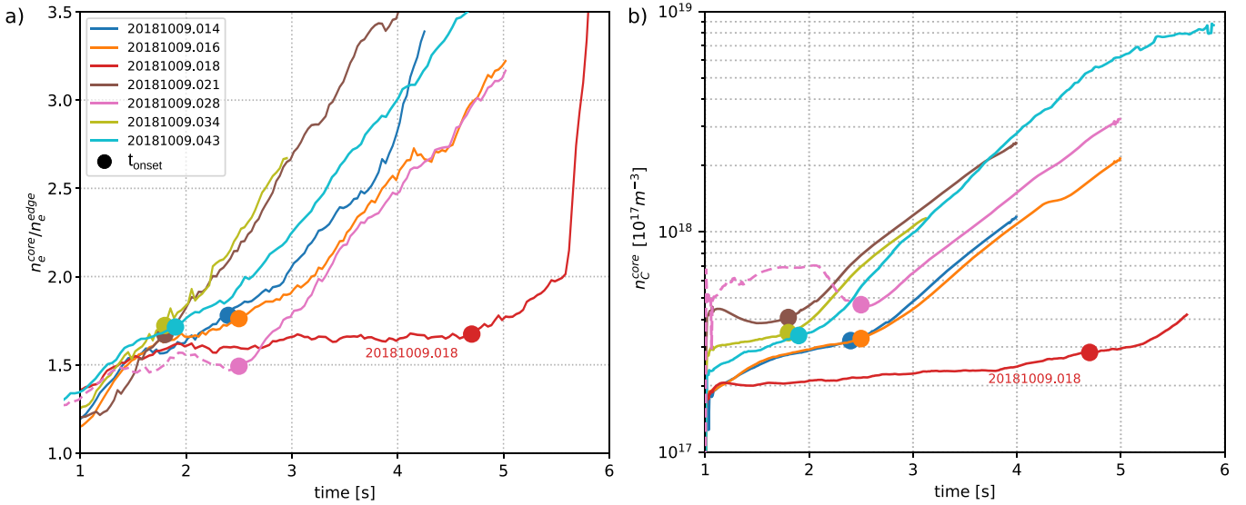
Figure 9. Evolution of electron density peaking factor n_e^{\text{core}}/n_e^{\text{edge}} (a) and core carbon density (b) during all pure NBI discharges. Approximate ‘onset’ times are marked by hand.
