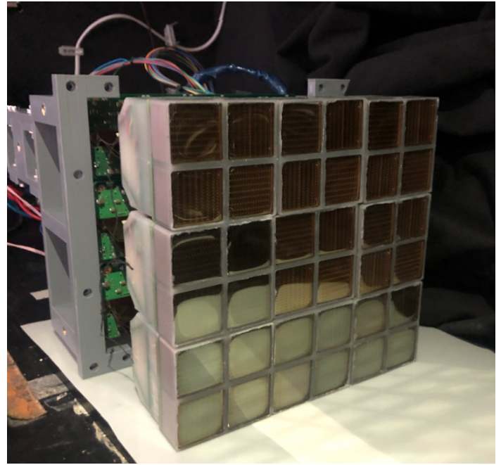
Fig. 2: Photograph of an assembled PDM, of which the FT will consist of three side by side. Four MAPMTs are potted into gelatinous gel to form an EC. These ECs are then connected to a cross-board, the green printed circuit boards in the back. The whole PDM is enclosed in a custom plastic enclosure.
