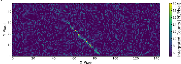
Fig. 7: Photo-electrons (PEs) per pixel integrated over 50 GTUs, shower with Energy E = 3 EeV, zenith angle \theta = 57^\circ , in an ideal location for observation below detector as in Figure 6. Simulated background of 0.1 average counts per pixel per GTU, which is lower than the expected background rate in flight but is useful for illustrative purposes.
