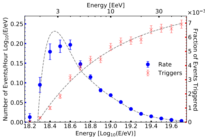
Fig. 8: The fraction of triggered showers per energy bin shown in red, fit to an activation function of the form a(1 - \exp(-(x+b)/c)) . The estimated event rate as a function of shower energy shown in blue, normalized to be differential with respect to \log_{10}(E/\text{eV}) . Error bars shown are Poissonian errors on the number of triggered events. Image taken from (Filippatos et al., 2021).
