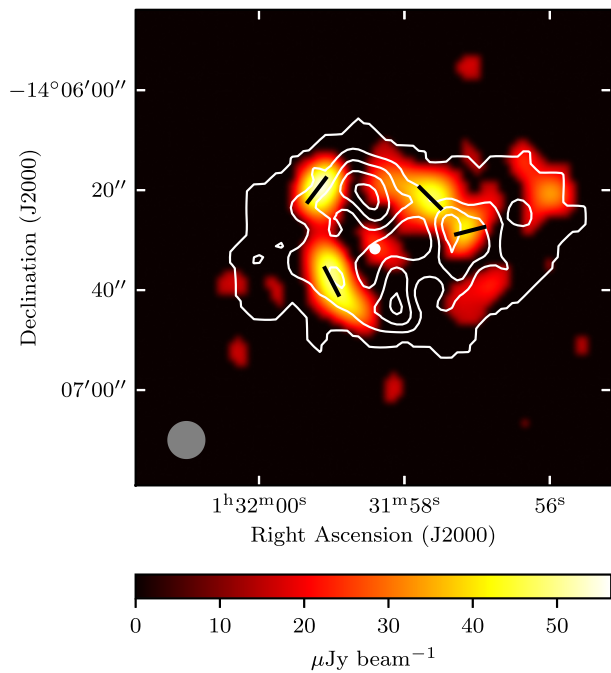
Figure 6. Average bias corrected polarized flux density, over the range 908–1145 MHz in orange and white total intensity contours at (3, 10, 15, 20, 25) × the rms value of 7.3 \mu\text{Jy beam}^{-1} . Black vectors indicate the inferred magnetic field directions at the positions of the four peaks in polarized intensity, after correction for the local RM. The white dot at the centre represents the potential host galaxy and background emission is removed with sigma clipping at a \sim 3\sigma level for the total intensity contours. The synthesized beam (FWHM 7.6 arcsec) is shown in the lower left-hand corner.
