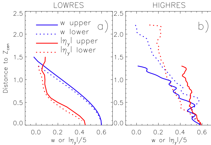
FIG. 9. Vertical profiles of thermal core vertical velocity w (blue lines) and absolute value of vorticity in the y - z plane |\eta_y| (red lines) as a function of distance from thermal's center height Z_{cen} (defined by the height of maximum streamfunction \psi ). (a),(b) Results from single realizations of the LOWRES ensemble at t = 15.2 and the HIGHRES ensemble at t = 15.3 . Solid lines show profiles from Z_{cen} to the thermal bottom ("lower") and dotted lines from Z_{cen} to the thermal top ("upper"). Profiles of w are averaged within 3\Delta x of the thermal's vertical central axis. Profiles of |\eta_y| are averaged over the whole thermal width.
