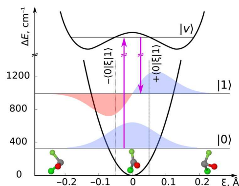
Fig. 1. Creation of a chiral vibrational wave packet in a planar molecule.
