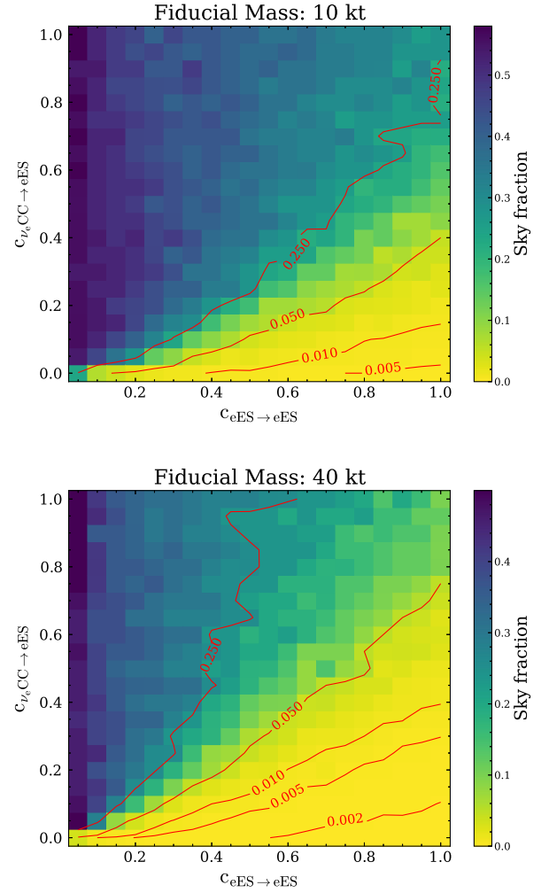
FIG. 14. Burst pointing resolution as a function of eES true positives ( c_{\text{eES} \rightarrow \text{eES}} ) and \nu_e CC false negatives ( c_{\nu_e \text{CC} \rightarrow \text{eES}} ). Results assuming the fiducial mass of a single far detector module (10 kton) and all four planned modules (40 kton) are shown. For each pair of values, 1000 supernova bursts are simulated to determine the pointing resolution. Contour lines for various pointing resolution angles are also shown.
