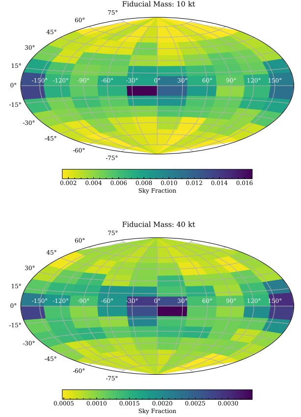
FIG. 16. Burst pointing resolution as a function of the direction of the supernova, given in the detector coordinate system ( \pm \hat{x} is the drift direction, +\hat{z} is approximately the beam direction). \theta (shown vertically) and \phi (shown horizontally) are spherical coordinates in a coordinate system for which \theta = 90^\circ corresponds to the +\hat{z} direction and \theta = 0^\circ , \phi = 0^\circ correspond to the +\hat{x} direction. Pointing resolution is given for the fiducial volumes of 10 and 40 kton. Perfect classification between eES and \nu_e \text{CC} events is assumed in these plots. Note that the local pointing resolution is smeared by the event selection radius of 10 degrees.
