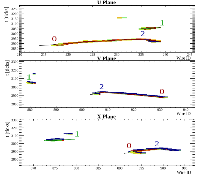
FIG. 4. Example standard DUNE event display of an eES event. The colors show a heat map of the charge deposited on each wire segment per time tick. From top to bottom, the three plots show the view of the three wire planes, U, V, and X respectively, for one APA of the LArTPC. The trajectories with numerical labels are reconstructed tracks, where “0” corresponds to the primary electron track, while “1” and “2” refer to the bremsstrahlung-induced blips.
