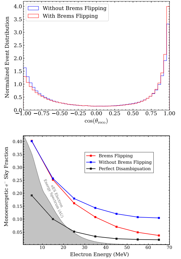
FIG. 7. Effectiveness of the brems-flipping algorithm: The top plot shows the bimodal distribution of the angular difference between true and reconstructed electron directions using the supernova eES electron energy spectrum, centering around the parallel ( \cos \theta = 1 ) and antiparallel ( \cos \theta = -1 ) directions. Brems flipping noticeably decreases the magnitude of the antiparallel peak. The bottom plot shows the relationship between the covered sky fraction and mono-energetic electron energy. The black curve corresponds to a perfect directional disambiguation always resulting the true direction. Brems flipping performs better at higher energies, as there are more secondary tracks to reference. The electron energy spectrum from eES illustrates the energies relevant to supernova pointing.
