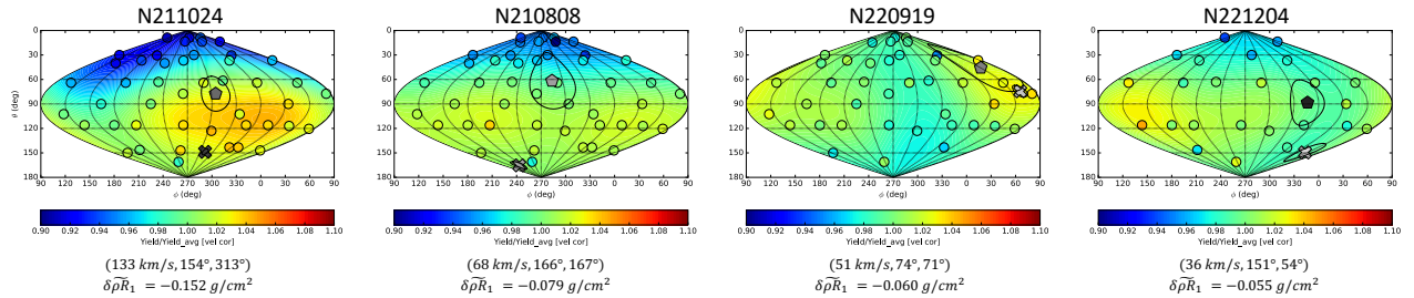
FIG. 2. Progression of \rho R skymaps (L-R) toward robust, ignition platform. Below each subplot is shown the hot spot velocity and maximum difference in yield. On the figures, X = hot spot velocity, pentagon = mode-1 drive, circle = RT-NAD locations.
