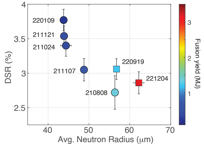
FIG. 4. The 4\pi averaged down scattered ratio (DSR) vs. the average radius of neutron emission for the 1.9 MJ design (circles) and 2.05 MJ design (squares). The color of the datum correspond to the fusion yield of the experiment.
