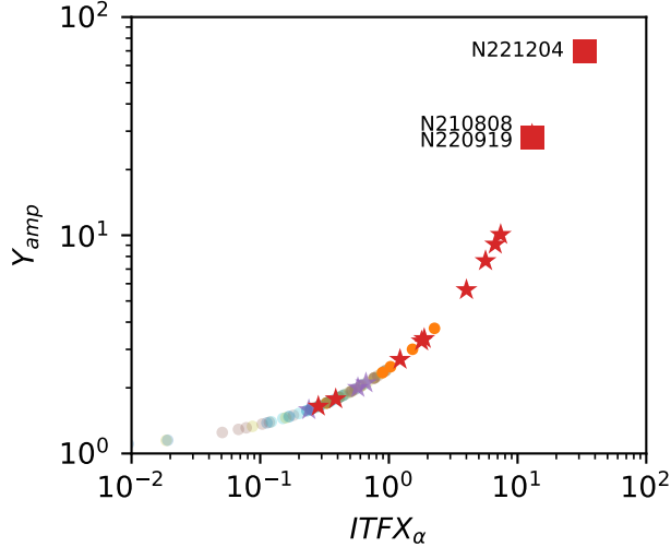
FIG. 8. Inferred yield amplification and ITFX_\alpha for NIF experiments culminating in N221204.
