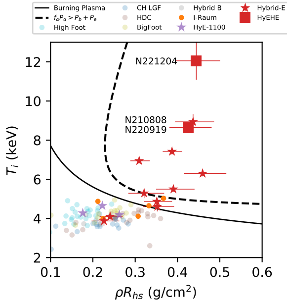
FIG. 7. Hot-spot ion temperature and areal density. Thresholds for the burning-plasma criteria and static self-heating are shown with NIF data.
