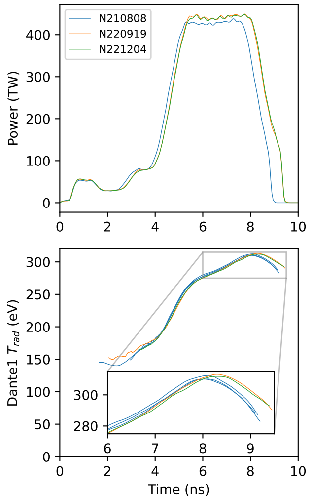
FIG. 1. Top: Laser pulses as delivered for N220919 and N221204 versus N210808. Bottom: Measured radiation temperature ( T_{rad} ) from Dante 1 versus time. Since the Dante 1 data are not available for N210808, data from several shots that repeated the same laser pulse and hohlraum conditions as N210808. These results can be directly compared to the data for N220919 (orange) and N221204 (green). The additional drive at the end of the pulse is clearly manifested by a slightly higher peak T_{rad} . This demonstrates the drive increase when using the additional laser energy. Additional analysis of the hohlraum conditions and radiation temperature are given in Ref. 19.
