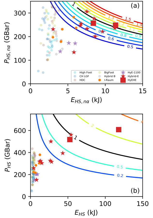
FIG. 9. Inferred hot-spot pressure and energy, inferred without the presence of self-heating (top, a) and directly for the burn-on experiments (bottom, b). Contours of EP^2 relative to N210808 in both cases are shown.
