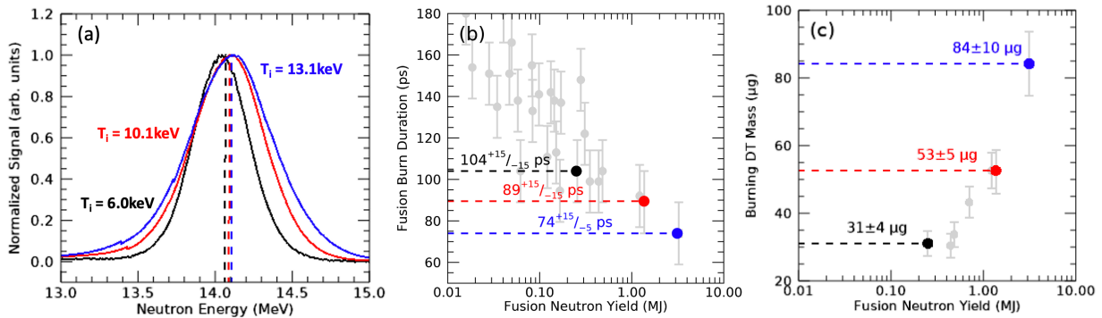
FIG. 5. a) Neutron spectra and apparent DT ion temperature, from 1.9 MJ laser energy experiments N220109 (black) and N210808 (red), and from a 2.05 MJ laser energy experiment N221204 (blue). b) Neutron emission duration as fusion yield. c) Inferred hot spot mass for 1.9 and 2.05 MJ laser experiments. In b) and c) experiments N220109 (black), N210808 (red), and N221204 (red) have been highlighted.
