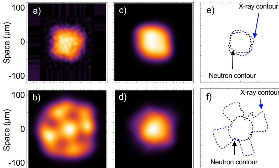
FIG. 6. X-ray and neutron emission measurements from N210808 (top row) and N221204 (bottom row). Time integrated x-ray emission ( > 10 keV) from N210808, a), and from N221204, b). Time integrated neutron emission from N210808 c) and from N221204, d). Comparison of contours that enclosed 50% of the x-ray and neutron emission for N210808 e), and for N221204, f).
