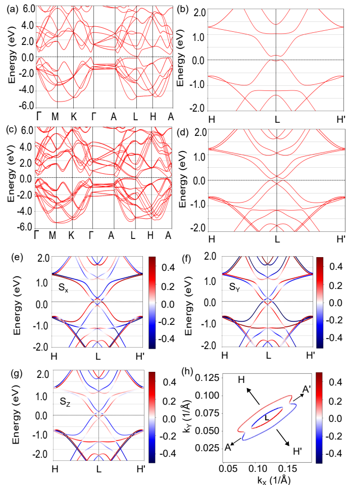
FIG. 3. Electronic band structure of bulk BiAs without SOC (a) along all the main high symmetry directions and (b) focusing on the H-L-H' direction of the hexagonal Brillouin zone. The corresponding band structures with SOC are shown (c) and (d). Spin-resolved band structure for (e) ( S_x ), (f) ( S_y ), and (g) ( S_z ) projections. (h) Spin texture around the L point of the Brillouin zone at 0.2 eV above the Fermi level.
