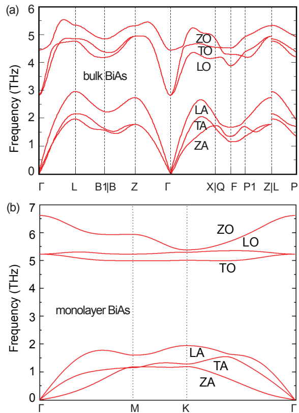
FIG. 2. Calculated phonon dispersion along the high symmetry lines for (a) the rhombohedral R\bar{3}m structure of the bulk BiAs and (b) monolayer BiAs.
