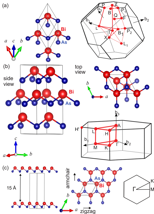
FIG. 1. Layered crystal structure of bulk BiAs, space group R\bar{3}m , represented by (a) a rhombohedral primitive cell containing two atoms and (b) a conventional hexagonal unit cell containing six atoms (side and top views). (c) Supercell used in the calculations of the monolayer BiAs (side and top views), with armchair and zigzag directions indicated. The corresponding Brillouin zones with high symmetry points and directions are also shown on the right side.
