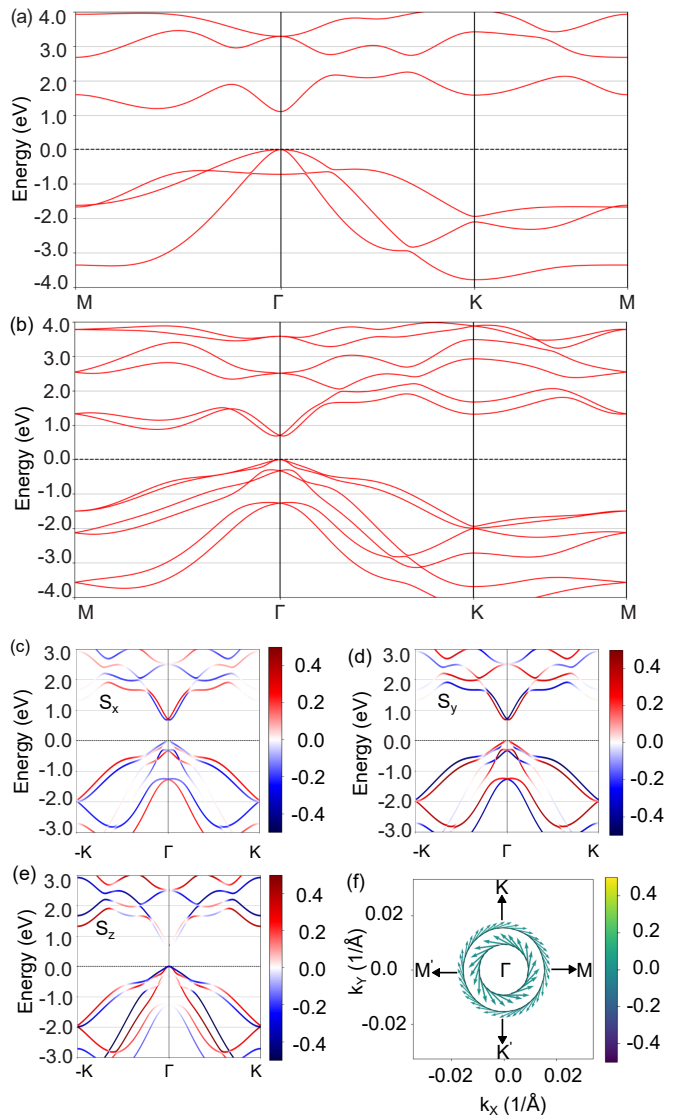
FIG. 4. Electronic band structure of monolayer BiAs along the M- \Gamma -K-M directions (a,b) without SOC and with SOC. Spin-resolved band structure for (c) ( S_x ), (d) ( S_y ), and (e) ( S_z ) projections. (f) Spin texture around the \Gamma point of the Brillouin zone at 0.75 eV above Fermi level.
