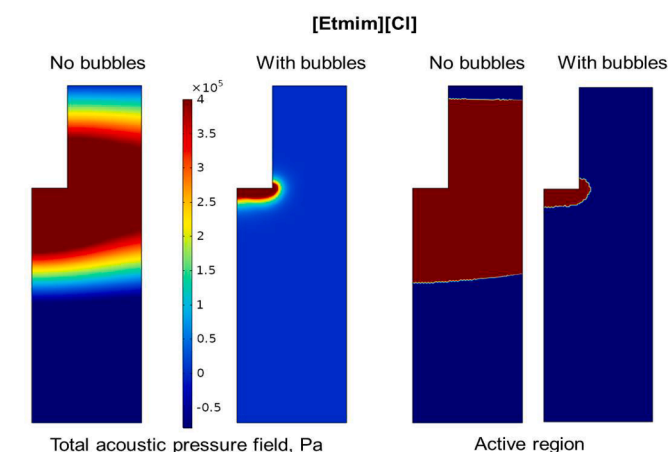
Fig. 3. Profiles of acoustic pressure field and active volume regions for [Etmim][Cl] at 60 W and d = 2 cm. Comparison between simulations with (profiles on the right) and without (profiles on the left) acoustic attenuation elicited by cavitation bubbles. For [Etmim][Cl], the volumes of the active regions differ by 193 %.
