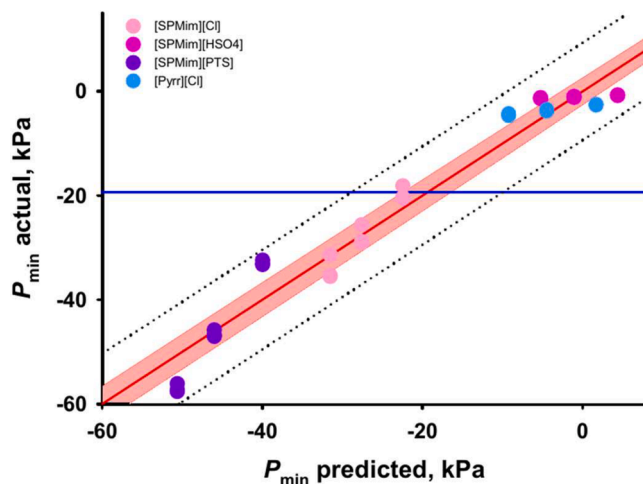
Fig. 5. Actual by Predicted plot of P_{\min} for ILs with \mu \geq 1 Pa s. ■ Regression, ■ 95 % CI of prediction, RMSE = 4294, R^2 = 0.955 , p -value < 0.0001 , ■ Mean of response (-19.34 kPa), • • • Prediction interval.
