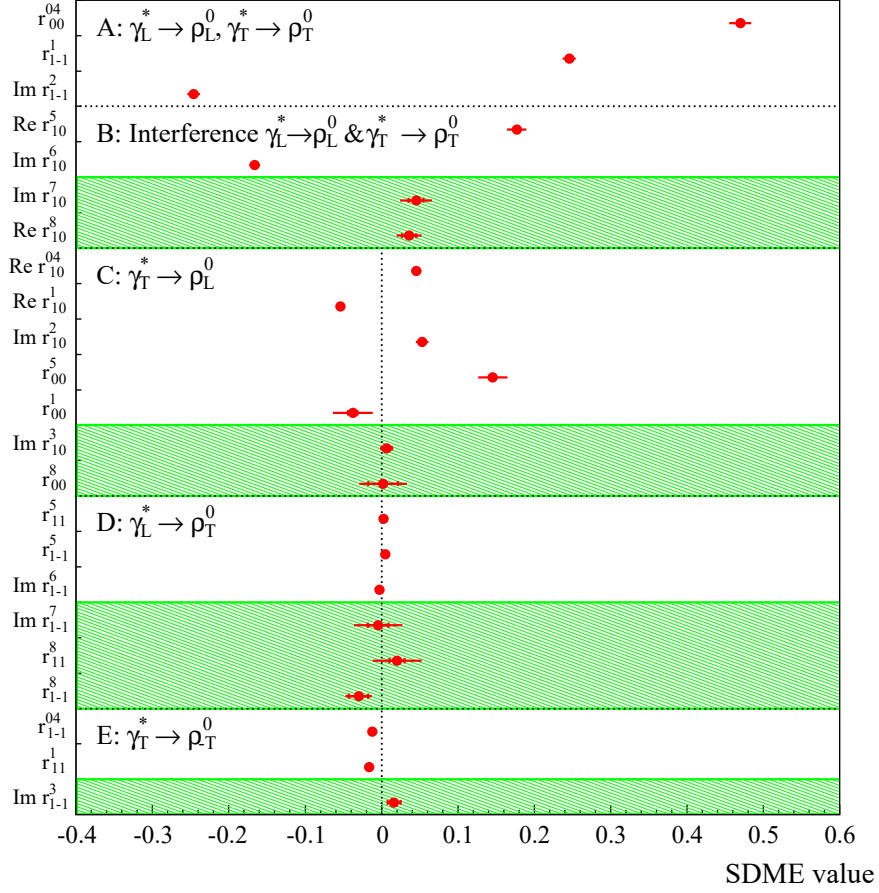
Fig. 4: The 23 SDMEs for exclusive \rho^0 lepton production extracted in the entire COMPASS kinematic region with \langle Q^2 \rangle = 2.40 \text{ (GeV}/c^2\text{)} , \langle W \rangle = 9.9 \text{ GeV}/c^2 , \langle p_T^2 \rangle = 0.18 \text{ (GeV}/c\text{)}^2 . Inner error bars represent statistical uncertainties and outer ones statistical and systematic uncertainties added in quadrature. Unpolarised (polarised) SDMEs are displayed in unshaded (shaded) areas.
