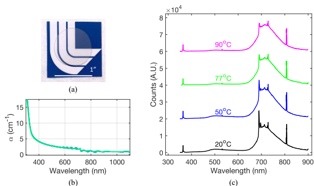
Fig. 1. (a) Optical image of the 1" Fe- \beta Ga 2 O 3 wafer, and (b) spectrophotometer measurement of the absorption coefficient from UV to IR, and (c) photoluminescence (PL) spectrum of the sample with a 355 nm optical source over from room temperature to 90°C.
