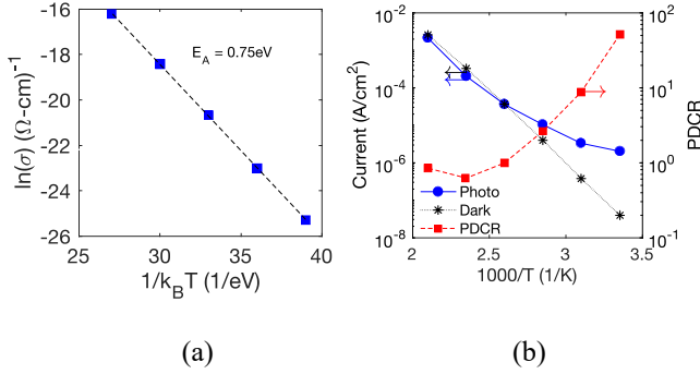
Fig. 5. Temperature characterization of the Fe- \beta Ga 2 O 3 PCSS. (a) Logarithmic plot with respect to temperature to extract activation energy of the sample. (b) Photo and dark current and PDCR with respect to temperature at 200V bias.
