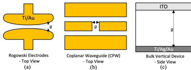
Fig. 2. Electrical test structures fabrication, including (a) Rogowski electrodes for high field measurements designed for electrode gap g . (b) coplanar waveguide structure with signal trace gap g used for lifetime measurements, and (c) vertical structure used for PCSS responsivity characterization.
