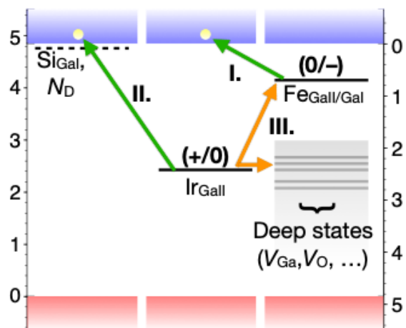
Fig. 7. Proposed trap model with active impurities in our sample. Green arrows correspond to carrier generation and yellow arrows correspond to internal transitions.
