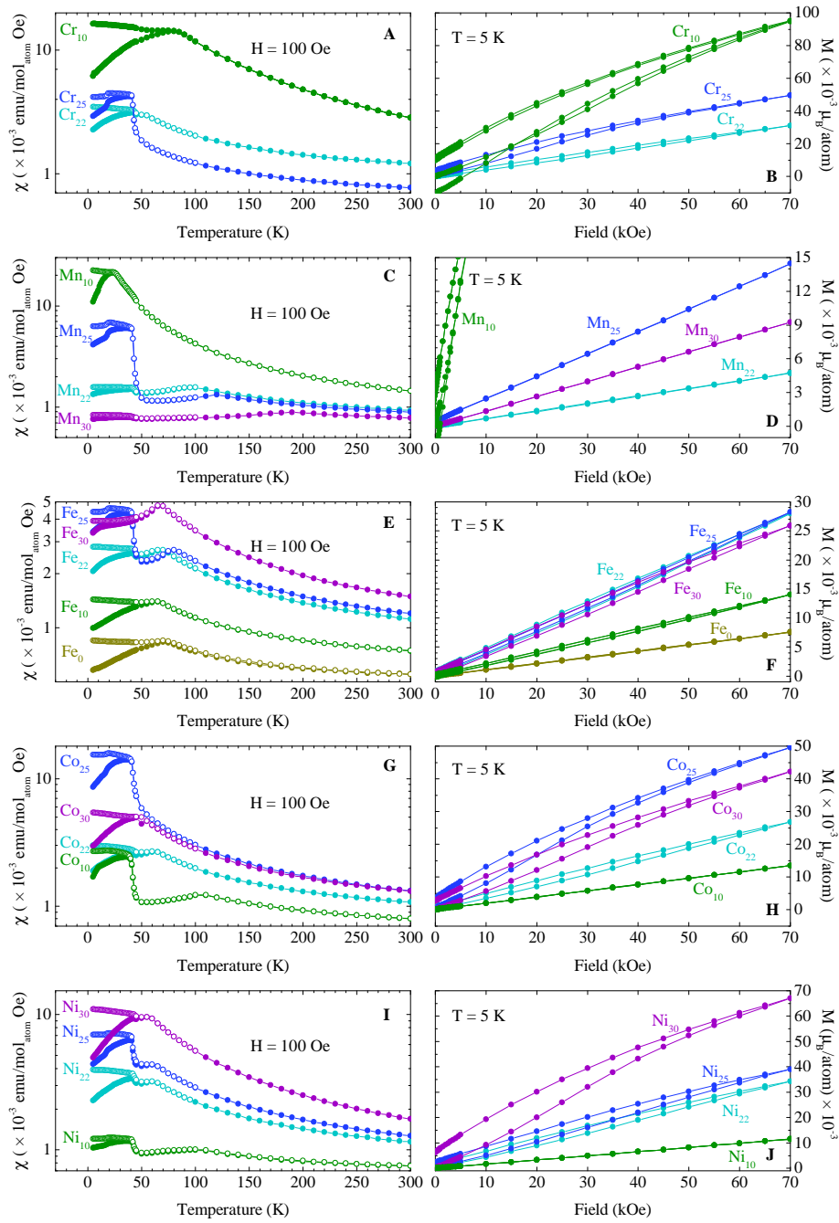
FIG. 1. Susceptibility and magnetization data for Cantor alloys of varying compositions. Panels on the left show susceptibility versus temperature on a logarithmic scale, while those on the right show magnetization as a function of magnetic field. In the susceptibility plots, solid circles represent zero-field cooled (ZFC) data, which were measured after cooling down in zero field. Open circles represent field-cooled warming (FCW) data, which were collected after cooling down in an applied field of 70 kOe. Each row displays a different set of compounds: (A)-(B) Cr-varied compositions, (C)-(D) Mn-varied compositions, (E)-(F) Fe-varied compositions, (G)-(H) Co-varied compositions, and (I)-(J) Ni-varied compositions. Section II B describes the sample nomenclature. Certain curves such as \text{Mn}_{10} and \text{Fe}_{30} display only one feature. In these cases, the feature is identified as T_1 or T_2 depending on its shape, with T_1 being step-like and T_2 being a peak.
