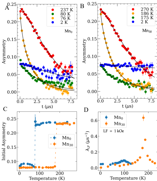
FIG. 3. (A, B) Representative zero-field \mu SR asymmetry spectra for \text{Mn}_0 and \text{Mn}_{30} , respectively. (C) Temperature dependence of the initial asymmetry at t = 0 for both samples, showing a sharp step at the expected transition temperatures. (D) Temperature dependence of the long-time relaxation rate \lambda_{\text{LF}} in an applied longitudinal field of 1 kOe.
