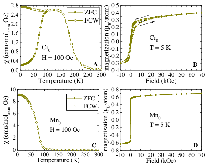
FIG. 2. Magnetic susceptibility as a function of temperature for the (A) \text{Cr}_0 and (C) \text{Mn}_0 samples. Magnetization as a function of applied field for the (B) \text{Cr}_0 and (D) \text{Mn}_0 samples. Magnetization data for \text{Cr}_0 show significant hysteresis, and arrows in panel (B) indicate the direction of the magnetic field sweep for each curve segment. In panel (C), ZFC and FCW curves are difficult to distinguish due to significant overlap, with less than 1% of difference across the entire data range.
