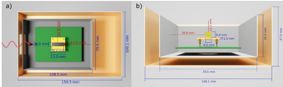
Fig. 3: a) Top and b) front view of the detector and our L-TCT setup. The dimensions used for calculation of the electric and weighting fields are shown. Here: Detector – grey (top view) and gold (front view), Sample holder – yellow, Conductive pads and pins – golden, readout PCB – green, and double ferromagnetic shielding – grey and orange. The dimensions displayed in red show the distance from the detector to the shielding.
