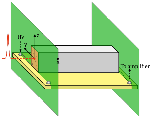
Fig. 1: Schematic of the experimental setup and illumination conditions. The additional electrodes used for making the uniform electric field are shown in green.
