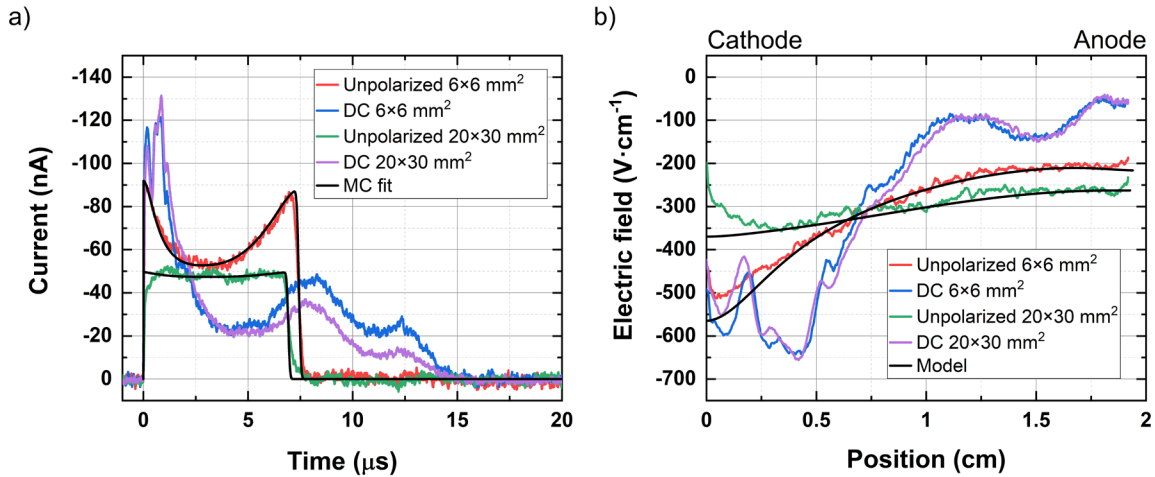
Fig. 8: a) Comparison of electron current waveforms with and without additional 20 mm \times 30 mm electrodes in an unpolarized and DC regime at 600 V. b) The electric field evaluated from the current waveforms in a).
