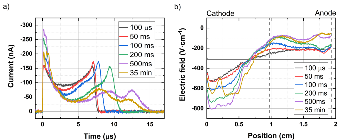
Fig. 5: a) Changes of electron current transients after -600 V biasing. b) The electric field evaluated from the current waveforms in a). The solid horizontal line represents the electric field in the planar sample. The dashed vertical lines mark the middle (0.97 cm) and anode (1.94 cm) positions of the detector.
