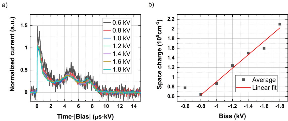
Fig. 6: a) Normalized electron waveforms obtained in the steady-state regime, measured 5 min after DC biasing. b) Dependence of the average space-charge density on the applied bias. The charge density was determined using the 1D Gauss law from the electric field.
