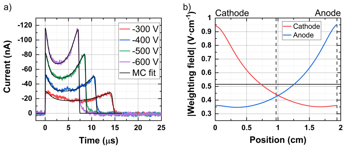
Fig. 4: a) Bias dependence of selected electron current waveforms in an unpolarized sample and fits using Monte Carlo simulations. b) Comparison of the absolute value of the weighting fields for the detector's cathode (positive) and anode (negative) for the bar detector in ferromagnetic shielding. The weighting fields are evaluated along the electric field line starting in the center of the cathode ( x=0 mm, y=0 mm, z=0 mm). The dashed lines show the position of the anode at 1.94 cm and the middle of the sample at 0.97 cm. The solid horizontal line represents the weighting field of a planar detector with the same thickness.
