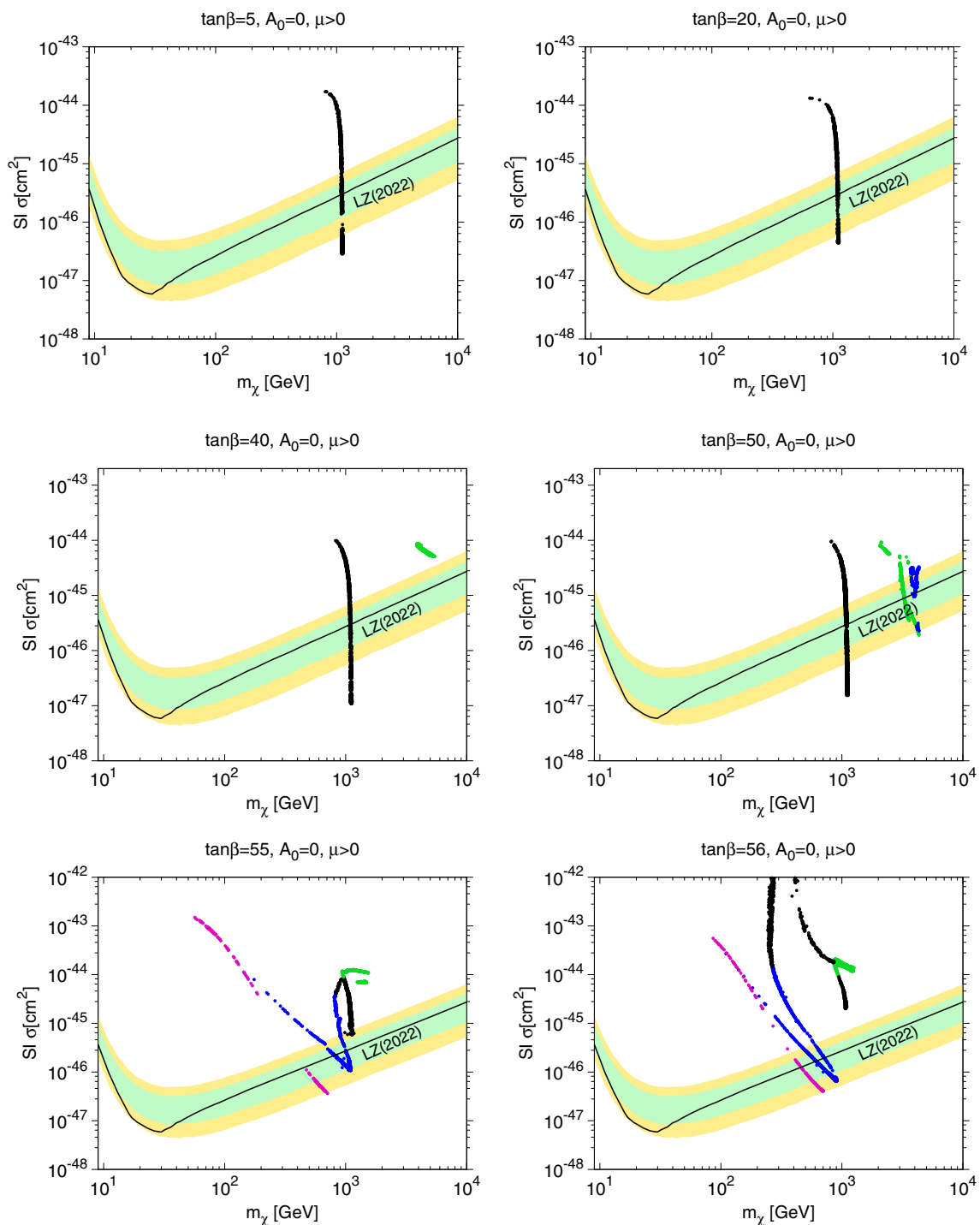
Fig. 9 Calculations of spin-independent WIMP-nucleon scattering for points along the dark matter strips for \tan \beta = 5, 20, 40, 50, 55 and 56 with A_0 = 0 and \mu > 0 compared with the LUX-ZEPLIN upper limit (solid black line). The green and yellow bands are the 1\sigma and 2\sigma LZ sensitivities
