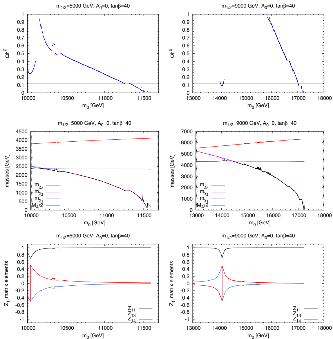
Fig. 2 Cuts across the (m_{1/2}, m_0) planes for \tan\beta = 40 , A_0 = 0 and \mu > 0 for varying m_0 and fixed m_{1/2} = 5.0 TeV (left panels) and 9.0 TeV (right panels), showing the dark matter density (top panels), particle masses (middle panels) and the composition of the bino-like neutralino (bottom panels)
