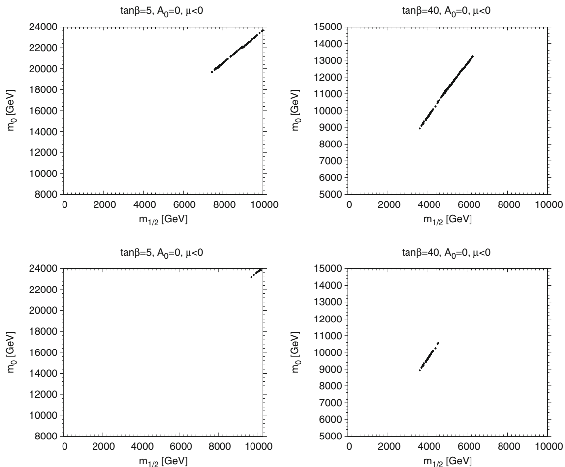
Fig. 20 The portions of the dark matter strips for \tan \beta = 5 and 40 , calculated assuming A_0 = 0 and \mu < 0 , that are allowed by all the constraints, assuming an uncertainty of 1.5 ( 0.5 ) GeV in the calculation of m_h in the upper (lower) pair of panels
