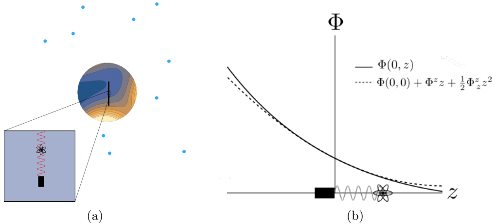
FIG. 2. a) Contour plot in two dimensions of the gravitational potential sourced by particles outside the cutoff radius r_{\min} . b) Comparison of the actual potential and the second order multipole approximation to it near the origin along the one dimensional slice shown in part a).
