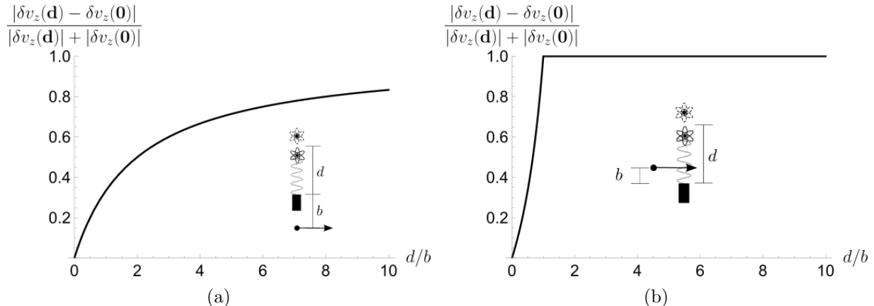
FIG. 3. Plot of the magnitude of the dominant phase shift in Eqn. 70 divided by the sum of the constituent phase shift magnitudes. For d \ll b there is significant phase shift cancellation due to similar common motion of the laser and the atom. a) A bath particle passes below the laser. The size of the net phase shift is about 80% of the sum of the separate phase shift magnitudes for d = 10b , the ratio asymptotes to 1 in the limit d/b \rightarrow \infty . Increasing d far beyond b gives diminishing returns. b) A bath particle passes above the laser. The behavior resembles the previous case for d/b \ll 1 , but as soon as d > b , the momentum kicks on the atom and laser are in opposite directions, so there is no common motion cancellation to the dominant phase shift.
