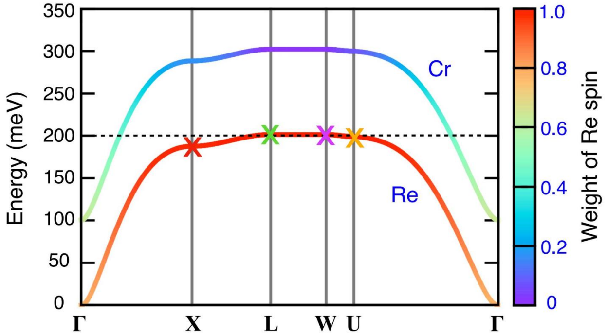
Figure 6: Magnon band structure. Two lowest, non-degenerate magnon bands. Color scale indicates the weight of Re spin involved in the magnon mode. Exchange parameters are obtained from the DFT and spin-wave calculation. The X markers represent the experimentally measured k-points and their energies.
