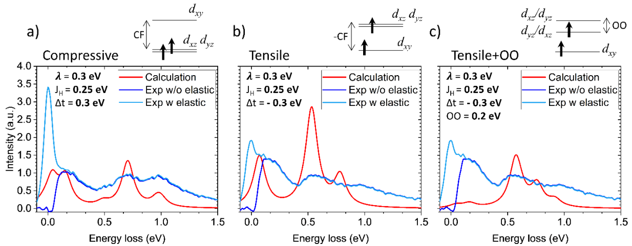
Figure 4: RIXS calculations and experimental data for (a) compressive and (b)-(c) tensile strained SCRO at T=17 K. A large set of input parameters, 0.2 \leq \lambda \leq 0.4 eV, -0.4 \leq \Delta_t \leq 0.4 eV, 0 \leq \text{OO} \leq 0.2 eV, and U=0, 2 eV, are used to match the experimental data. The best set is found to be U=2 , \lambda = \Delta_t = 0.3 eV and J_H=0.25 eV, although the quality of the fit is poor, especially for the excitation at 0.2 eV for tensile SCRO. The agreement between experiment and calculation is not improved with OO as shown in (c).
