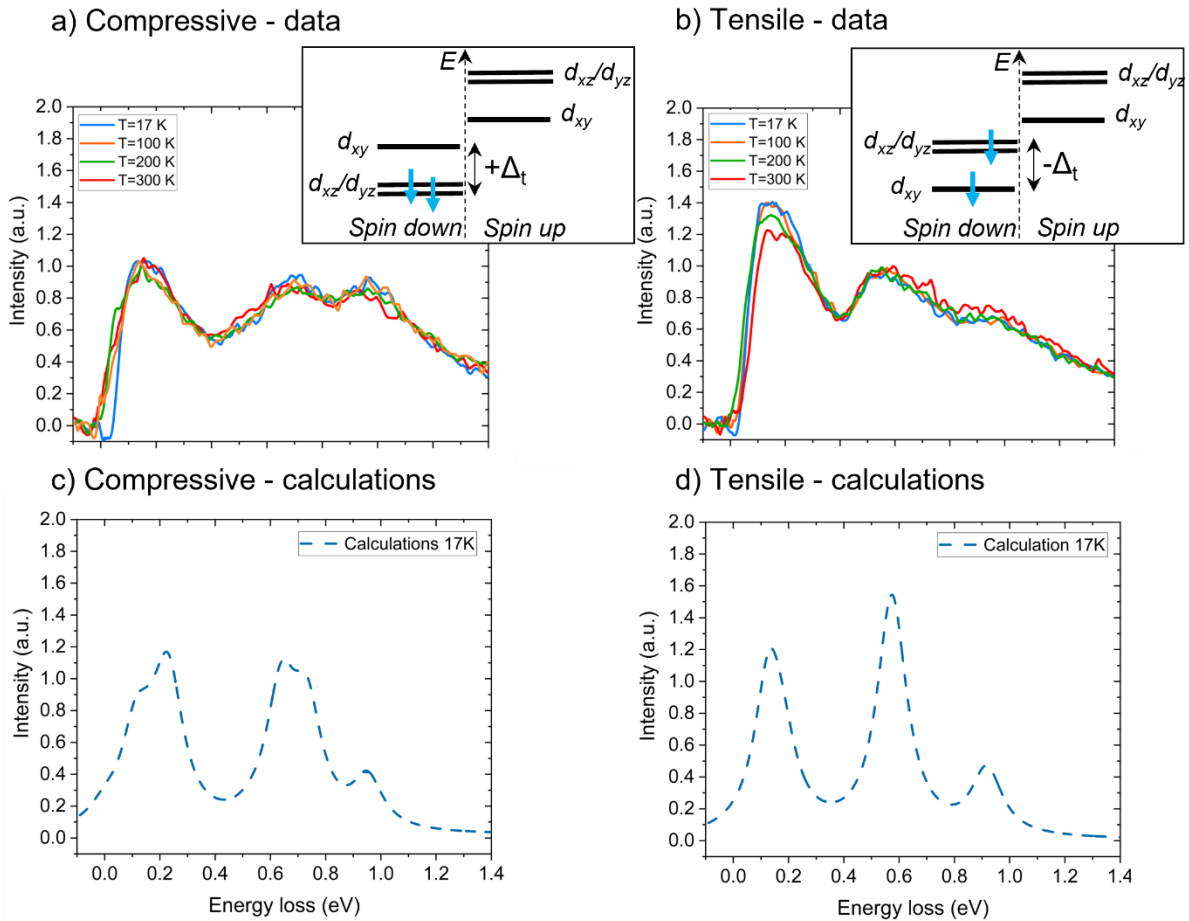
Figure 3: RIXS spectra collected at different temperature for a) compressive SCRO film at q=(6.4, 0.34, 6.8) and b) tensile SCRO film at q=(6, 0.34, 7.2) in the 17-300 K range. The elastic line at 0 eV has been removed for a better reading of the low energy excitations in the experimental data, and the spectra are normalized by the integrated intensity between 0.05 and 1.4 eV. c) and
