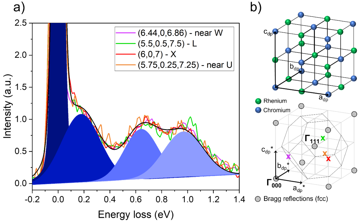
Figure 2: RIXS spectra for different momentum transfer. a) Low-energy RIXS spectra (zone I in the map of Figure 1) collected from the compressive SCRO thin film for different momentum transfer q expressed in the double perovskite cubic system ( dp ), at a temperature of 17 K. The spectra are normalized by the integrated intensity between 0.05 and 1.4 eV. Three excitations are resolved at 0.2, 0.65 and 1 eV, in addition to the elastic line at 0 eV. The black curve represents the sum of four Voigt functions that are used to fit the experimental data collected at the X point. b) Schematic unit cell of the fcc-SCRO in real space, and the corresponding reciprocal space and Brillouin zone. The X marks represent the momenta that have been probed, with the same color code used for the spectrum.
