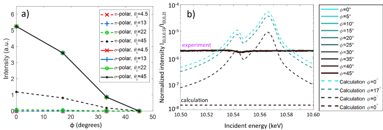
Figure 5: Experimental and calculated energy scans at q=(0\ 0\ \frac{1}{2}) for the OO-induced reflections in tensile SCRO. a) Calculated intensity of the OO-induced reflection at (0\ 0\ \frac{1}{2}) and an incident energy E_i=10.565 keV, as a function of the azimuthal angle \phi , for different incident angle \theta_i and for \pi , \sigma polarization. b) Experimental (solid lines) and calculated (dashed lines) energy-dependent intensity of the OO-induced reflection for \sigma polarization, \theta_i=8.5 degrees and for different \phi values. The simulation is calculated from the absorption spectra resulting from the EDRIXS calculation with OO for the tensile SCRO. The data are corrected for self-absorption and normalized by the Bragg reflection intensity at q=(0\ 0\ 2) .
