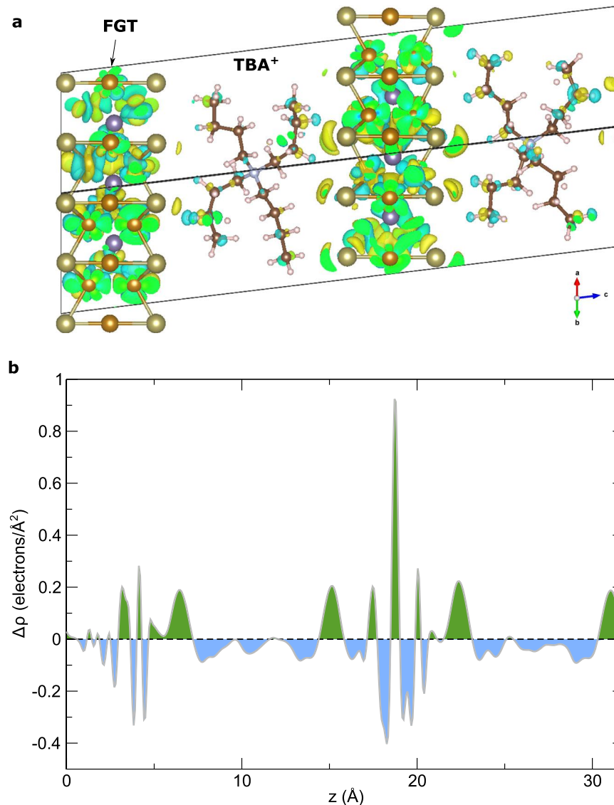
Fig. 3 Theoretical simulations of the charge density difference in intercalated FGT. a, b Charge density difference ( \Delta\rho = \rho(\text{FGT} + \text{TBA}) - \rho(\text{FGT}) - \rho(\text{TBA}) , where \rho(\text{FGT} + \text{TBA}) is the total charge density of FGT plus TBA, \rho(\text{FGT}) is the charge density of the isolated FGT system, and \rho(\text{TBA}) is the charge density of the TBA molecules) through iso-surface and planar average along the z direction, respectively. In a , green and blue iso-surfaces correspond to positive and negative charge, respectively.
