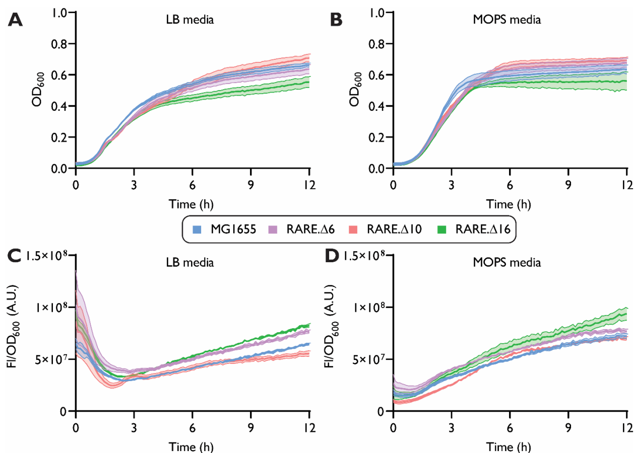
Figure 4. Growth and protein production performance of engineered TPAL retaining strains. Growth was monitored via optical density at 600 nm (OD 600 ) in 96-well plate for 12 h in LB media (A) and in MOPS EZ Rich media (B). Plasmid-based protein overexpression of superfolder green fluorescent protein (sfGFP) was monitored via 96-well plate in a plate reader for 12 h by measuring fluorescence (ex: 488 nm, em: 525 nm) normalized by OD 600 in both LB media (C) and MOPS EZ Rich media (D) (A.U. indicates arbitrary units). Data represents technical triplicates (n=3) where error bars represent the standard deviation across triplicates.
