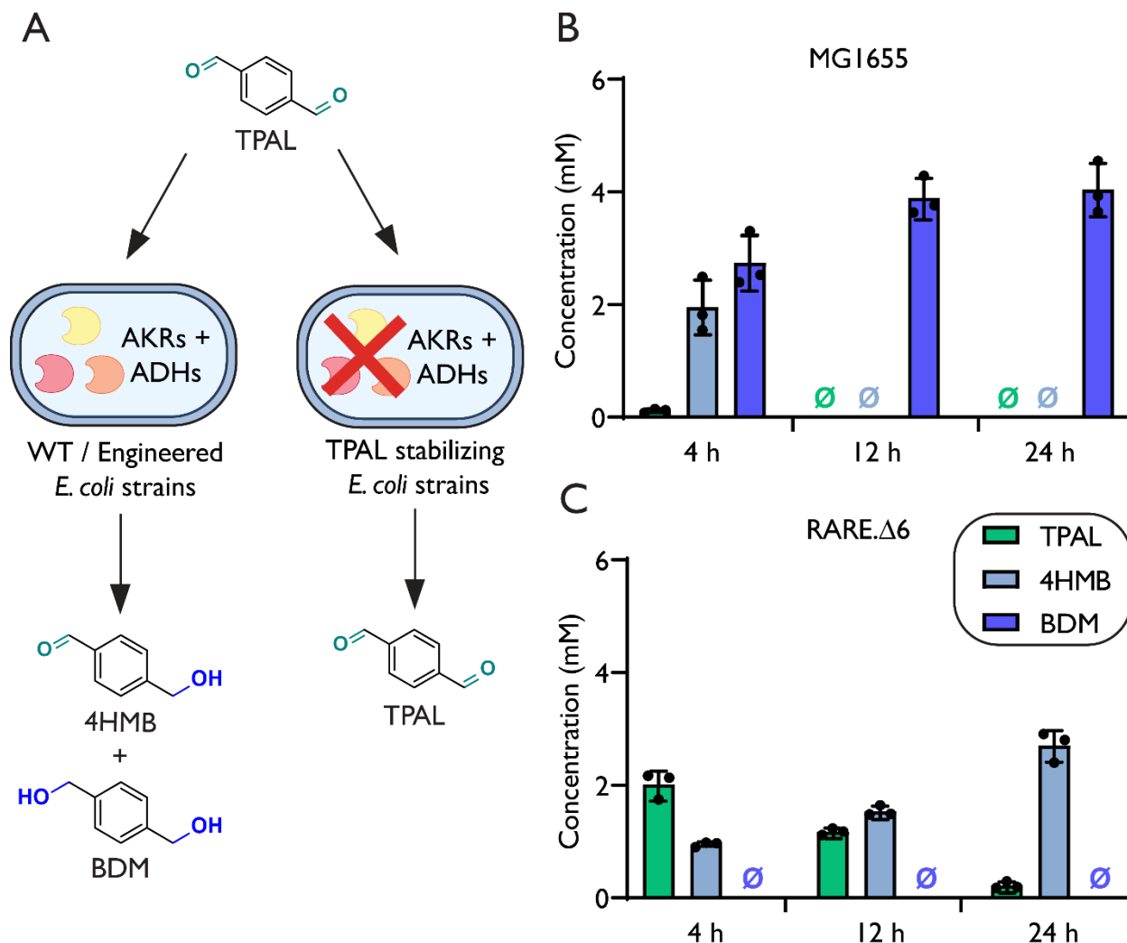
471 472 Figure 1. Evaluation of the stability of TPAL when supplemented to aerobic cultures of E. 473 coli . (A) TPAL was added to culture media to determine its fate in the presence of growing E. coli 474 cells over time. (B) Cultures of wild-type E. coli MG1655 were grown in LB media at 37°C and 475 supplemented with 5 mM TPAL at mid-exponential phase. TPAL metabolites were tracked via 476 HPLC at 4 h, 12 h and 24 h. (C) Cultures of the previously reported E. coli RARE.Δ6 strain were 477 grown under identical conditions and TPAL metabolites were tracked via HPLC at 4 h, 12 h and
