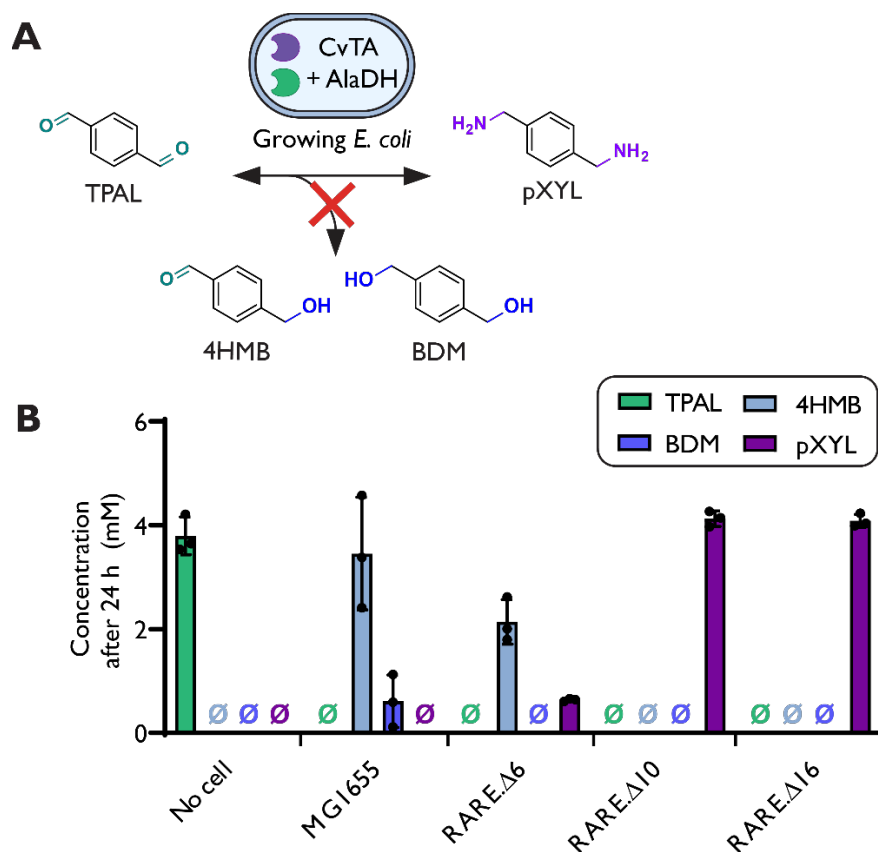
Figure 5. Biosynthesis of pXYL in engineered strains expressing CvTA. (A) We created E. coli strains containing CvTA and AlaDH that can convert TPAL to pXYL without additional reduction of TPAL. (B) Cultures of MG1655, RARE.Δ6, RARE.Δ10, and RARE.Δ16 expressing CvTA were grown in LB media at 37°C and were supplemented with 10 mM L-alanine (amino donor) and 5 mM of TPAL at mid-exponential phase. TPAL, 4HMB, and pXYL concentrations were tracked via HPLC at 24 h. Data represents technical triplicates (n=3) where error bars represent the standard deviation across triplicates. Null sign indicates no detectable quantities were observed.
