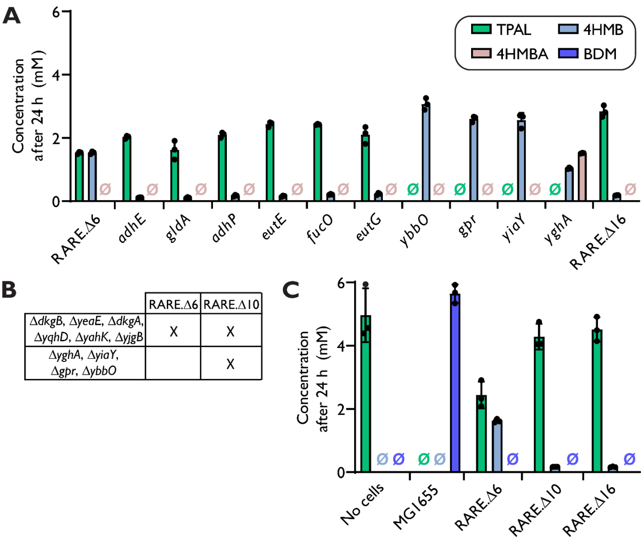
Figure 3. Evaluation of overexpressed ALR activity on TPAL stability. (A) Cultures of RARE.Δ6, RARE.Δ10 and RARE.Δ16 transformed with a single plasmid for each individual ALR gene from this study were grown in LB media at 37°C and supplemented with 5 mM TPAL and then induced of targeted gene at mid-exponential phase and tracked via HPLC after 24 h (4HMBA indicates 4-hydroxymethyl benzoic acid). (B) Gene knockouts contained within RARE.Δ10 strain. Using the E. coli RARE.Δ6 strain as a basis, MAGE was performed to translationally knockout the 4 ALRs that showed reduction of TPAL when overexpressed to generate the RARE.Δ10 strain
