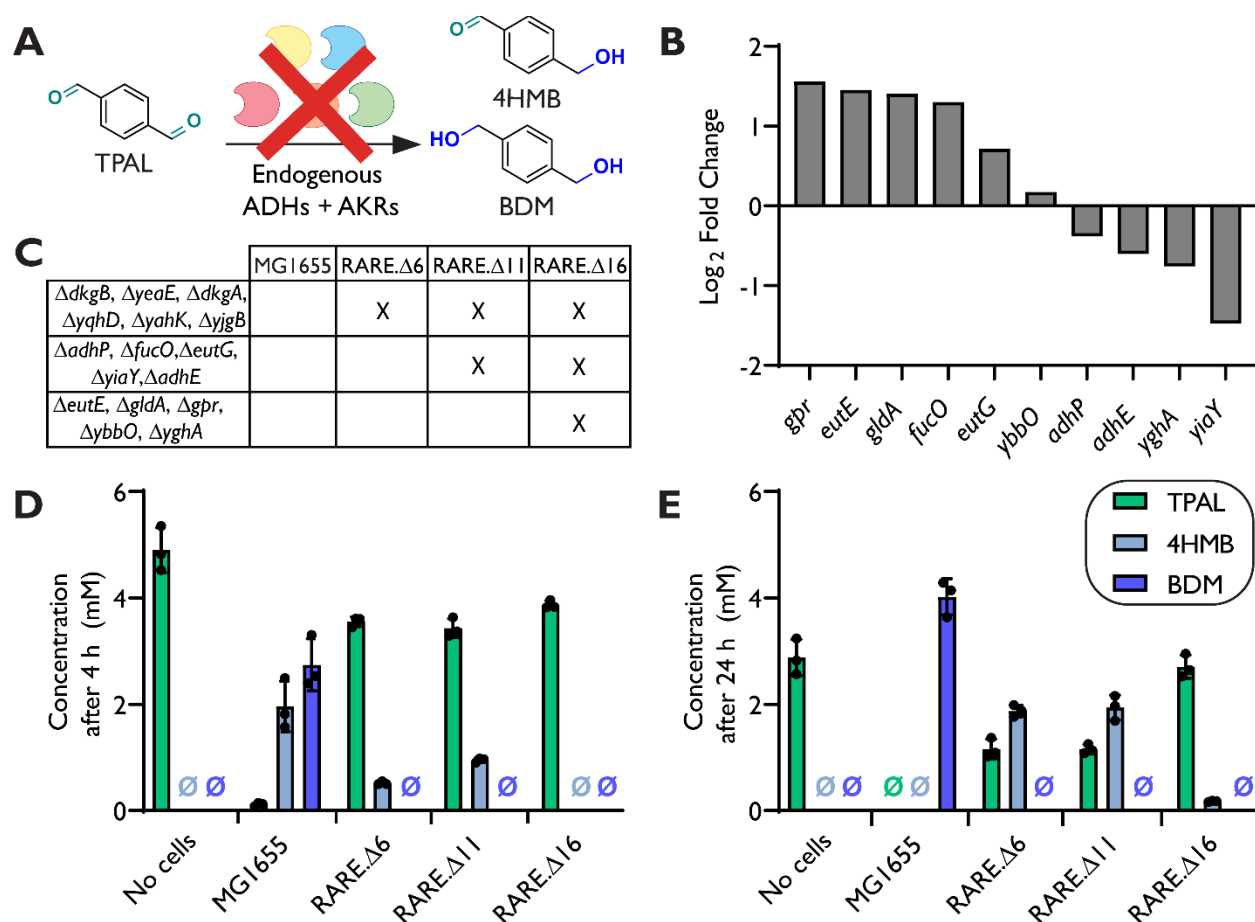
Figure 2. Genomic knockout of aldehyde reductases (ALR) toward improved TPAL stability in aerobic conditions. (A) Using the E. coli RARE.Δ6 strain as a basis, MAGE was performed to translationally knockout ADHs and AKRs to generate two strains RARE.Δ11 (RARE.Δ6, ΔadhP ΔfucO ΔeutG ΔyiaY ΔadhE) and RARE.Δ16 (RARE.Δ11, ΔeutE ΔgldA, Δgpr ΔybbO ΔyghA). (B) Log 2 fold change of targeted genes were determined through a TPAL challenge RNA-seq. Data represents TPAL supplementation in RARE.Δ6 compared to a RARE.Δ6 baseline in technical duplicates (n=2). (C) Gene knockouts contained within each strain. (D&E) Cultures of wild-type E. coli MG1655, RARE.Δ6, RARE.Δ11 and RARE.Δ16 were grown in LB media at 37°C and supplemented with 5 mM TPAL at mid-exponential phase. TPAL metabolites were tracked via
