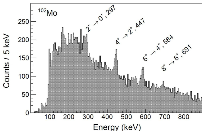
FIG. 6: Doppler-corrected \gamma -ray singles spectrum obtained for the fission fragment ^{102}\text{Mo} identified in the high-rigidity setting. Data are restricted to GRETINA detectors located at 90^\circ relative to the beam direction. An additional condition has been imposed upon the interaction depth of the \gamma rays in each HPGe crystal in order to suppress x rays.
