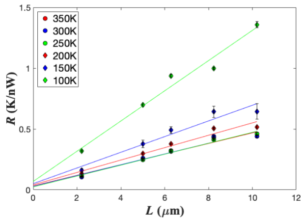
Figure 4. Measured thermal resistances ( R_j ) of the suspended segments of MWCNT sample 1 as a function of the suspended segment length at different temperatures specified in the legend.
