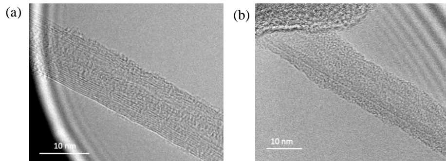
Figure 6. TEM images of sample 10 before (a) and after (b) metal evaporation through a shadow mask onto the four contact areas between the MWCNT and the thermometer lines.
