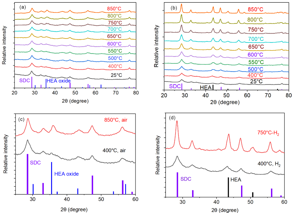
Fig. S3. HT-XRD patterns of HEA nitrate precursors fired in air and 4% H_2/N_2 from 25-850°C with a temperature step of 50-100°C. (a) 400°C pre-fired HEA nitrate precursors fired in air from 25-850°C, (b) 400°C pre-fired HEA catalyst and 4% H_2/N_2 from 25-850°C. (c) 400°C pre-fired HEA nitrate precursors fired in air at 400°C and 850°C (d) 400°C pre-fired HEA catalyst and 4% H_2/N_2 at 400°C and 850°C. * HEA oxides (JCPDS:10-0325, blue dash), SDC (JCPDS: 75-0161, pink dash), HEA, cubic (JCPDS: 47-1417, black dash).
