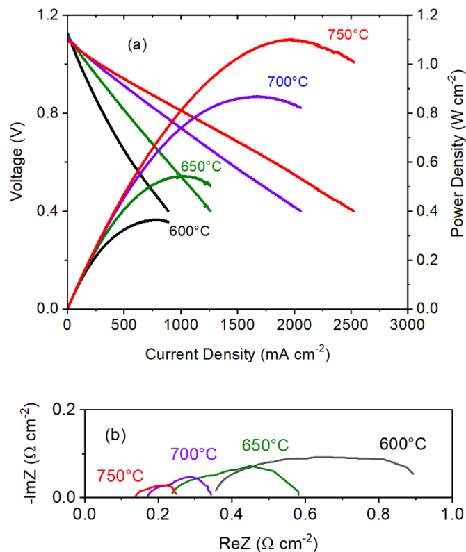
Fig. S7. Cell performance of an optimized HEA-SDS-Ni anode-based MS-SOFC cell tested at a temperature range of 600-750°C in H 2 -air. (a) VI PI curves, (b) EIS of (a). Test conditions: ethanol flow rate: 6 mL min -1 , air flow rate: 1.2 L min -1 .
