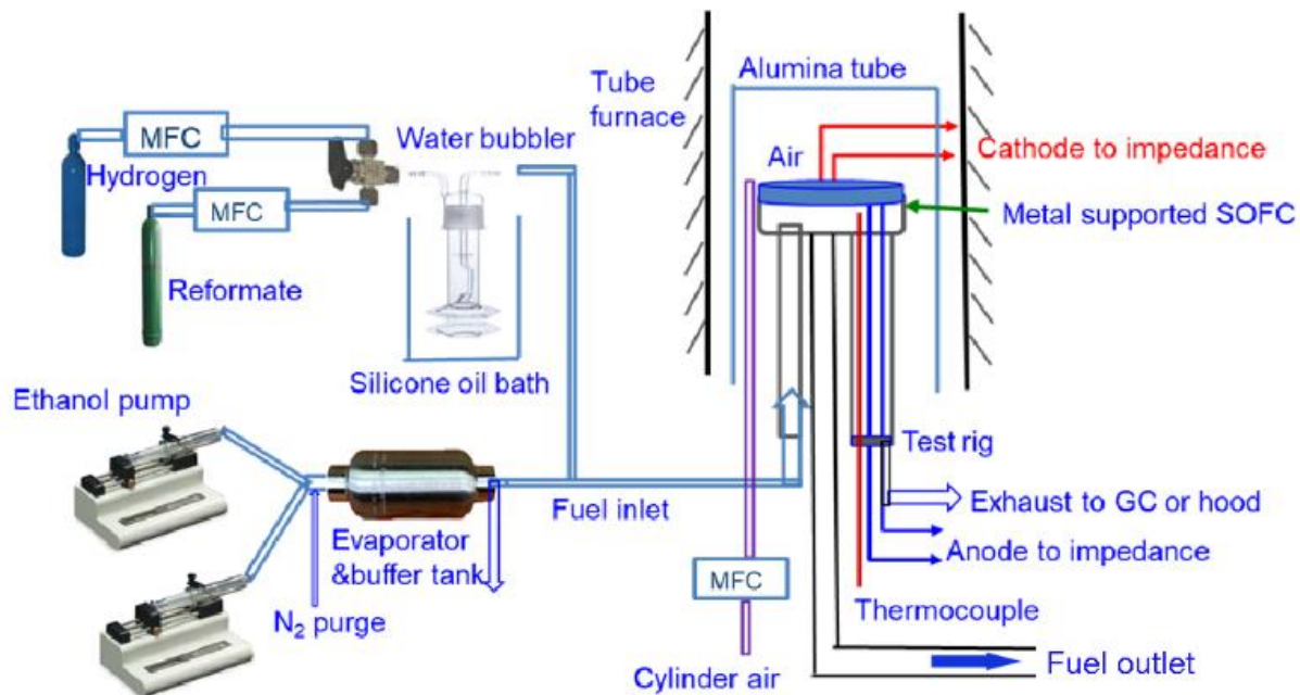
Fig. S2. Scheme of experimental setup and equipment for ethanol-fueled MS-SOFC testing.
