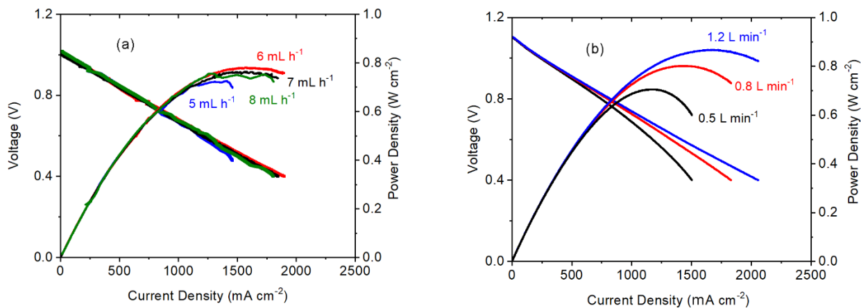
Fig. S6. Optimal ethanol and air flow rates determined by cell testing. (a) VI-PI curves of different ethanol liquid injection flow rates, (b): VI-PI curves of different air flow rates. Test conditions: testing temperature: 700°C, 45% EtOH for (a), and 97% H 2 /3% H 2 O for (b).
