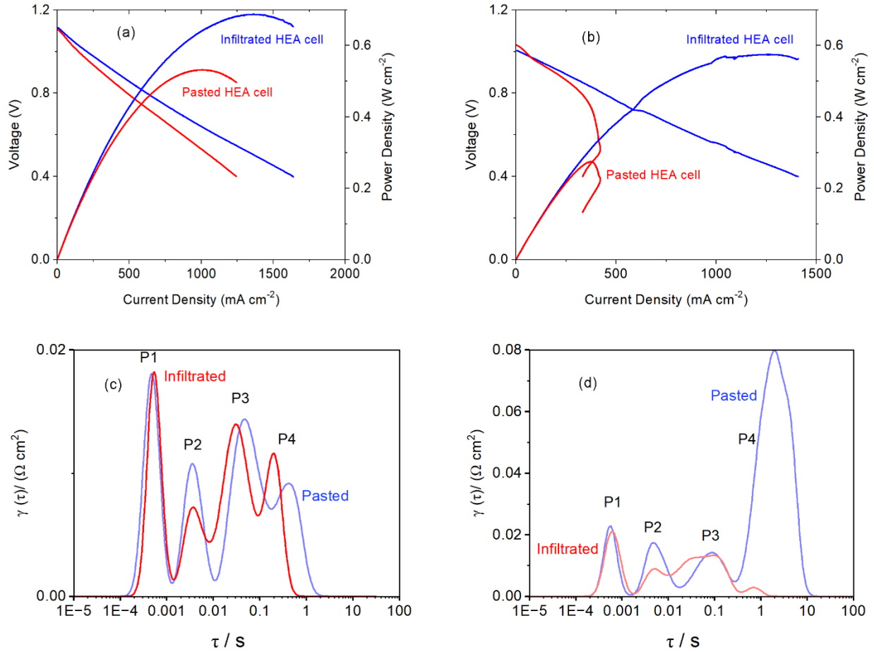
Fig. S1. VI-PI and DRT curves of infiltration HEA-SDC-Ni cell and pasted HEA-SDC-Ni cell tested in 97% hydrogen fuel (a) and 60% EtOH fuel (b) at 700°C. Noticed that the baseline cell with thicker MS was utilized for these tests and led to high mass transport resistance.
