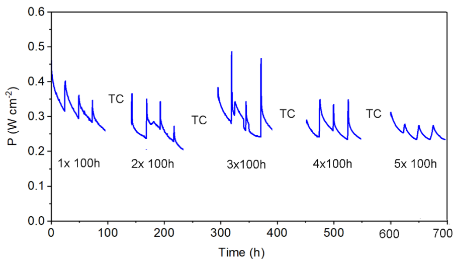
Fig. S9. P-t of the HEA-SDS-Ni anode-based MS-SOFC cell during 500 h operation in 45% ethanol. Note: The upper peaks are due to switching of 45% EtOH to hydrogen fuel when refilling the syringe. Thermal cycling (TC) is from 700-250-700°C, heating ramp rate 25°C/min, naturally cool down.
