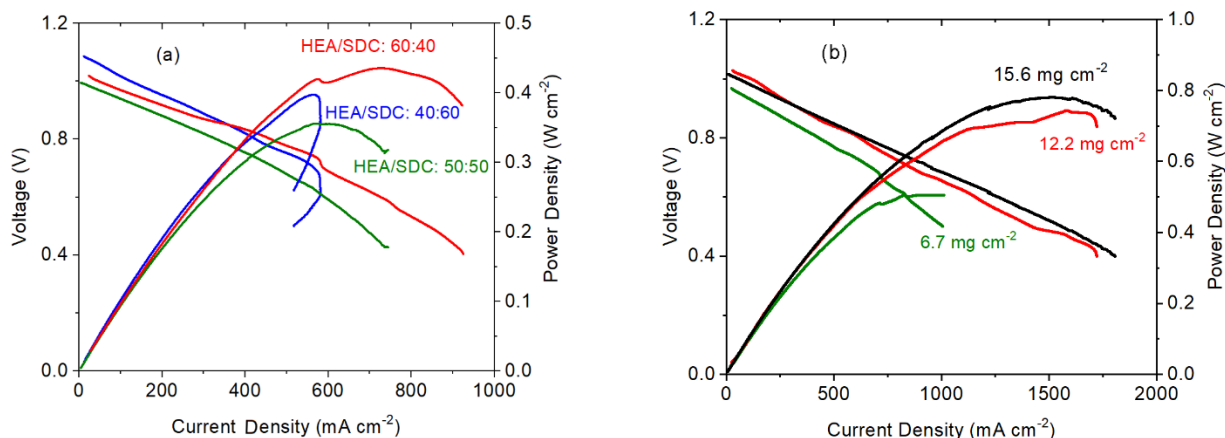
Fig. S5. Optimal HEA/SDC ratio and HEA-SDC catalyst loading for MS-SOFC cells. (a) VI-PI curves of different HEA/SDC ratio (b) VI-PI curves of different catalyst loading. Test conditions: 700°C, 45% EtOH. HEA-SDC catalyst was loaded with 1x, 2x, and 3x infiltration cycles with 6.7, 12.2, and 15.6 mg cm -2 after firing at 850°C for 0.5 h. Note that these cells used standard metal supports, whereas most cells in the main text used improved metal supports (thinner and therefore less total loading of catalyst in the support).
