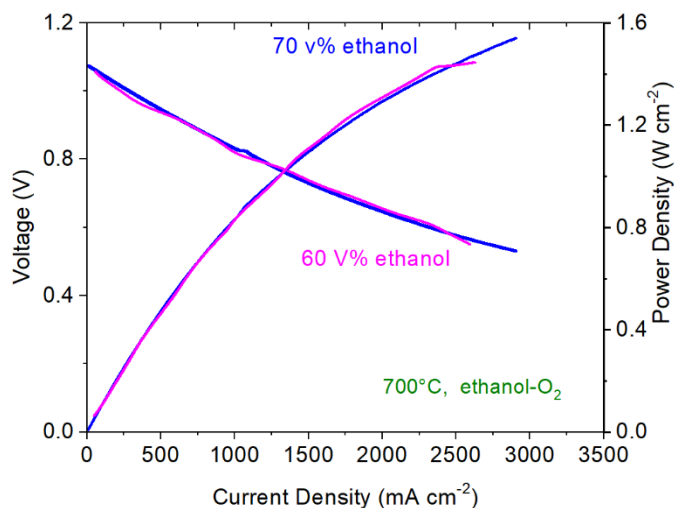
Fig. S8. VI PI curves of optimized HEA-SDS-Ni anode-based MS-SOFC cell in ethanol-O 2 . Test conditions: ethanol flow rate: 6 mL min -1 , air flow rate: 1.2 L min -1 .
