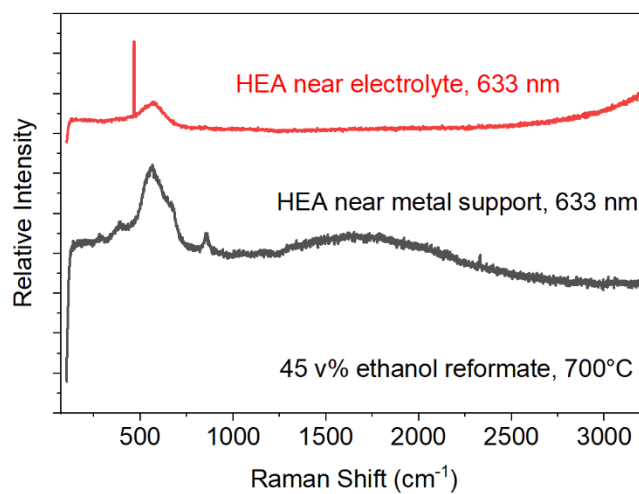
Fig. S12. Raman spectra of posttest HEA-SDC-Ni anode-based MS-SOFC tested in a simulated reformat of 45% ethanol at 700°C for ~350 h. A peak at 383 cm -1 is assigned MnO. A sharp peak at 465 cm -1 is assigned to CeO 2 . A peak at 553 cm -1 is assigned to NiO. A peak at 862 cm -1 is assigned to CrOx. Peaks are not observed for disordered or graphitic carbon.
