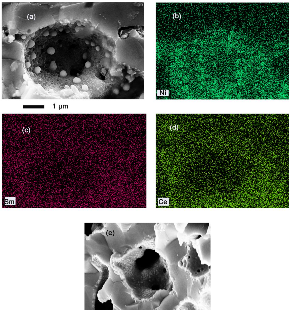
Fig. S13. SEM-EDS maps of 100 h-posttest MS-SOFC showing Ni coarsening at the Ni-SDC anode, test conditions: 700°C, 6 mL h -1 60% EtOH, 1.2 L min -1 air. a: SEM image, b-d: elemental EDS maps of Ni, Sm, and Ce, respectively, e: fresh Ni-SDC catalyst on ScSZ support.
