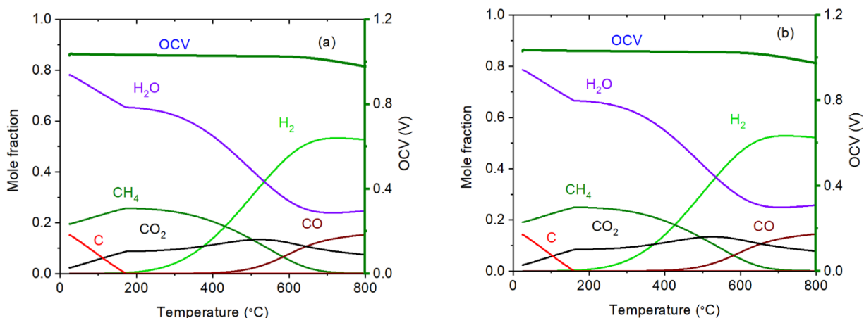
Fig. S14. Gas composition equilibria of steam reforming of ethanol or methanol at different temperatures. (a) 45 v% ethanol/55 v% steam ratio (b) 60 v% methanol/40 v% steam. Note that the results are very similar for these two fuel compositions.
