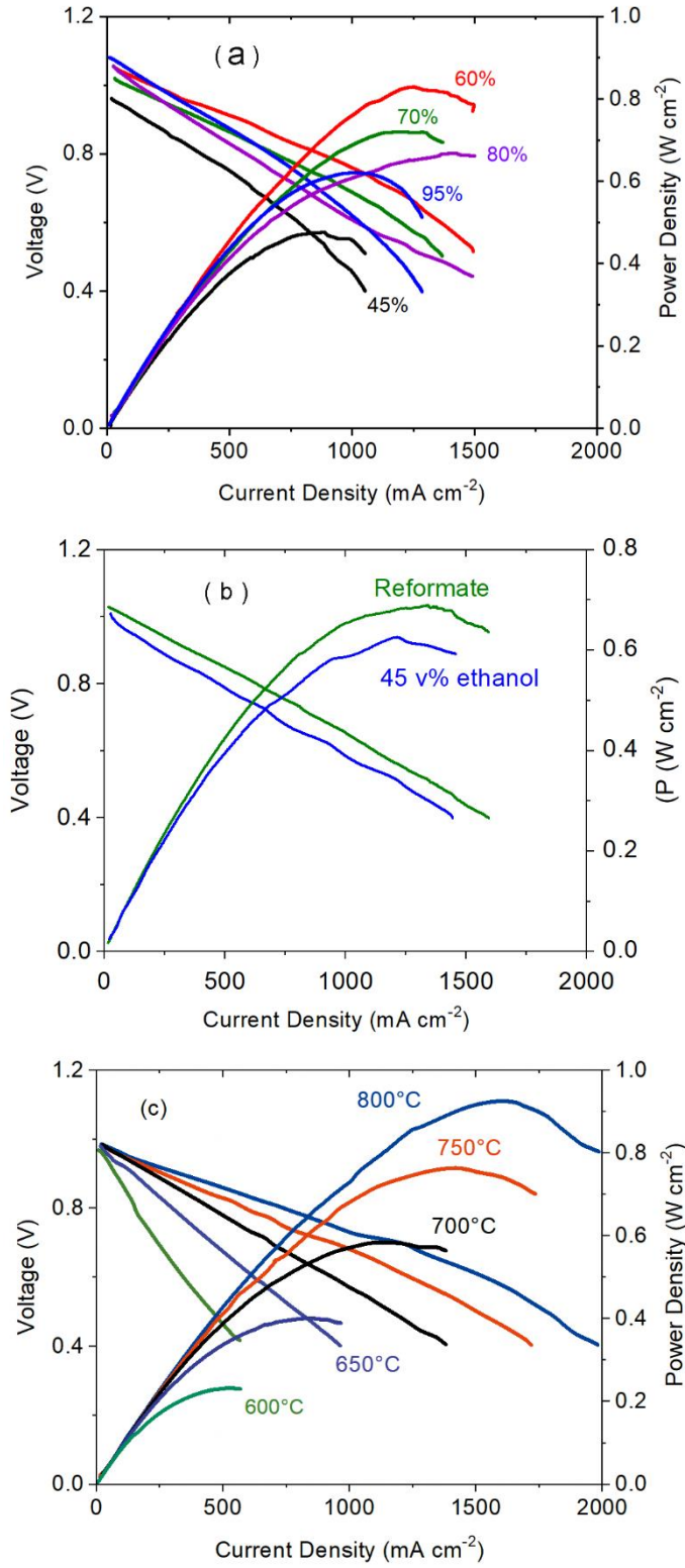
Fig. 4. Evaluation of HEA loading, internal reforming efficiency and cell performance at different ethanol concentrations and operating temperature. a: VI-PI curves at 45 to 95% EtOH
