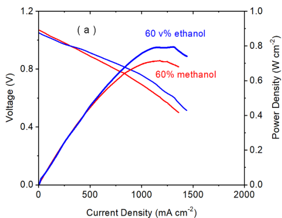
Fig. S10. VI-PI curves of HEA-SDS-Ni anode-based MS-SOFC cell at 700°C. Test conditions: ethanol (methanol) flow rate: 6 mL min -1 , air flow rate: 1.2 L min -1 .
