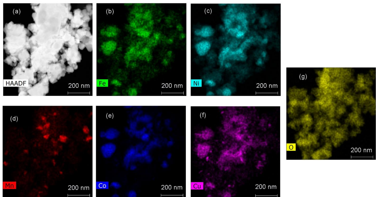
Fig. S4. STEM-EDS maps of HEA elemental distributions on SDC support after sintering at 850°C in air. a: STEM image of HEA catalyst, b-g: elemental EDS maps of Fe, Ni, Mn, Co, Cu, and O, respectively.
