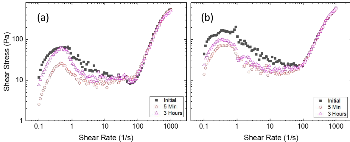
Figure 8: Sequential flow curve tests for: (a) enzyme-treated and (b) untreated (control) slurries with initial solids concentrations of 15% (w/v) measured using the starch pasting impeller.
