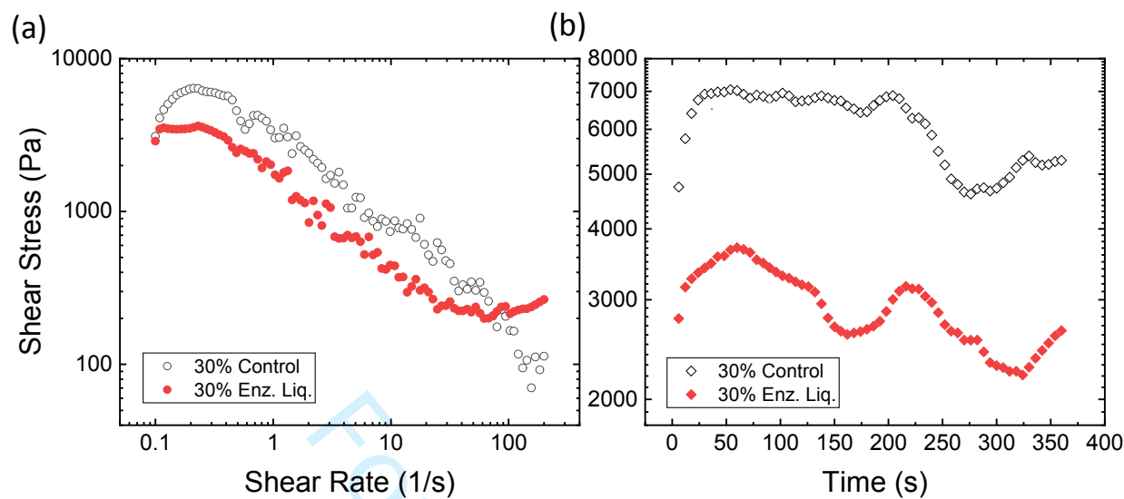
Figure 6: Representative relative shear stress response of high concentration slurries (30% w/v initial solids) from: (a) an increasing shear rate ramp (flow curve) and (b) a constant shear rate test ( 0.1\text{ s}^{-1} ), both performed in a wide-gap rheometer setup with a starch pasting impeller.
