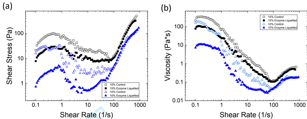
Figure 4: Representative relative (a) shear stress and (b) viscosity responses for low concentration slurries (10 and 15% w/v initial solids) sheared in a wide-gap rheometer setup with a starch pasting impeller.
