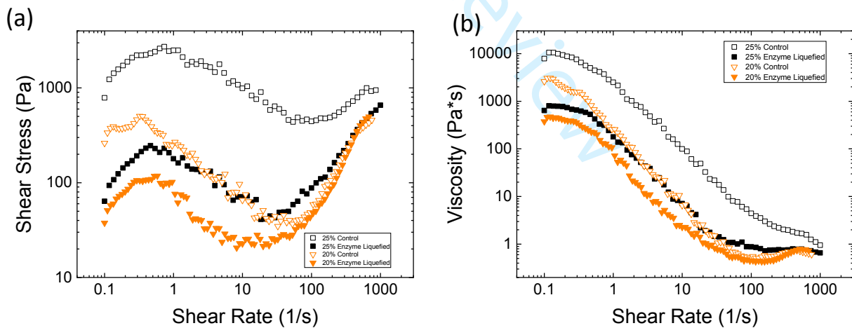
Figure 5: Representative relative (a) shear stress and (b) viscosity responses for moderate concentration slurries (20 and 25% w/v initial solids) sheared in a wide-gap rheometer setup with a starch pasting impeller.
