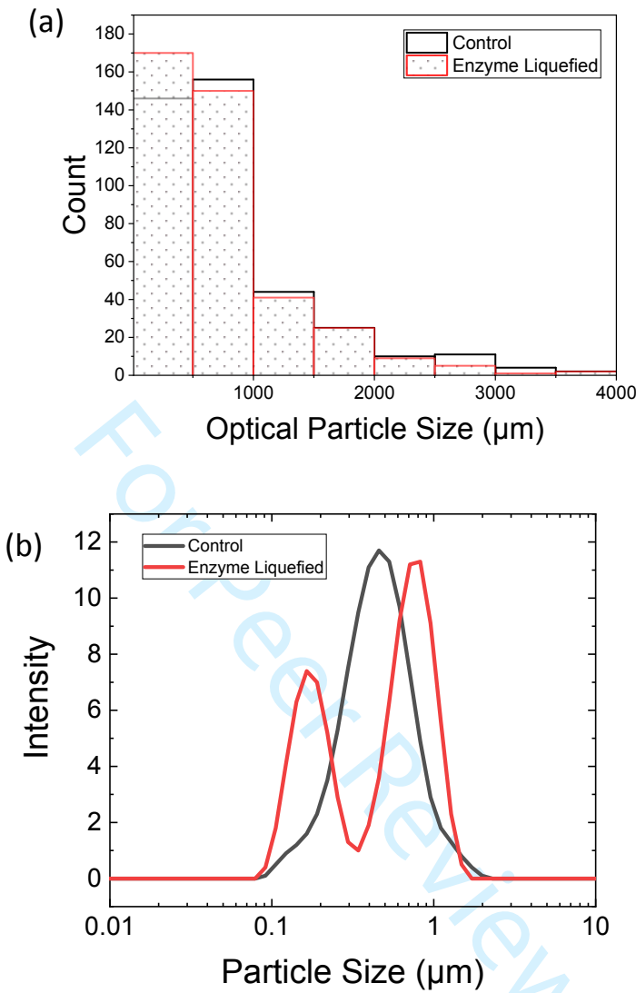
Figure 3: Particle size measurements performed on diluted samples of untreated (control) and enzyme-treated corn stover slurries with an initial solids concentration of 30% (w/v) from both (a) optical microscopy and (b) dynamic light scattering.
