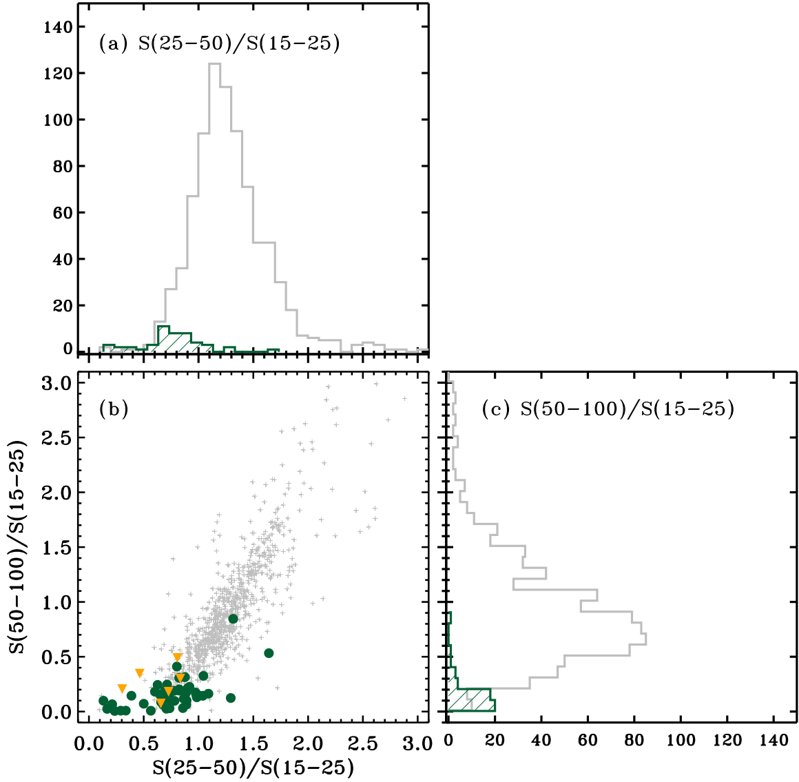
Fig. 3. Energetics. Comparison of energetics of SFXT ( N = 48 , dark green) and GRB ( N = 833 , grey): (a) distributions of the S_{21} = S(25 - 50)/S(15 - 25) colours; (b) colour-colour diagram drawn from the 15–25 keV, 25–50 keV, and 50–100 keV energy bands, with the orange triangles ( N = 6 ) representing 3\sigma upper limits for S(50 - 100) ; (c) distributions of the S_{31} = S(50 - 100)/S(15 - 25) colours.
