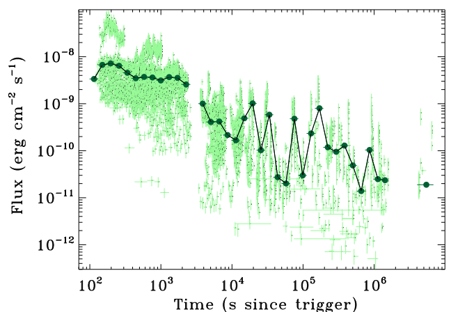
Fig. 9. XRT unabsorbed flux light curves (erg cm -2 s -1 ) in the 0.3–10 keV energy band as a function of time (s since the BAT trigger). The dark green points mark the medians.
