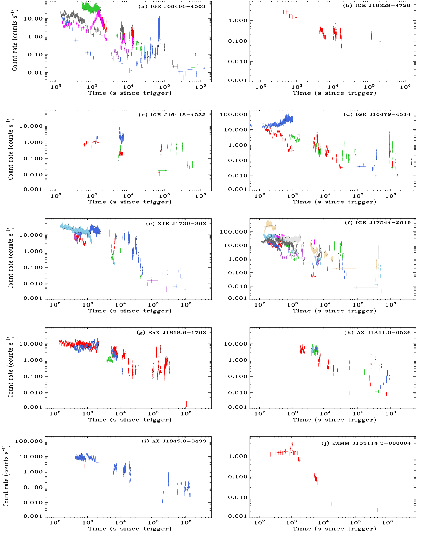
Fig. 7. XRT light curves counts \text{s}^{-1} in the 0.3–10 keV energy band grouped by source [(a) IGR J08408–4503, (b) IGR J16328–4726, (c) IGR J16418–4532, (d) IGR J16479–4514, (e) XTE J1739–302, (f) IGR J17544–2619, (g) SAX J1818.6–1703, (h) AX J1841.0–0536, (i) AX J1845.0–0433, (j) 2XMM J185114.3–000004] as a function of time (s) since the BAT trigger, where different colours correspond to different events. The complete list of triggers for each source can be found in Table 2.
