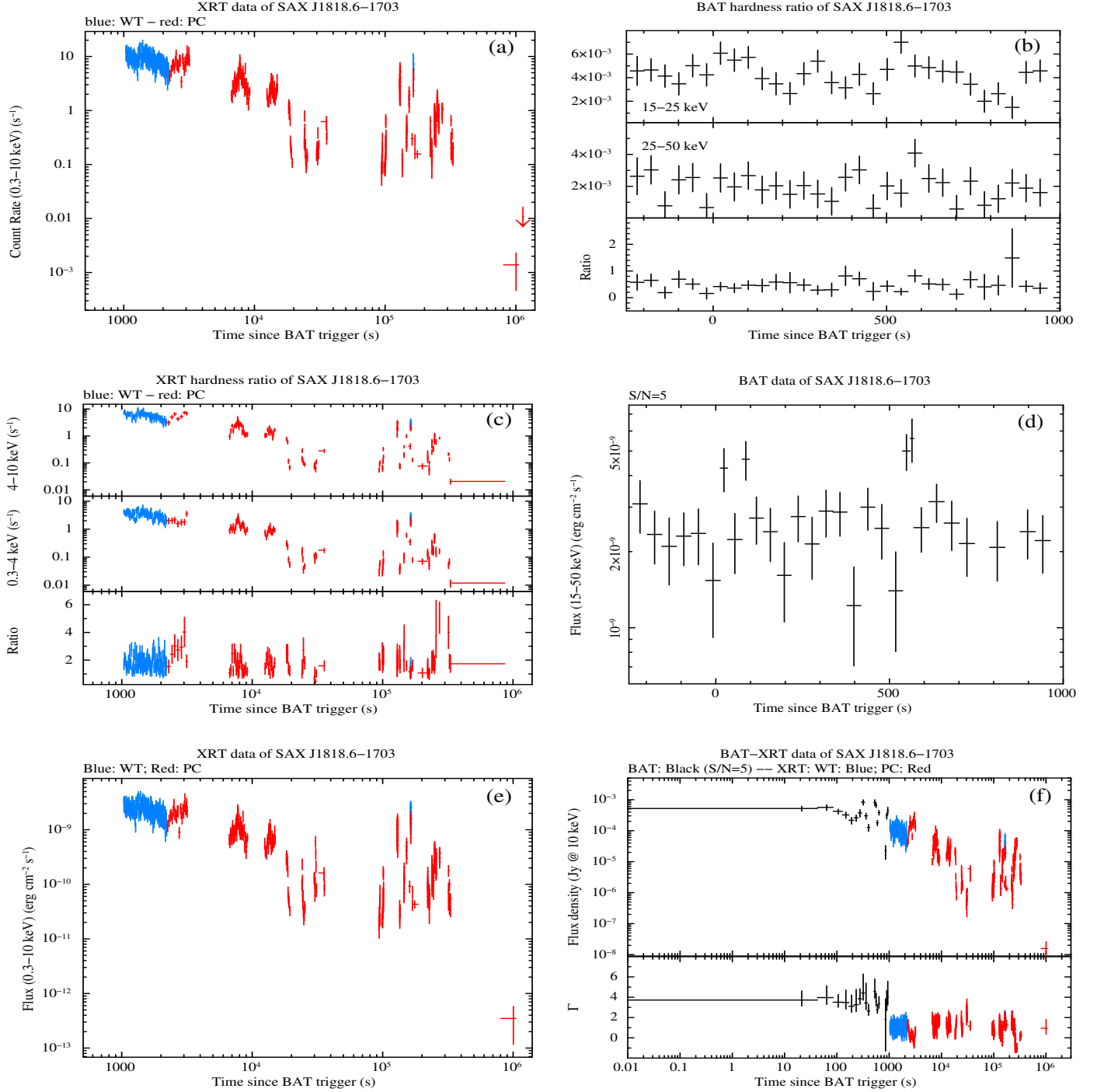
Fig. 1. Example of Burst Analyser products for the third recorded outburst from SAX J1818.6–1703 (see Table 2). (a): XRT 0.3–10 keV count-rate light curve; (b): BAT 15–25 keV, 25–50 keV, and (25–50 keV/15–25 keV) hardness ratio; (c): XRT 4–10 keV, 0.3–4 keV and (4–10 keV/0.3–4 keV) hardness ratio; (d): BAT 15–50 keV spectral evolution dependent flux light curve; (e): XRT 0.3–10 keV spectral evolution dependent, unabsorbed flux light curve; (f): evolution dependent flux density light curves at 10 keV.
