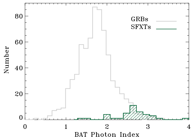
Fig. 6. Distribution of photon indices for SFXT triggers (hashed green histogram) and GRBs (light grey histogram) when BAT spectra are fit with a simple power-law model.
