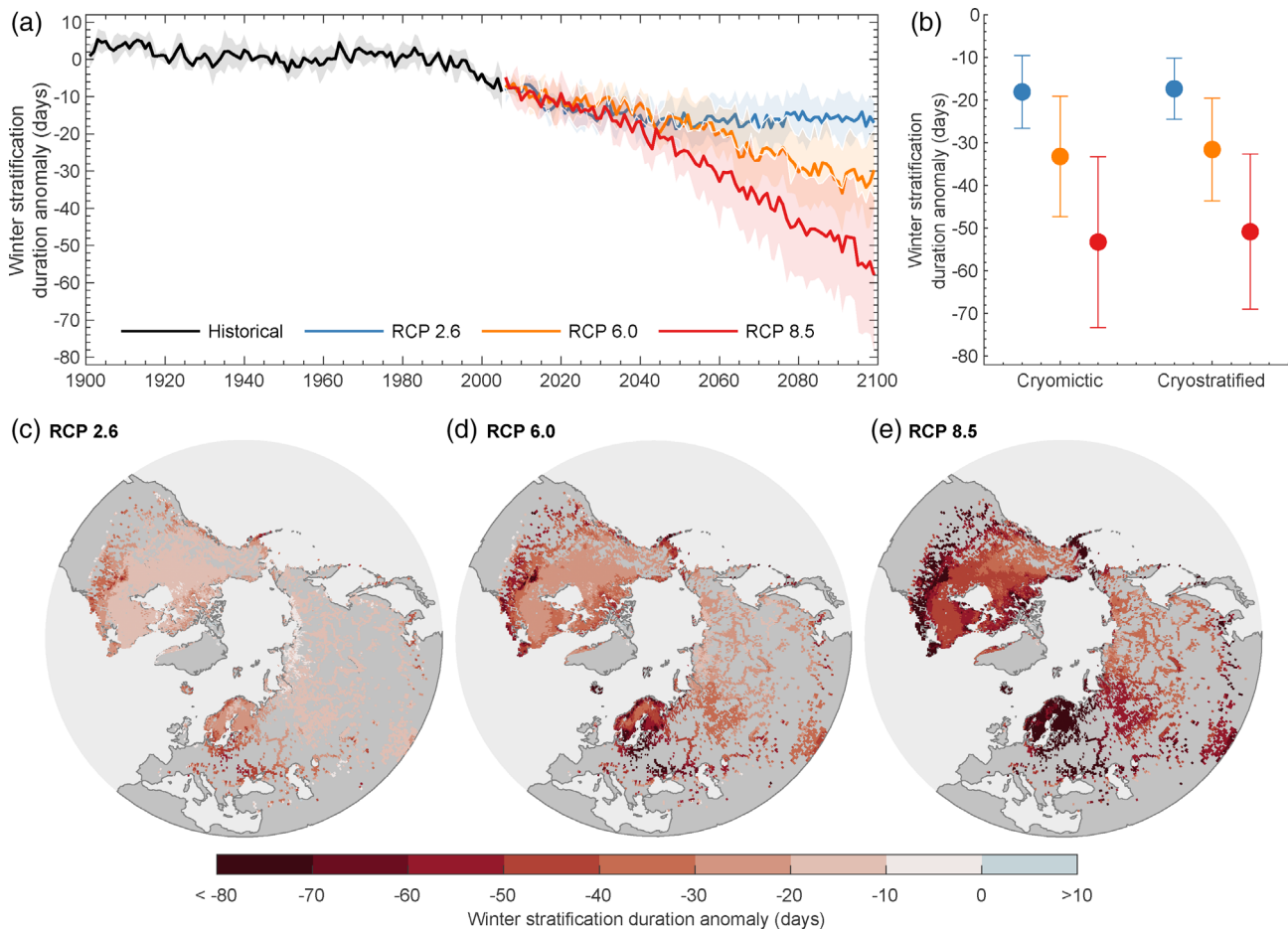
Fig. 3. Historic and future projections of winter lake stratification duration. Temporal and spatial variations in the duration of winter stratification. The temporal changes in winter stratification are shown (a) from 1901 to 2099 under historic (1901–2005) and future (2006–2099) climate change scenarios (RCP 2.6, 6.0, 8.5). The thick lines show the average across all lake-climate models, and the shaded regions represent the standard deviation across the ensemble. Panel (b) shows the average change (and standard deviation) in winter stratification duration by 2070–2099, separated by lake mixing regimes (i.e., cryomictic and cryostratified). Panels (c–e) show the spatial patterns in winter stratification duration anomalies by the end of the 21 st century (2070–2099) under (c) RCP 2.6, (d) RCP 6.0, and (e) RCP 8.5. Anomalies are quoted relative to the 1970–1999 average. All results are based on the average simulations across the model ensemble.
