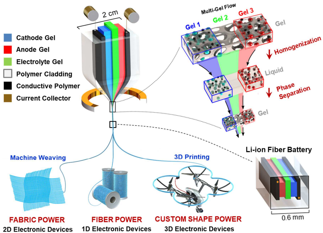
Figure 1. Thermal fiber battery drawing including multiple gels and its expansion into 2D and 3D flexible multidimensional electronics. The thermally drawn fiber battery consists of lithium-iron-phosphate (LFP) gel for the cathode, lithium titanate (LTO) gel for the anode, electrolyte gel, cyclic olefin copolymer (COC) cladding, and metal wires embedded in carbon-loaded polyethylene (CPE). The PVDF and EC:PC solvent mixture in LFP, LTO, and electrolyte gels are homogenized at the elevated temperature (in the furnace) and then phase-separated at room temperature (outside the furnace) forming interconnected pore structures with minimal gaps between cathode, anode, and electrolyte. The fiber battery can be integrated with electronic components to form 1D, 2D, and 3D electronic devices.
