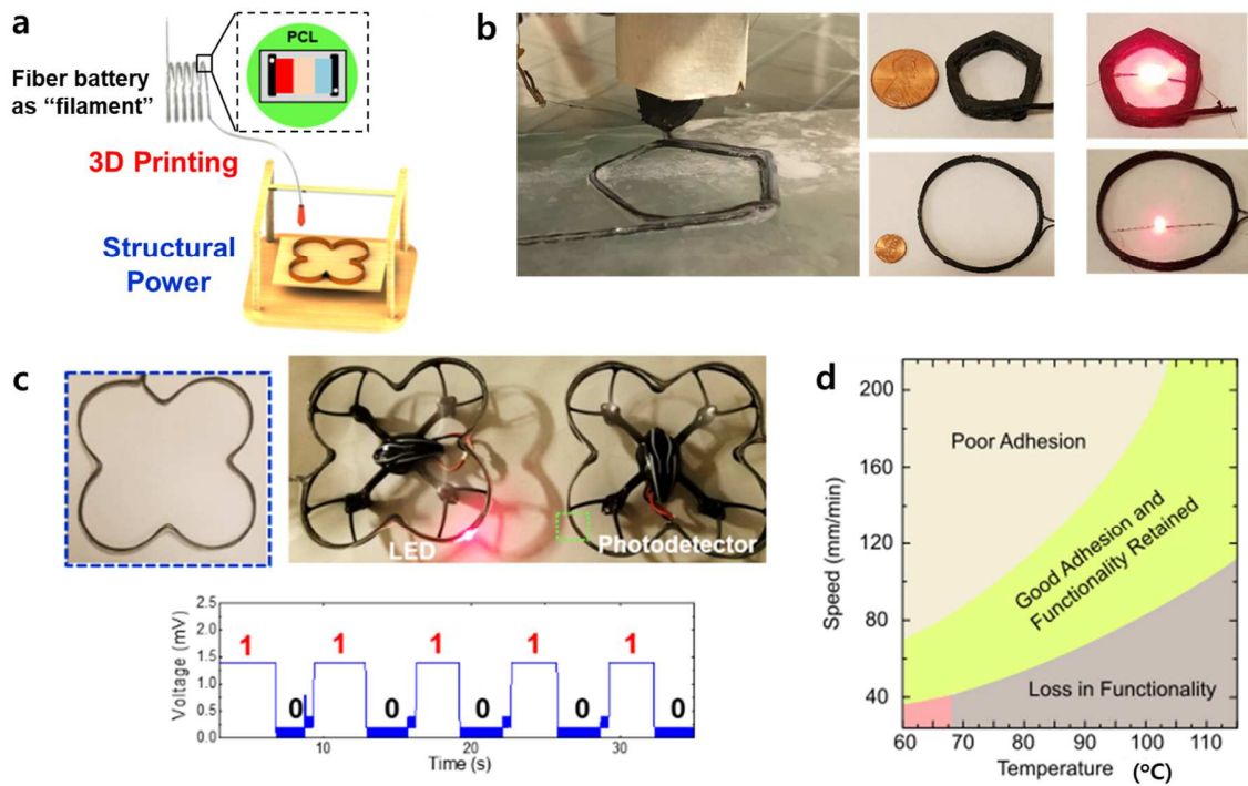
Figure 5. Thermally drawn fiber battery in 3D electronics; a) Schematic diagram of 3D printing process by using a thermally drawn Li-ion battery fiber. Fiber battery with PCL cladding enables a new fiber battery direction towards 3D structural power. b) multiple 3D-printed batteries in different shapes and size, c) 3D-printed drone casings from the fiber battery. The 3D-printed drone casing powers the fiber LED, and photodetector system for drone-to-drone communication. d) 3D product quality with respect to the 3D printing speed and temperature.
