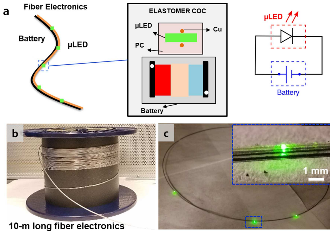
Figure 3. Thermally drawn fiber battery in 1D electronics; Integrated fiber battery through co-drawing of LED and battery modalities; a) schematic diagram of integrated LED/battery fiber and its corresponding electrical circuit, b) the 10-meter-long LED/battery fiber, c) green LEDs powered by fiber battery within the same fiber.
