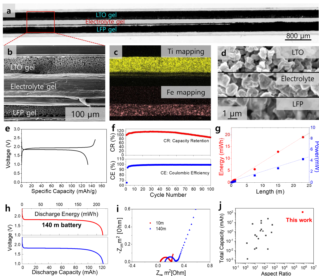
Figure 2. Morphology and electrochemical characterization of the fiber battery; a) Optical micrograph of the side view showing clear segregations between anode and cathode, b) SEM micrograph of dried fiber battery, c) EDS Fe mapping and Ti mapping, d) dried LFP, LTO, and electrolyte gels in fiber. SEM and EDS images are acquired after dissolving cladding material in cyclohexane under ambient conditions, e) representative galvanostatic charge-discharge profile at \sim C/5 , f) capacity retention and coulombic efficiency versus cycle number at \sim 5C , g) energy and power versus length of fibers. The cross-section area of active material is approximately 120(t) \times 180(w) \mu\text{m}^2 , h) discharge profiles of 140 m thermally drawn battery fiber. i) Nyquist plots of 10 m and 140 m battery fibers, and j) total capacity vs aspect ratio of thermally drawn Li-ion battery fibers compared with previously reported fiber cells. For a cylindrical shape fiber, the diameter was used while for the ribbon shaped fiber, the averaged value of width and thickness ( (\text{width} + \text{thickness})/2 ) was adopted to calculate the aspect ratio.
