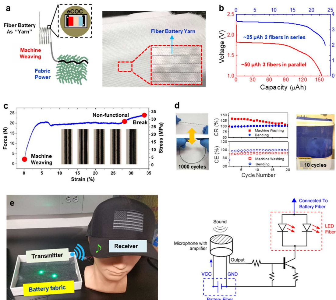
Figure 4. Thermally drawn fiber battery in 2D electronics; a) A battery fiber embedded within 135 \times 120 \text{ cm}^2 textile. The 1.27 \text{ cm} space between black fiber batteries is filled by white polypropylene coated glass fibers. The fiber battery powers flexible fiber-based fabric electronics. b) Fiber battery in parallel and series configurations. Discharge profiles of three \sim 50 \mu\text{Ah} fiber batteries in parallel and two \sim 25 \mu\text{Ah} fiber batteries in series. c) Force/Stress-Strain curve of a thermally drawn Li-ion fiber battery and side-view images of fiber battery corresponding to the strains of 10, 15, 20, 25, and 30%. d) Capacity retentions after 1000 bending cycles and 10 washing cycles. e) A 100 m long fiber battery-powered LiFi fabric sample as a next-generation communication fabric and its corresponding electric circuit. Fiber battery powers a microphone with a pre-amplifier, a transistor, and diode fibers.
