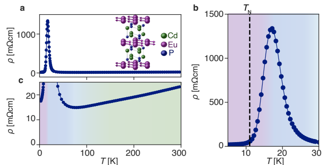
Figure 1. (a,b) The resistivity of \text{EuCd}_2\text{P}_2 (structure in the inset) shows a pronounced peak at 18 K. (c) Above 75 K it exhibits metallic behavior. Data are from ref. [5].
