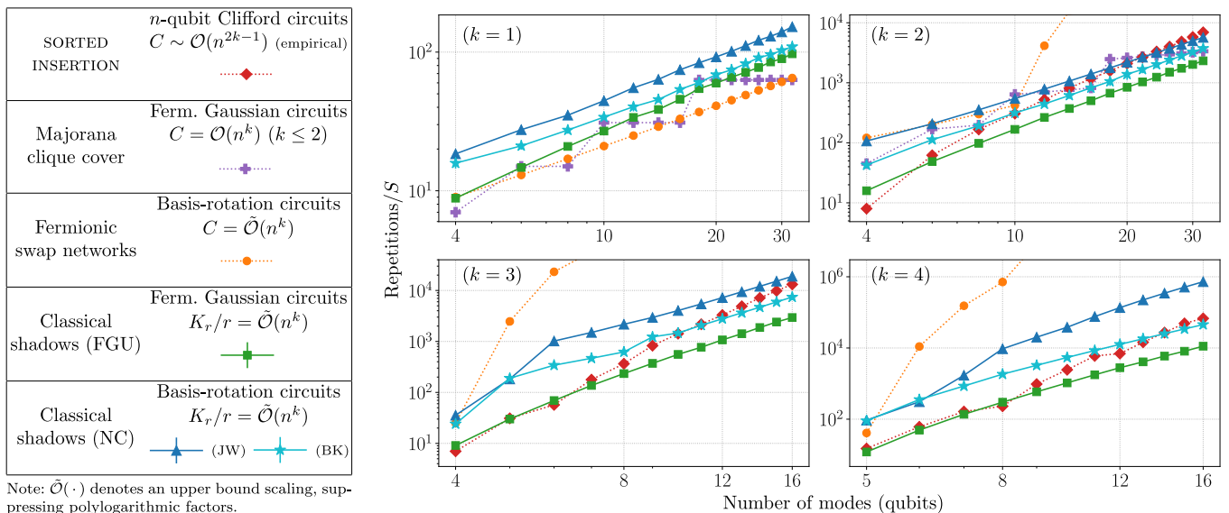
FIG. 1. (Left): Summary of the methods compared here, cataloging their required circuit types and scalings in the number of measurement settings. Since graph-based methods [33–35, 38] are resource-intensive, we employ SORTED INSERTION [17] as a more tractable alternative. The Majorana clique cover [37], which employs the same class of fermionic Gaussian Clifford circuits as our classical shadows (FGU) unitaries, possesses optimal asymptotic scaling; however, it exhibits jumps at powers of 2 due to a divide-and-conquer approach. Furthermore, the construction only exists for k \leq 2 . The measurement strategy using fermionic swap networks is a generalization of the optimal 1-RDM strategy introduced in Ref. [61], which we describe in Sec. IV of the SM [83]. (Right): Numerical performances (log-log scale). Note that SORTED INSERTION and the Majorana clique cover are equivalent for k = 1 . Since our scheme uses randomization, we include error bars of 1 standard deviation, averaged over 10 instances. However, they are not visible at the scale of the plots, indicating the consistency of our method.
