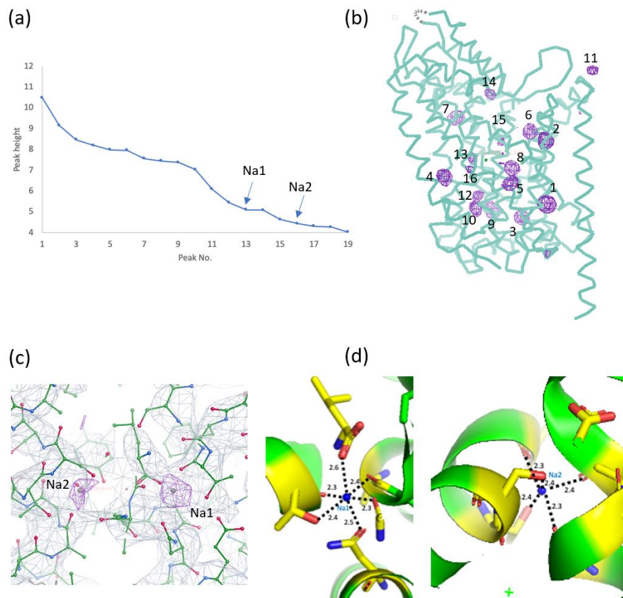
Figure 3. Characterization of Na + in LeuT. (a) A plot of the 19 highest Bijvoet-difference Fourier peaks in LeuT. Two Na + peaks are indicated by arrows. Sulfur peaks for methionine residues are 1, M363; 2, M403; 3, M65; 4, M199; 5, M360; 6, M394; 7, M44; 8, M176; 9, M452; 10, M18; 12, M59. (b) Bijvoet-difference Fourier peaks are shown as purple isomeshes contoured at 3.5 \sigma . The refined LeuT model is shown as sticks. Peaks 13 and 16 are for Na1 and Na2, respectively. (c) Electron densities (magenta isomeshes contoured at 4 \sigma ) for two Na + in LeuT. 2Fo-Fc electron densities are shown as gray isomeshes contoured at 1.5 \sigma . (d) Na + -binding sites in LeuT. Residues and leucine forming the Na + -binding sites are shown as sticks. Distances (Å) between Na + and the bound atoms are shown as dash lines.
