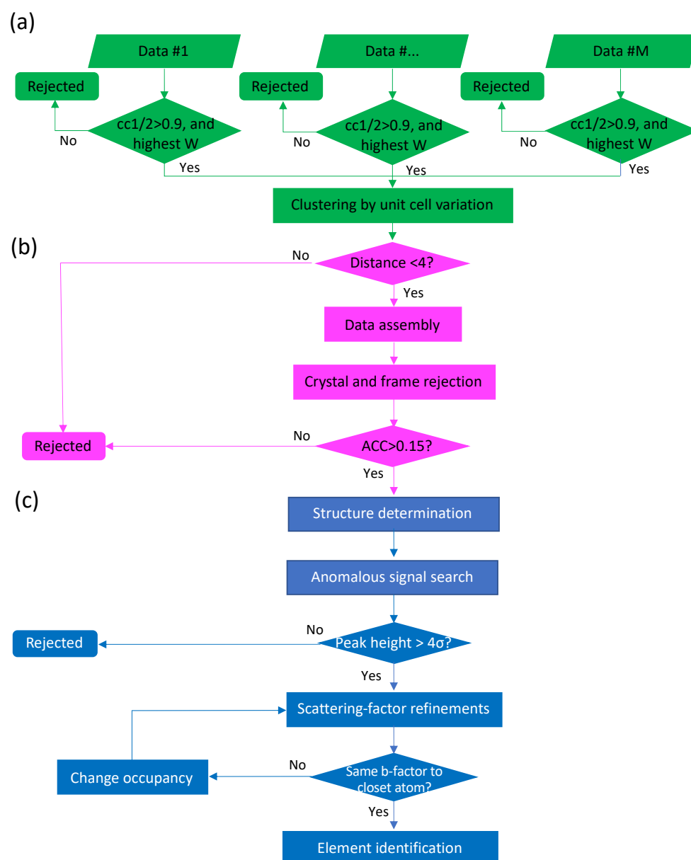
Figure 1. Schematic workflow for \text{Na}^+ identification. (a) Single-crystal data set processing. Single-crystal data sets were independently indexed, integrated, and scaled using PyMDA as 10 progressively accumulated wedges (W) (W1, 1-60; W2, 1-120; ..., W10, 1-600 frames). The largest wedges which have CC1/2 > 0.9 were selected for further data analysis. (b) Data assembly and rejection. Data sets classified with a unit-cell variation of less than 4 were combined. Unit-cell variation is defined as Euclidean distances normalized by population variances as reported previously [26]. Assembled data sets were subjected to crystal rejection followed by frame rejection by PyMDA. Only data sets that showed significant anomalous signals ( ACC > 0.15 ) were advanced to the next step. (c) LeuT structure was determined by molecular replacement using PDB code 3GJD as a search model. Anomalous signals were searched by ANODE. Significant anomalous signals ( > 4\sigma ) at the \text{Na}^+ binding site were subjected to f'' refinement by PHENIX.REFINE. The occupancy of anomalous scatterers was changed from 1.0 to 0.1 in 0.1 intervals and refined individual B-factor and f'' values. The refined
