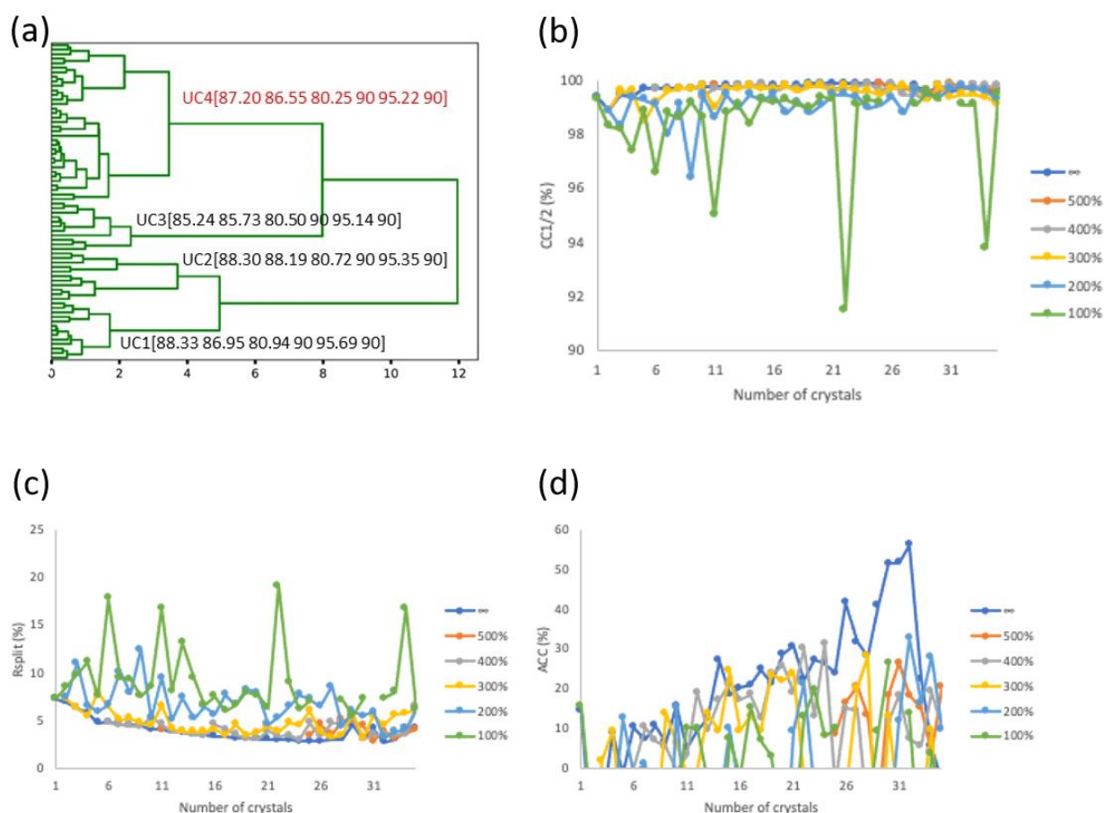
Figure 2. Data analysis of assembled LeuT data sets. (a) Unit-cell variation analysis for classification of single-crystal data sets. Unit-cell parameters of each cluster are shown. (b)–(d) Data assembly and subsequent crystal and frame rejections were performed by using PyMDA as described in the methods: \infty , no frame rejection and 500–100%, where 100% is the most stringent rejection. (b) CC1/2 at 4 Å d_{\min} . (c) Rsplit at 4 Å d_{\min} . (d) Anomalous correlation coefficient (ACC) at 10 Å d_{\min} .
