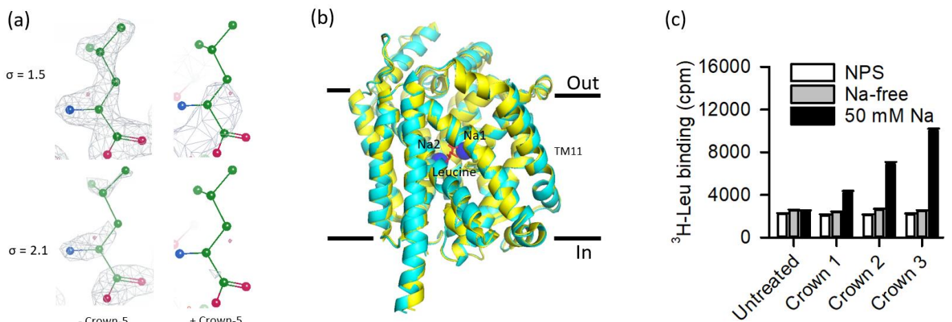
Figure 4. \text{Na}^+ and leucine depletion in LeuT. (a) 2Fo-Fc electron density maps of bound substrate leucine with and without Crown-5 soaking. (b) Comparison of LeuT structure with (yellow) and without (cyan) Crown-5 soaking (PDB code: 3GJD). Two \text{Na}^+ and the substrate leucine in the non-soaking structure (PDB code 3GJD) are shown as blue spheres and red sticks, respectively. (c) Removal of \text{Na}^+ from LeuT-containing E. coli C41(DE3) membrane vesicles by repeated treatments with Crown-5 as described in the Methods. The activity of 50 ng of purified LeuT from differently treated vesicles was then assessed by measuring the binding of 50 nM ^3\text{H} -Leu (120 Ci/mmol) in the presence of 50 mM NaCl (50 mM Na; black bars) or the absence of NaCl (Na-free; gray bars) in the assay buffer using the scintillation proximity assay (SPA). The non-proximity signal (NPS) was determined for each condition. \text{Na}^+ and Leu from the cell culture medium are trapped in LeuT and prevent significant binding of ^3\text{H} -Leu to the untreated sample. Repeated treatments with Crown-5 during the vesicle preparation led to the removal of the trapped compounds. Data are the mean \pm S.E.M of three independent repeats that were performed as technical triplicates.
